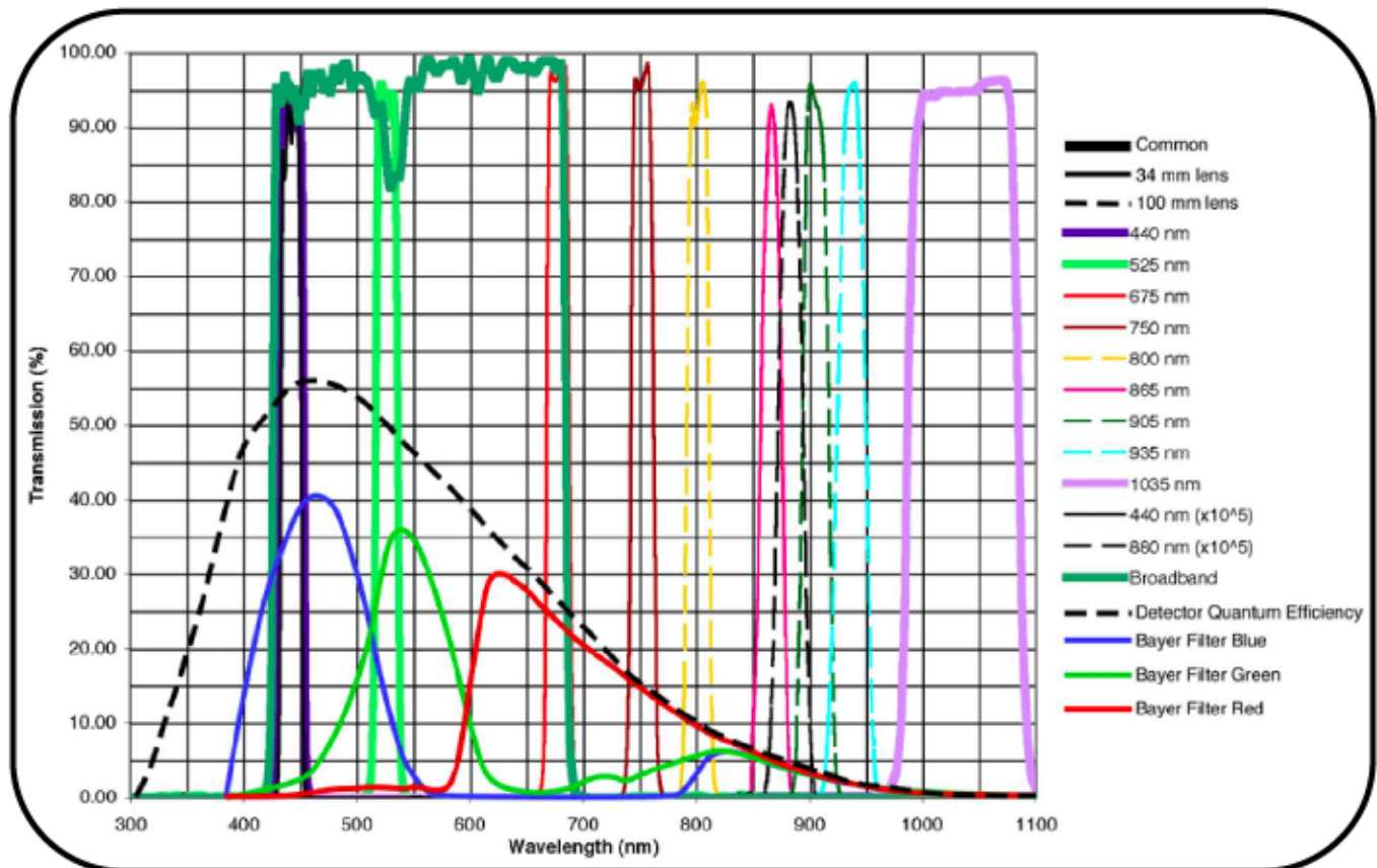
Figure 2.3.1.2.2 - Mastcam Filter Profiles, Filter Wheel Set to Nonzero
