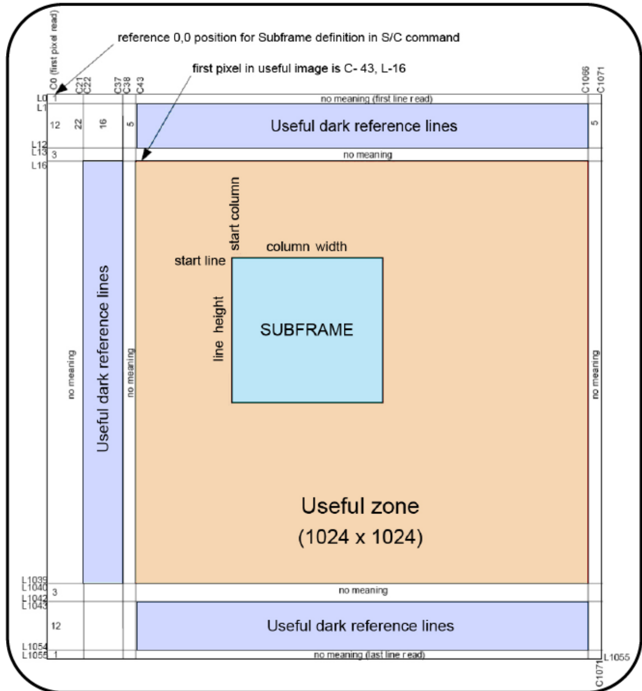
Figure 2.2.1.1 - Acquisition and Readout of RMI Camera Image Data
