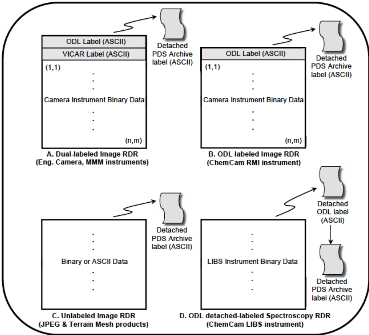
Figure 5.4 - RDR Product Structures
