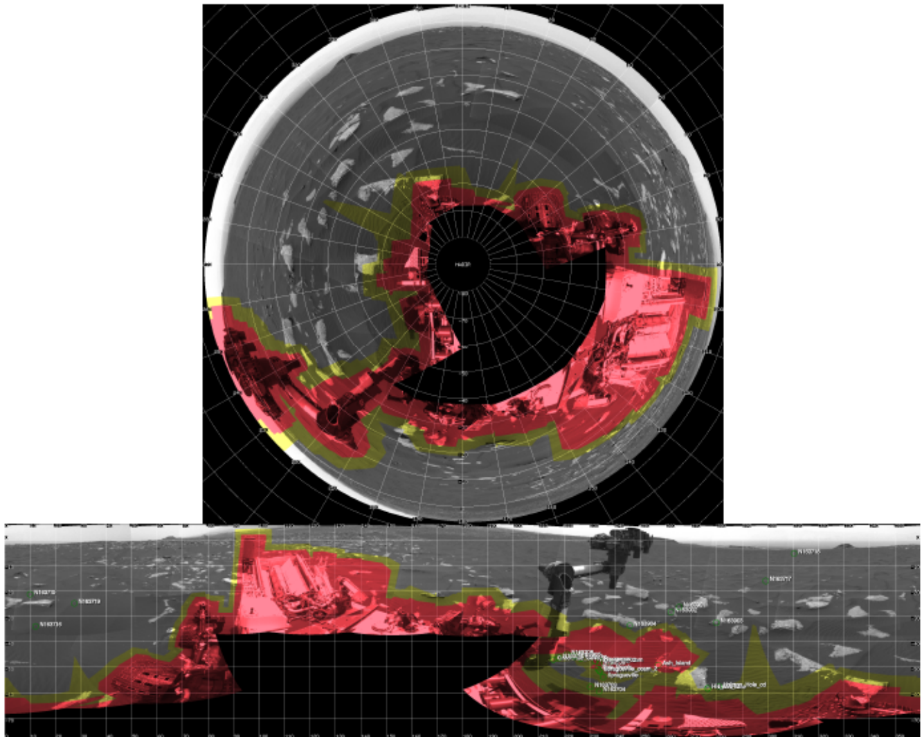
Figure 5.2.1.13.11 – ChemCam Finder “MCF” masks for 2 different arm configurations, applied to the same Navcam mosaic basemap in polar (top) and cylindrical (bottom) projections.
