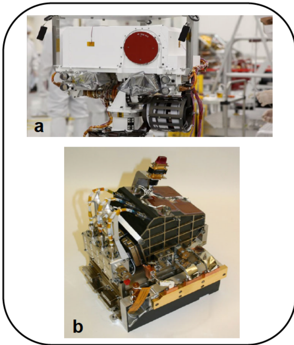
Figure 2.2.1 – Mast Unit (a) in white housing with red telescope cover, and Body Unit (b)
