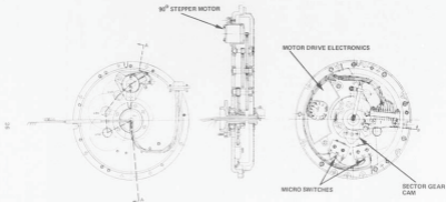
Fig. 6-4 Gear-box assembly, Y axis.
