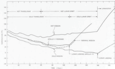
Fig. 7-1. Quad III storage pallet temperatures.
