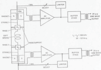
Fig. 4-1 Schematic diagram VSA and support electronics.
