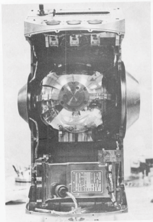
Fig. 10-3 Gravimeter interior detail.
