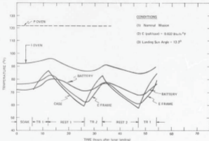
Fig. D-2 Normal-mission thermal response.
