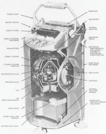
Fig. 6-2 Cutaway view of traverse gravimeter.
