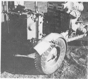
Fig. 8-2 Gravimeter ready for EVA 2.
