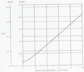
Fig. F-1 Error due to leveling system bias (assuming \pm 3 arc minute pendulum deadband).
