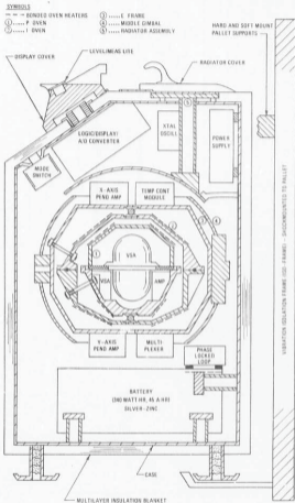
Fig. 7-2 TG thermal design cutaway.
