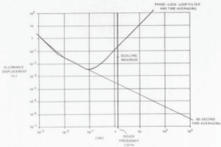
Fig. G-3 Displacement sensitivity.
