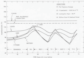
Fig. D-1 Hot-mission thermal response.
