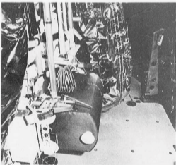
Fig. 11-1 Gravimeter installed before launch.
