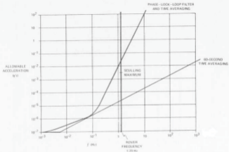
Fig. 6-1. Vibration sensitivity.
