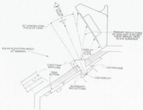
Fig. 8-1 LED numeric display technique.
