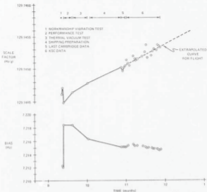
Fig. 10-1 Scale factor and bias vs. time for prime flight gravimeter.
