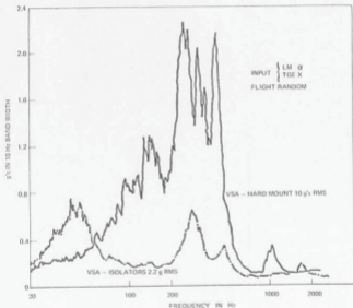
Fig. 6-3 Effect of rubber isolators.
