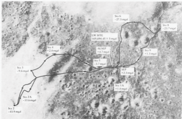
Fig. 11-2 Traverse gravity values from Apollo 17.
