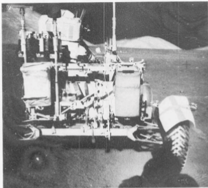
Fig. 11-4 Traverse gravimeter mounted on geology pallet.
