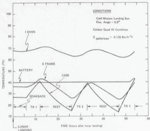
Fig. D-3 Cold-mission thermal response.
