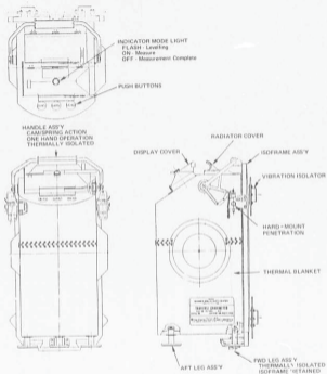
Fig. 6-1 Outline drawing of traverse gravimeter.
