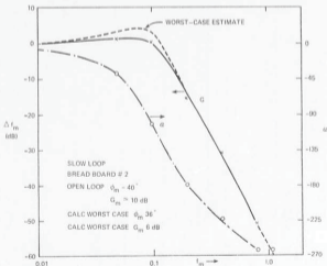
Fig. G-2 Phase-locked loop - Bode plot.
