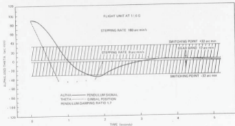
Fig. 3-1. Response to a 1.5-degree step.
