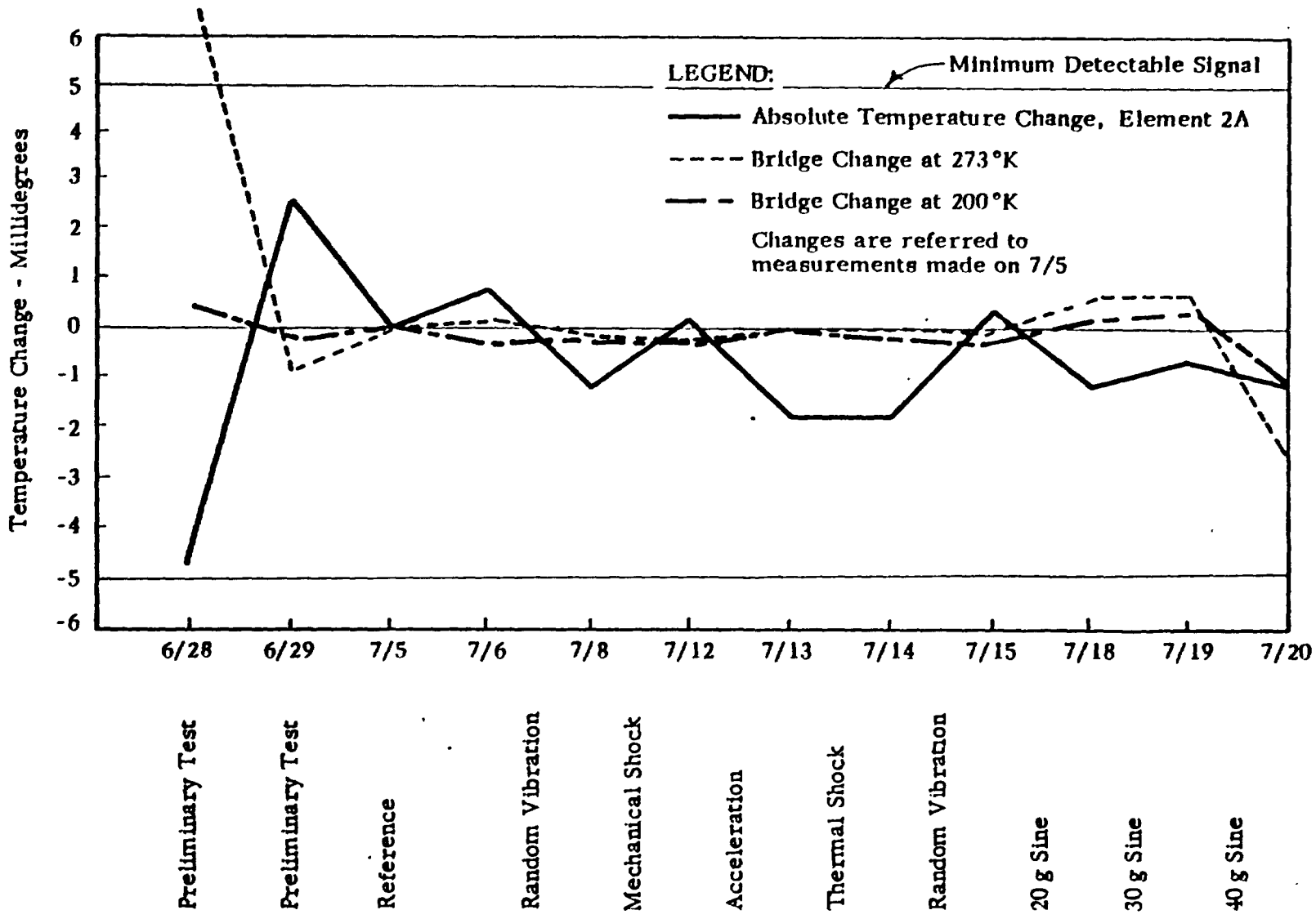
PLATINUM SENSORS 2A, 2B, 3A, & 3B PERFORMANCE--ROSEMOUNT DATA
