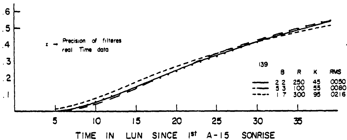
Fits to the astronaut induced transient component at representative A-15 sensors
