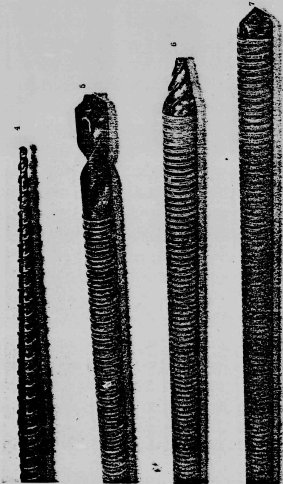
Appendix B-Figure 5. Hole Casing Tip Configurations
