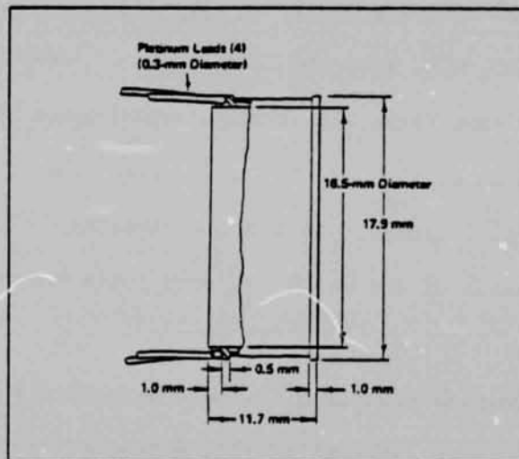
Figure 3 Ring- or Remote-Sensor Construction
