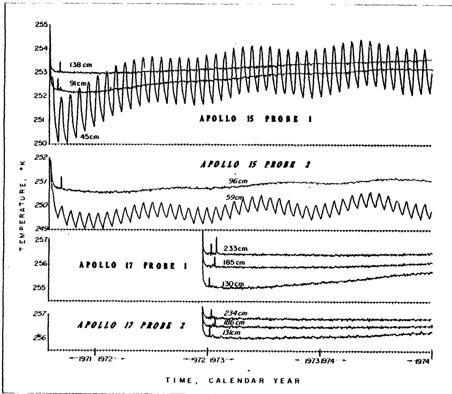
Subsurface temperature histories covering a 3.5 yr period of representative sensors on the four heat-flow probes. Initial cooldown of the probes after insertion can be seen at the start of each history. The small spikes in the first 60 days result from the short-term conductivity experiments.
