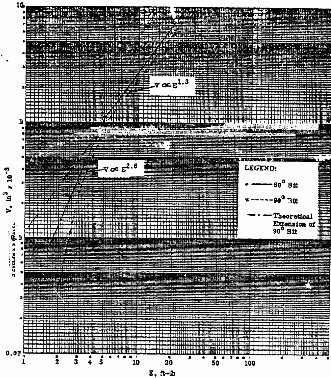
Volume-Energy Relation for 60° and 90° Wedge Bits in Drop Tests on NASA Standard Basalt Sample.
