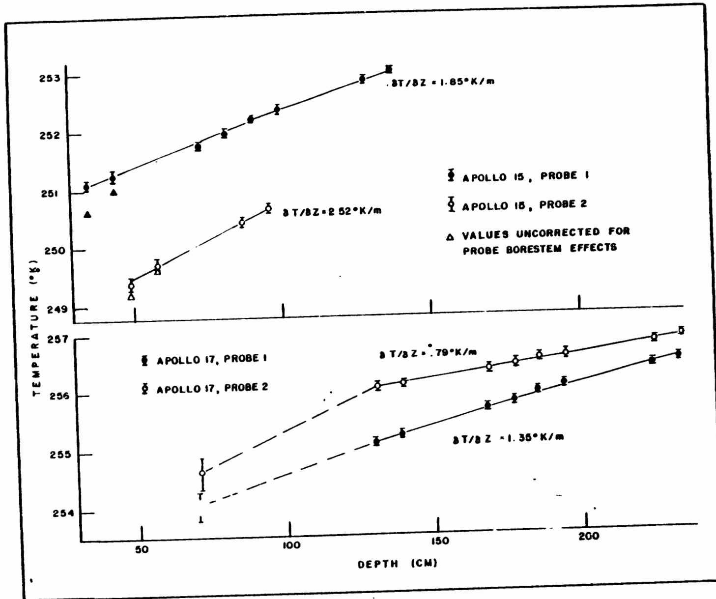
Mean subsurface temperatures at the four probes vs. depth. Note that temperatures of sensors shallower than 65 cm have been corrected upward to account for a steady radiative heat loss to the surface.
