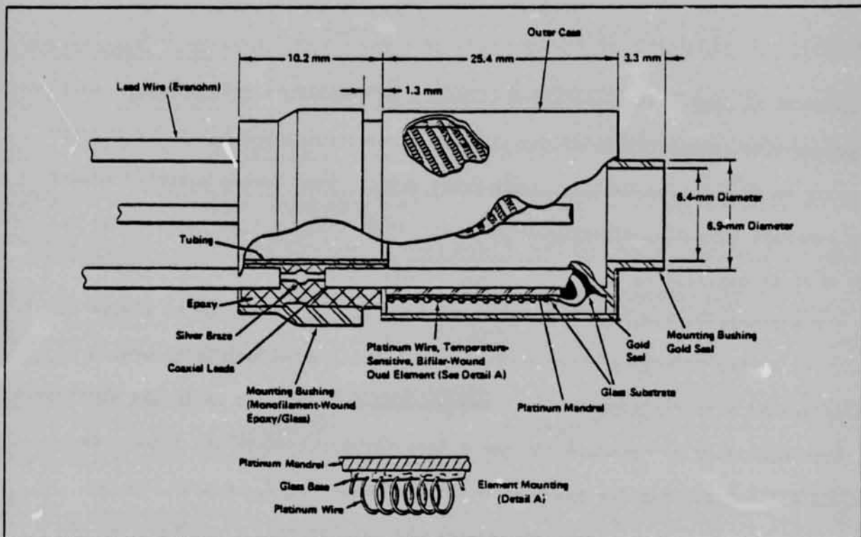
Figure 2 Gradient-Sensor Construction
