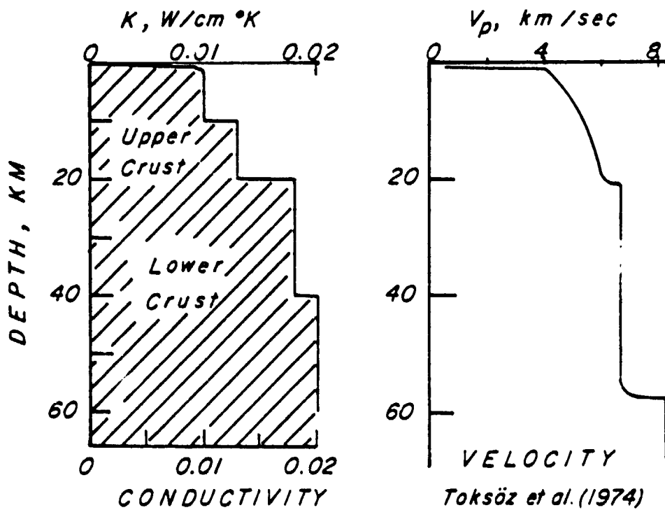
Top: Thermal conductivity versus porosity from laboratory measurements of returned lunar samples as summarized in Horai and Winkler (1976). Bottom: Inferred crustal thermal conductivity profile (left) based on a correlation of porosity and the seismic profile (right) of Toksöz et al. (1974)
