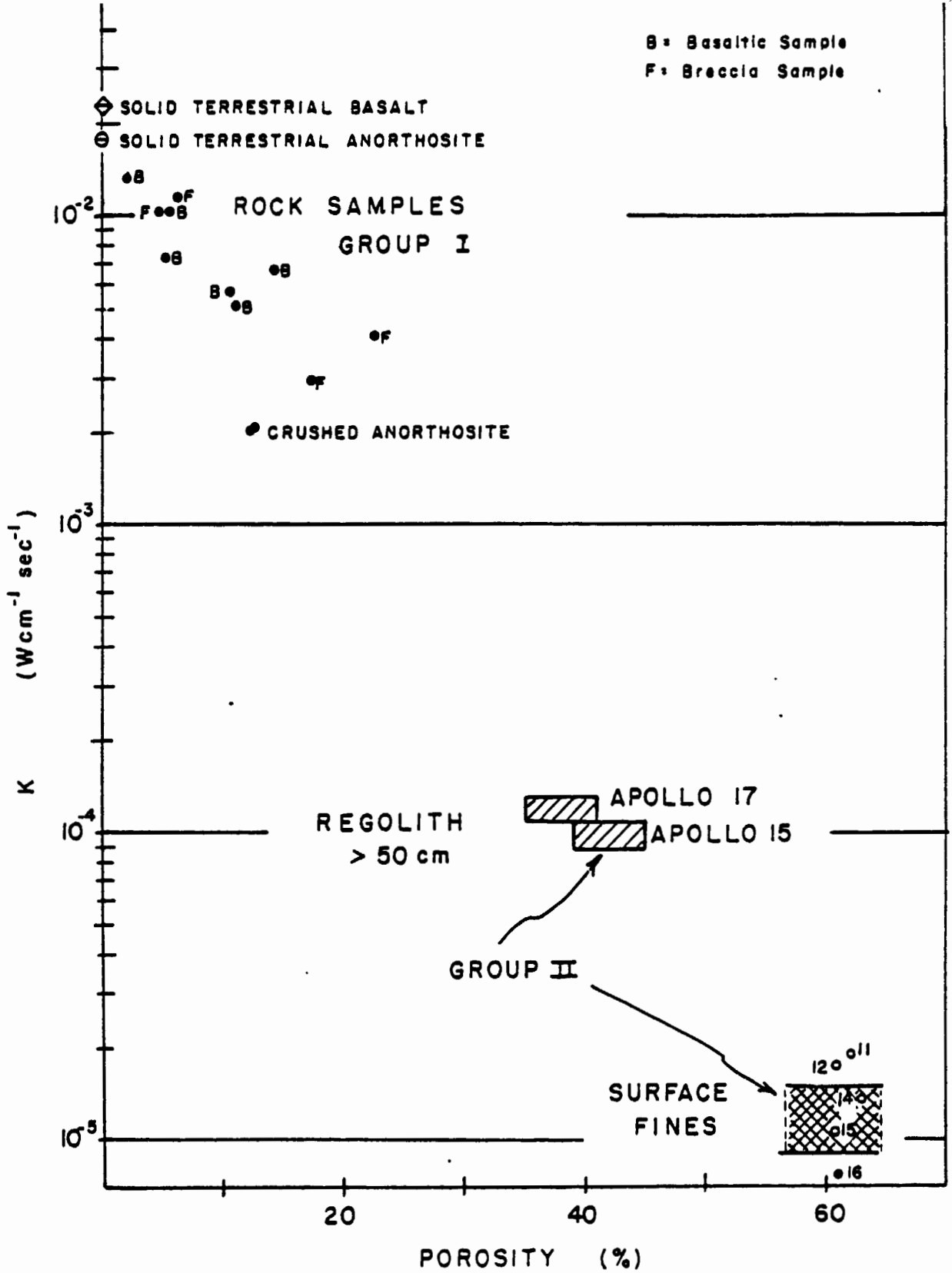
Published conductivity values of lunar materials vs. porosity. For laboratory measurements, values at 300°K are shown as points in the plot. The doubly hatched box is the range of in situ values determined from nighttime cooldown data (Keihm and Langseth, 1973) and the singly hatched boxes are the results reported in this paper. Rock data are summarized in Horai and Winkler (1976) and soil data in Cremers and Hsia (1973)
