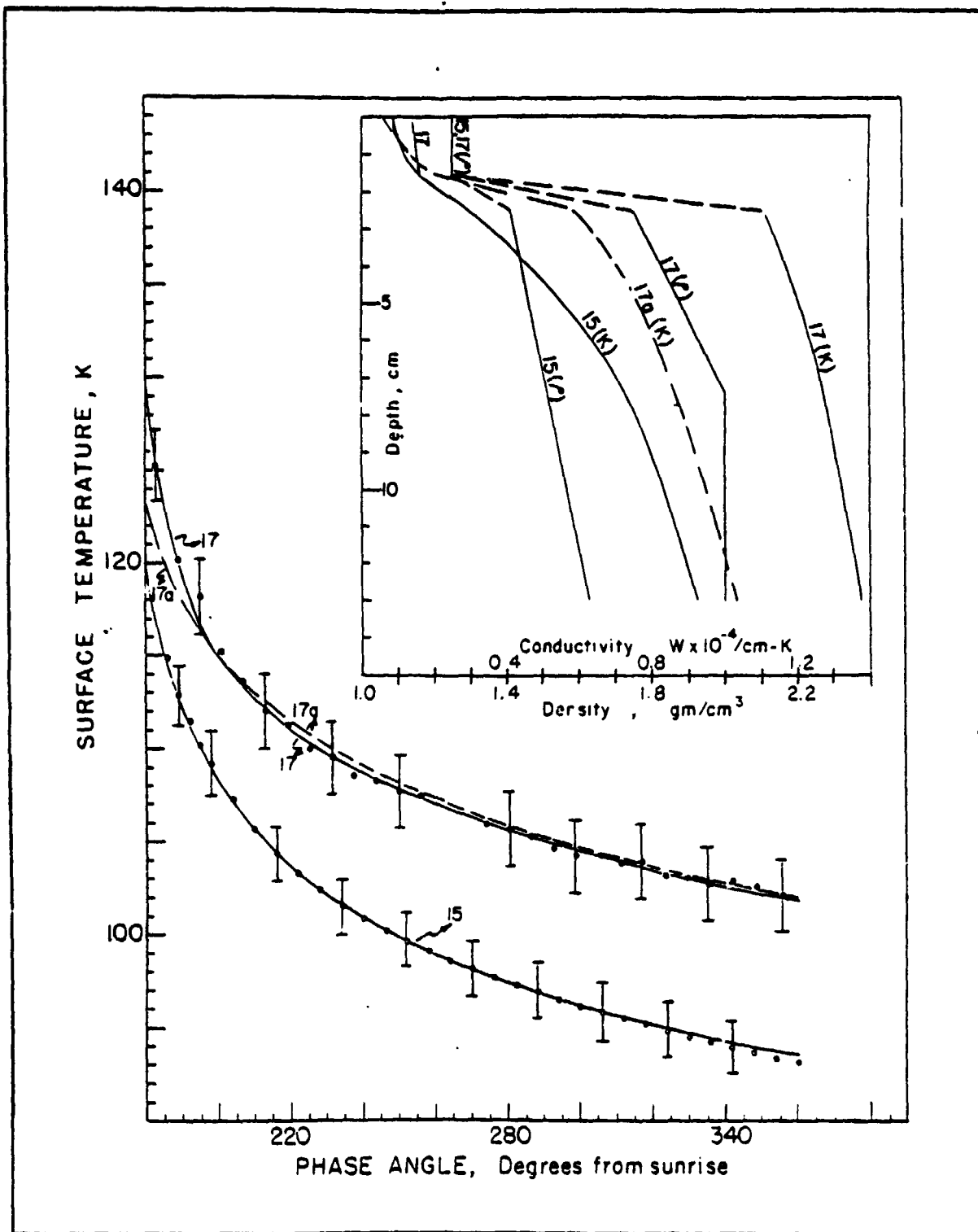
Surface temperatures during the lunar night at the Apollo 17 (solid dots) and Apollo 15 (open circles) heat flow sites. Vertical bars are estimated errors. The continuous curves are theoretical curves derived from the thermal property models shown in the inset.
