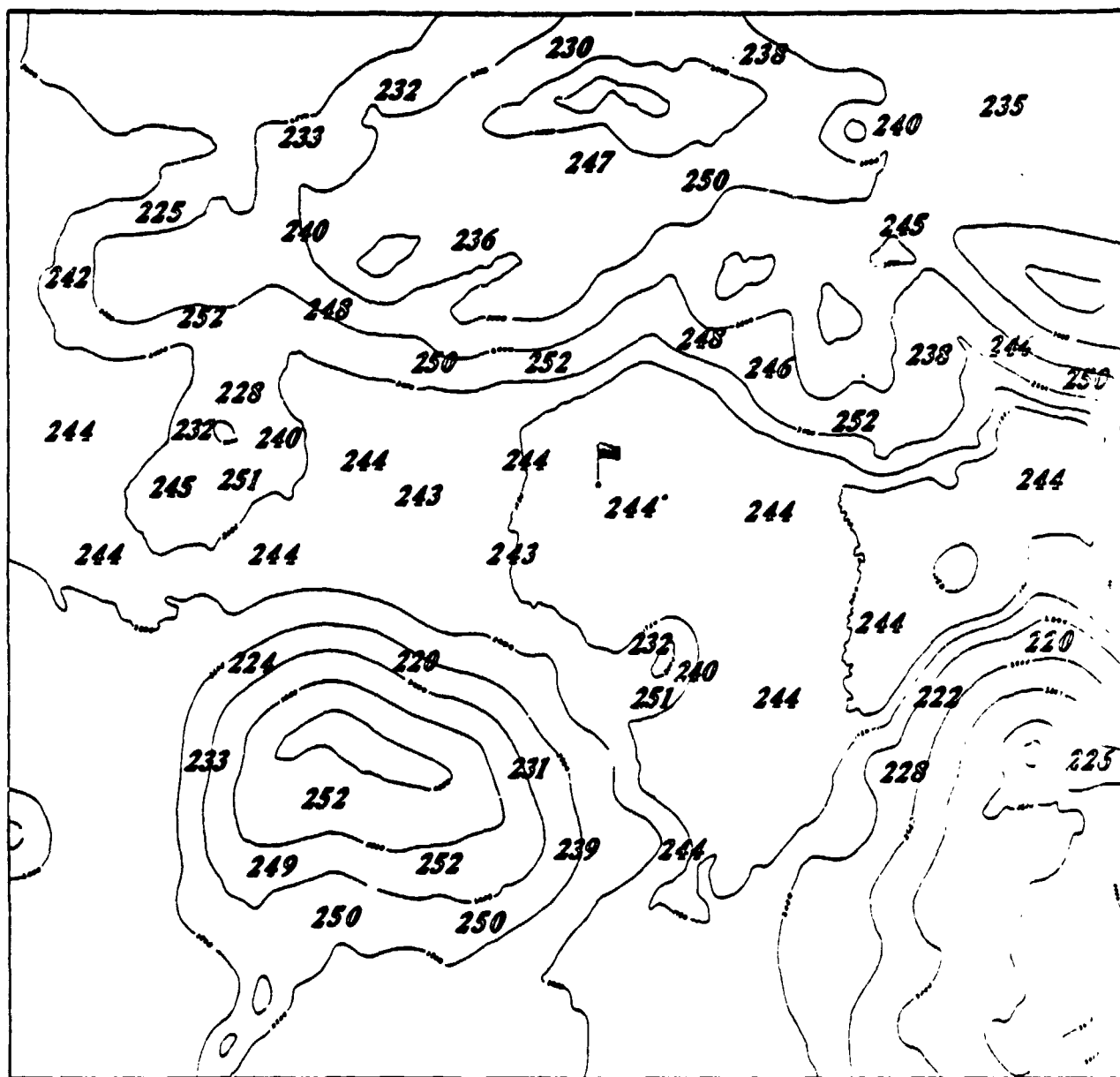
Mean surface temperature ( ^{\circ} K) in the region of Taurus Littrow. The contours represent topography.
