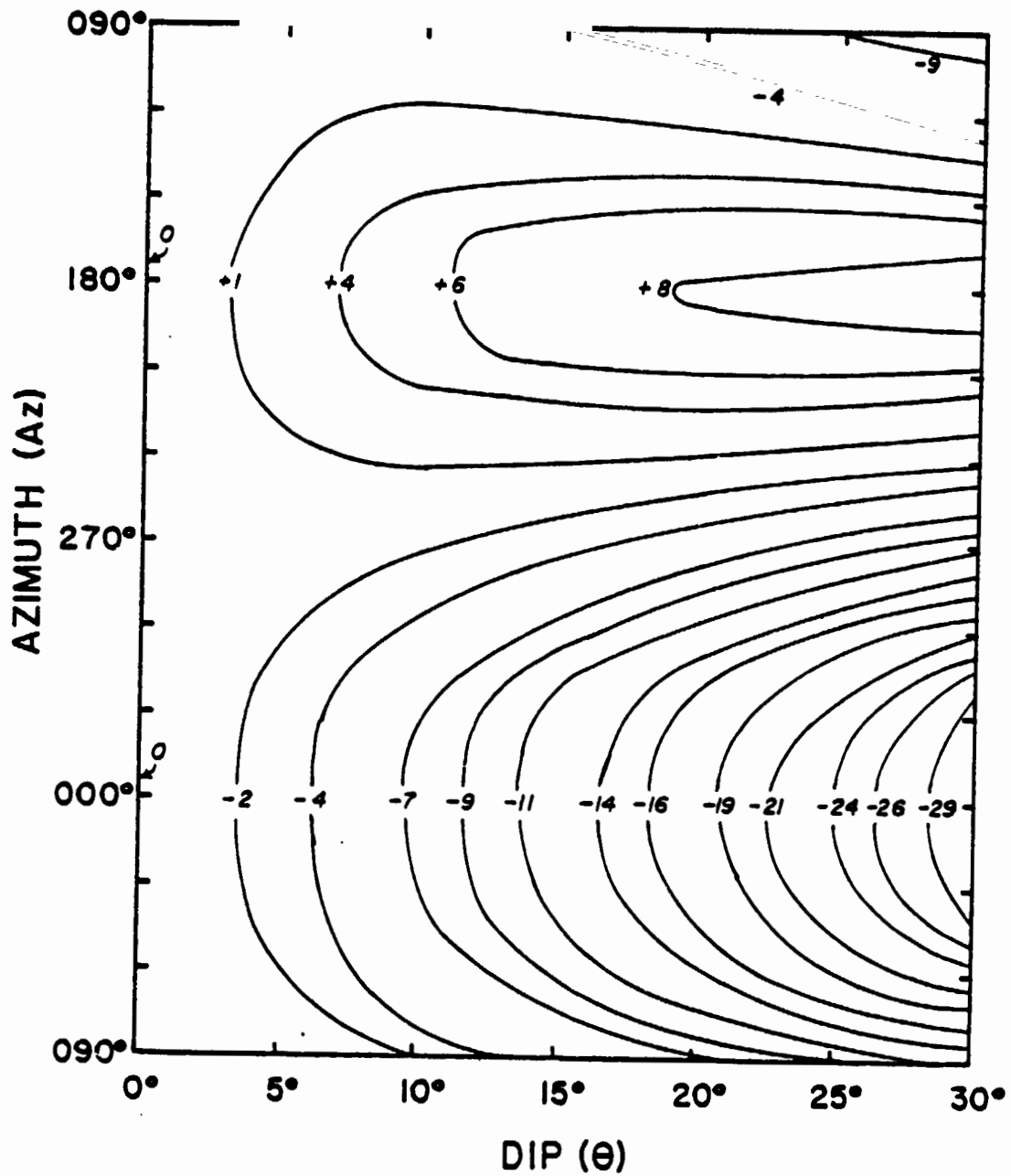
Dependence of mean temperature ten centimeters below the local surface on dip and azimuth angles. The contours represent the deviation ( ^\circ\text{K} ) of mean temperature from that of a flat surface.
