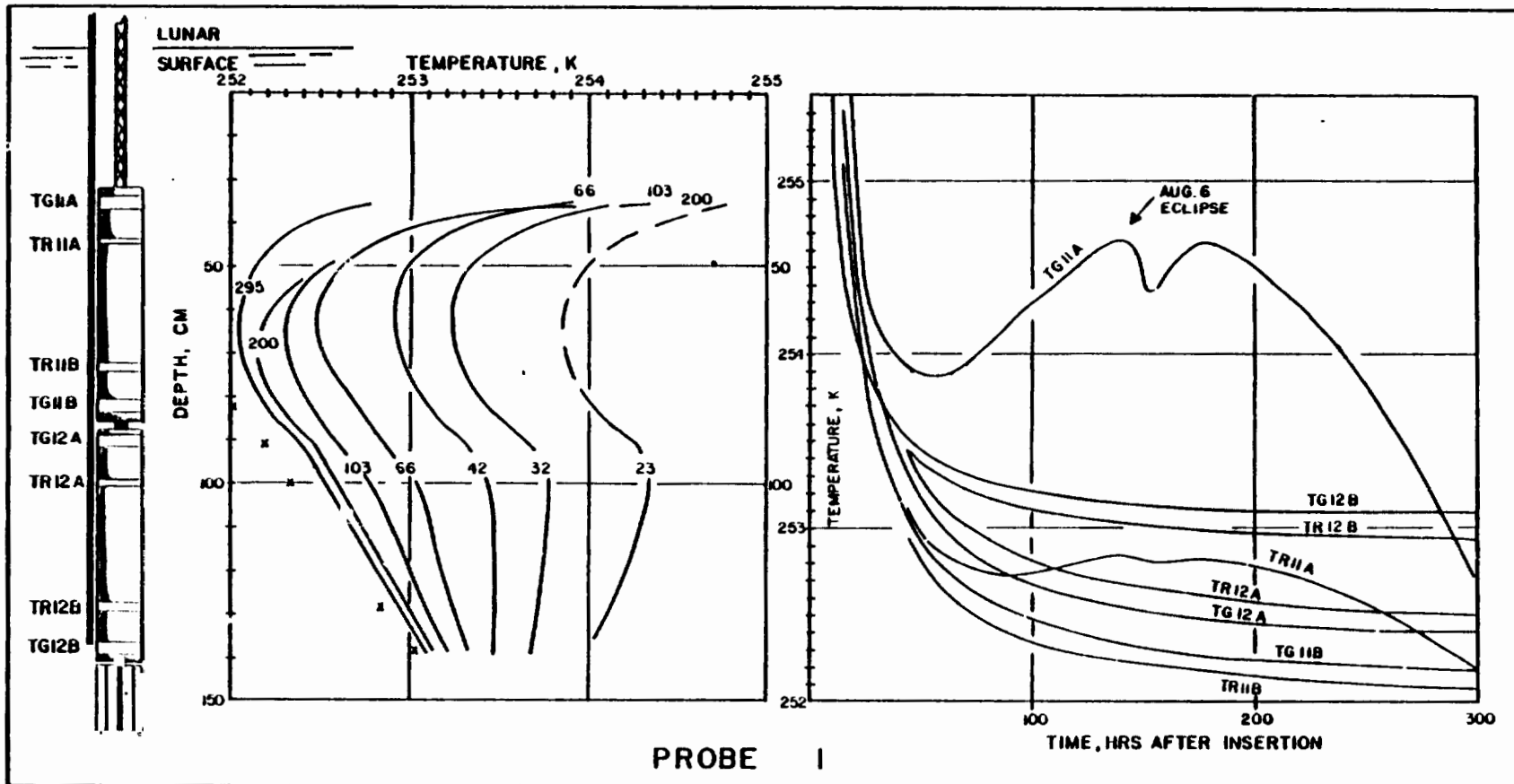
Temperature histories of the sensors on probe 1 during the first 300 hours after emplacement. The subsurface geometry of the probe and temperature as a function of depth are shown on the left. Temperature as a function of time is shown on the right.
