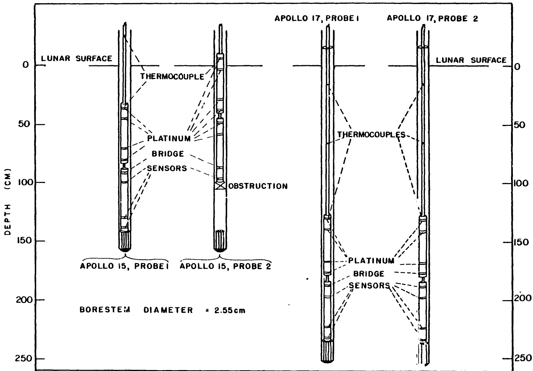
Schematic of final probe emplacement geometries at the Apollo 15 and 17 heat-flow sites
