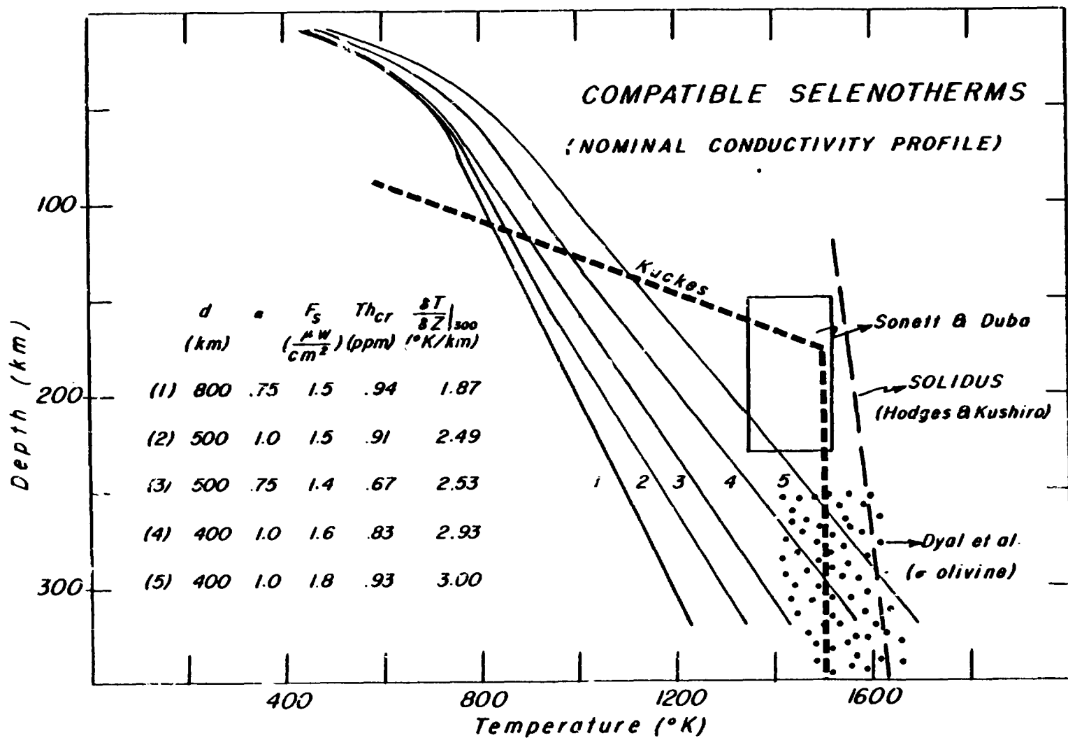
Representative selenotherms calculated for steady-state models. Model parameters for each selenotherm are shown in the accompanying table. The dotted curve, and rectangular and stippled regions are upper mantle temperature estimates from the magnetometer data (Kuckes, 1974; Sonett and Duba, 1975; Dyal et al., 1976). The solidus of Hodges and Kushiro (1974) is shown for reference
