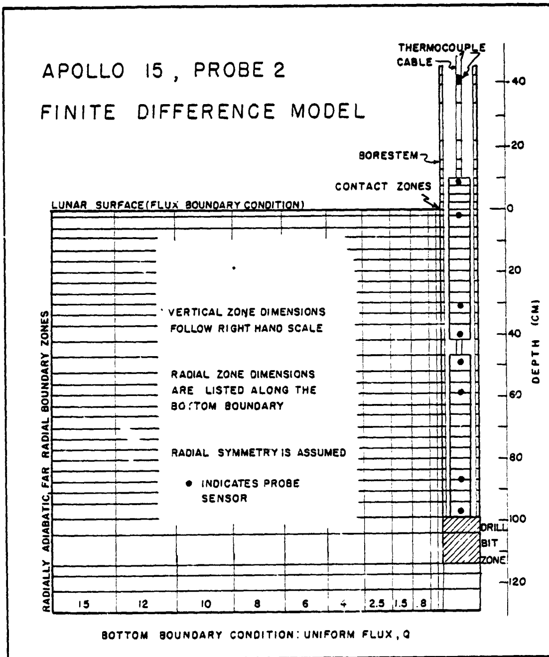
Schematic of Apollo 15 probe 2 numerical model
