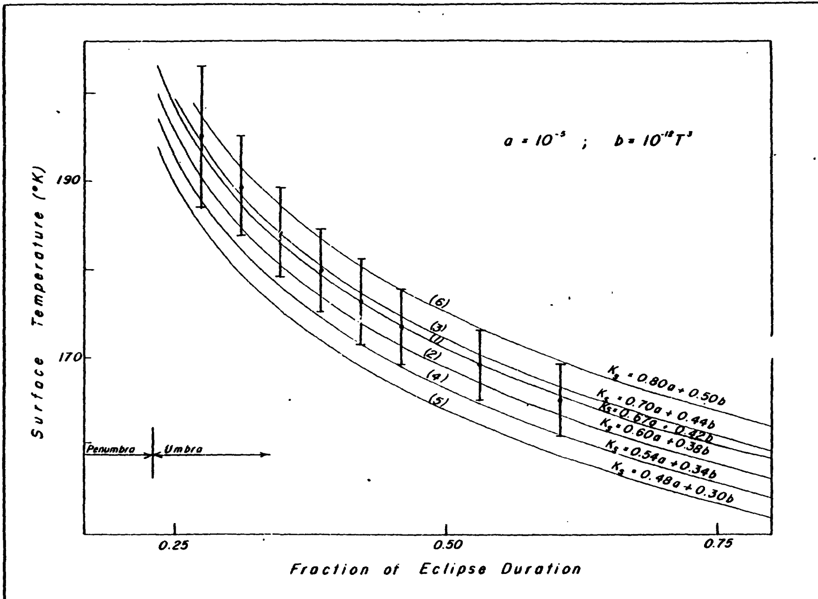
Surface temperature history during the umbral phase of the lunar eclipse of August 6, 1971. The vertical bars span a range of two standard deviations centered at the reduced surface temperature measurement. The solid lines represent computer generated models characterized by conductivity functions, K_s(T) , for the top centimeter.
