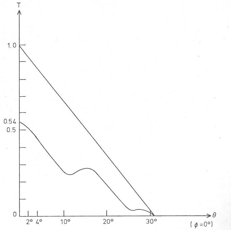
Figure 4: Transmission function of the X-ray spectrometer compared to a triangular response function (Adler et al. [1975]).
