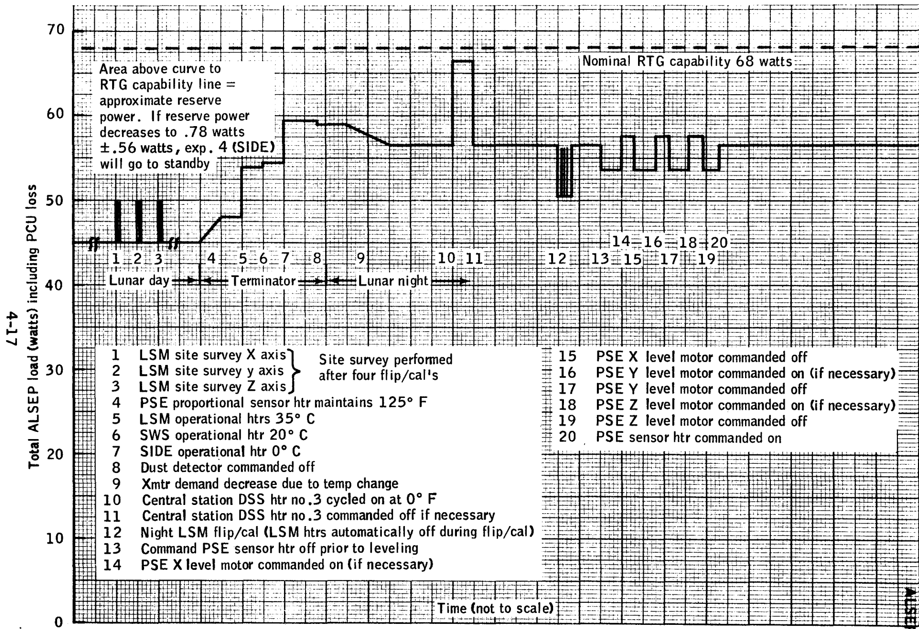
Figure 4-7.- Lunar day to night power profile.
