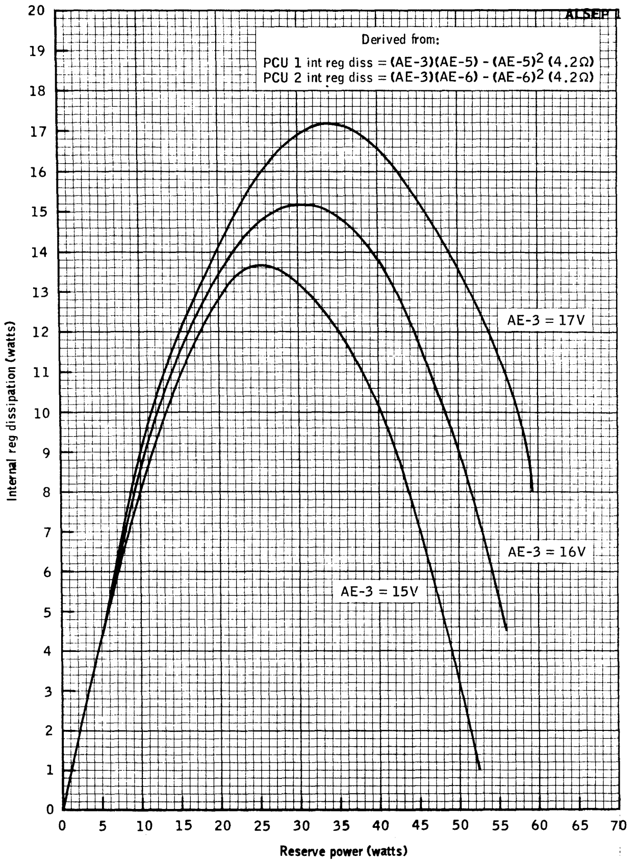
Figure 4-8.- Internal regulator dissipation.
