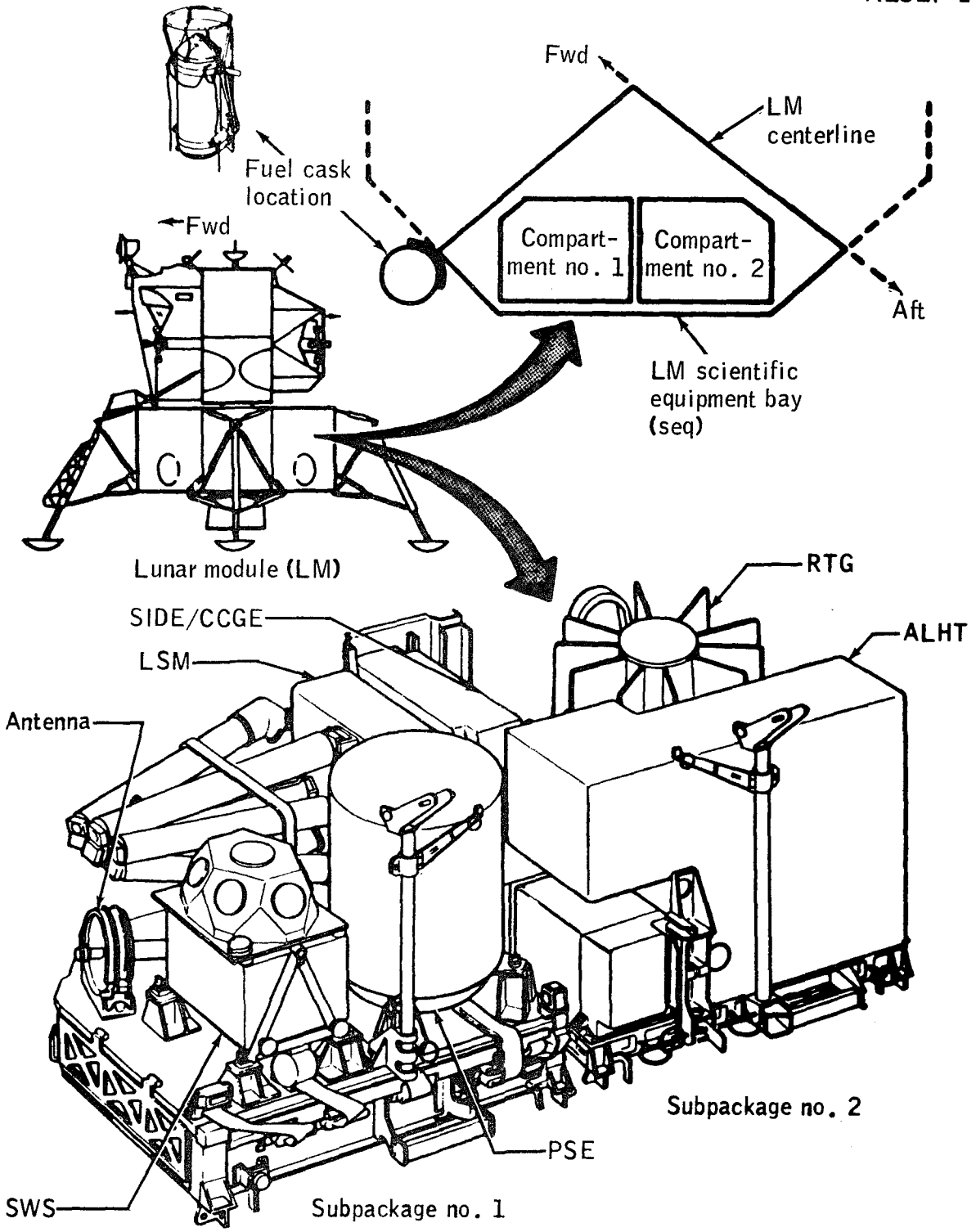
Figure 2-1.- ALSEP/LM interface.
