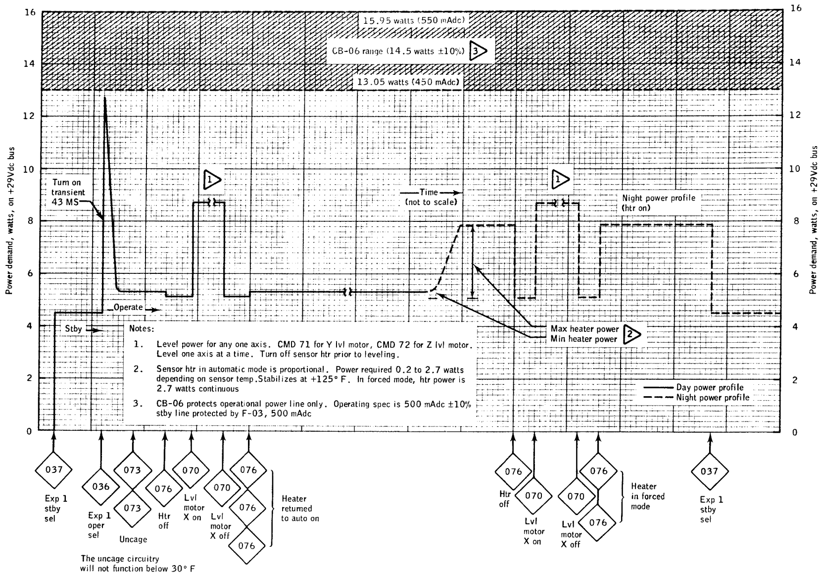
Figure 8-1.- PSE power profile.
