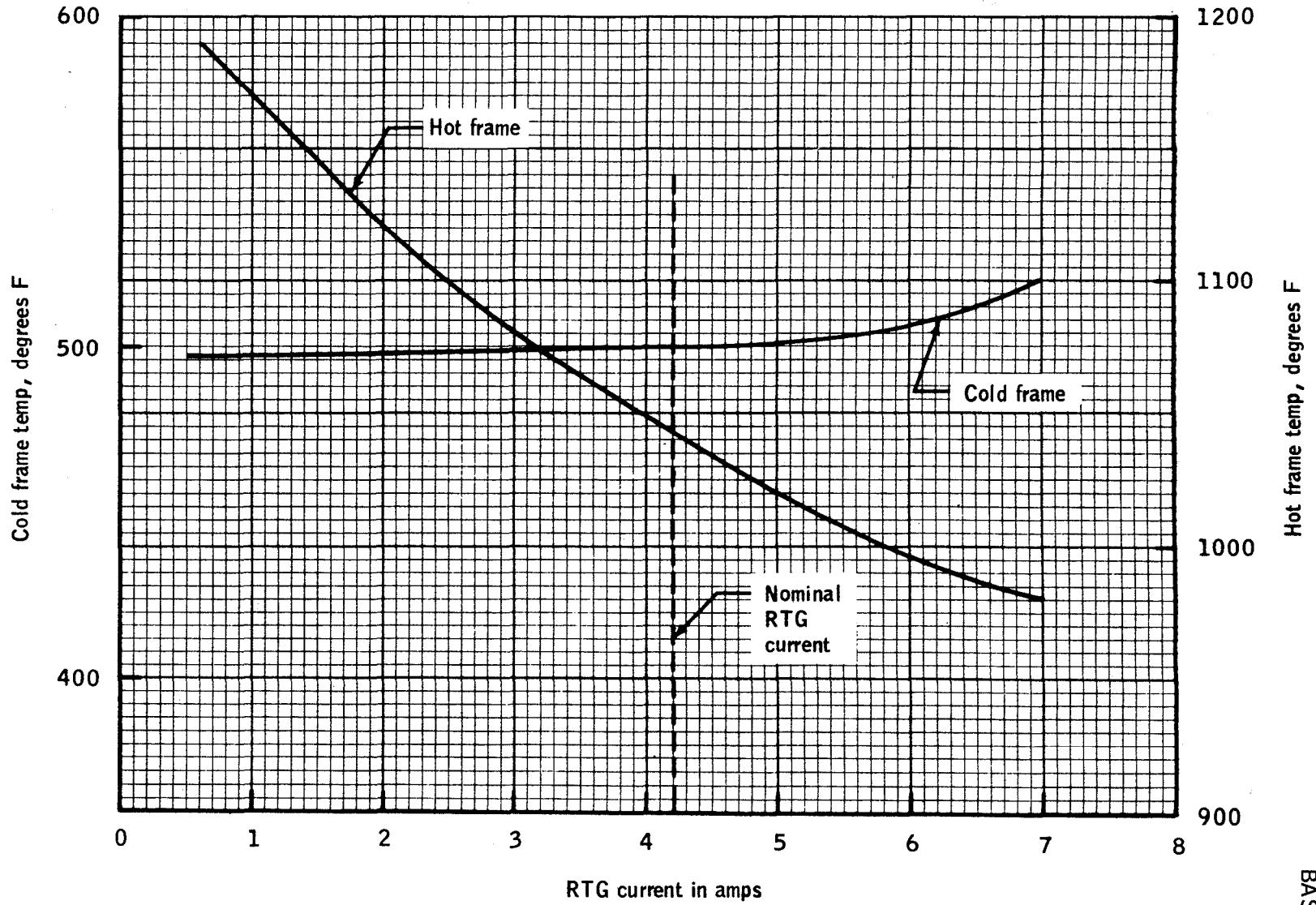
Figure 4-2. - RTG hot and cold frame temps vs RTG current (typical).
