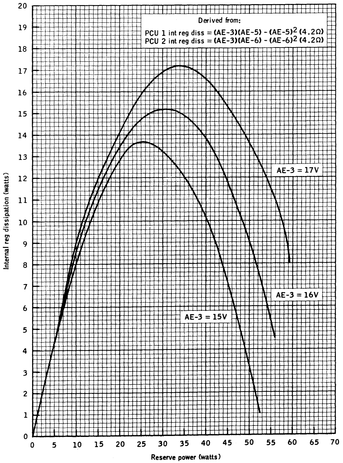
Figure 4-5. - Internal regulator dissipation.
