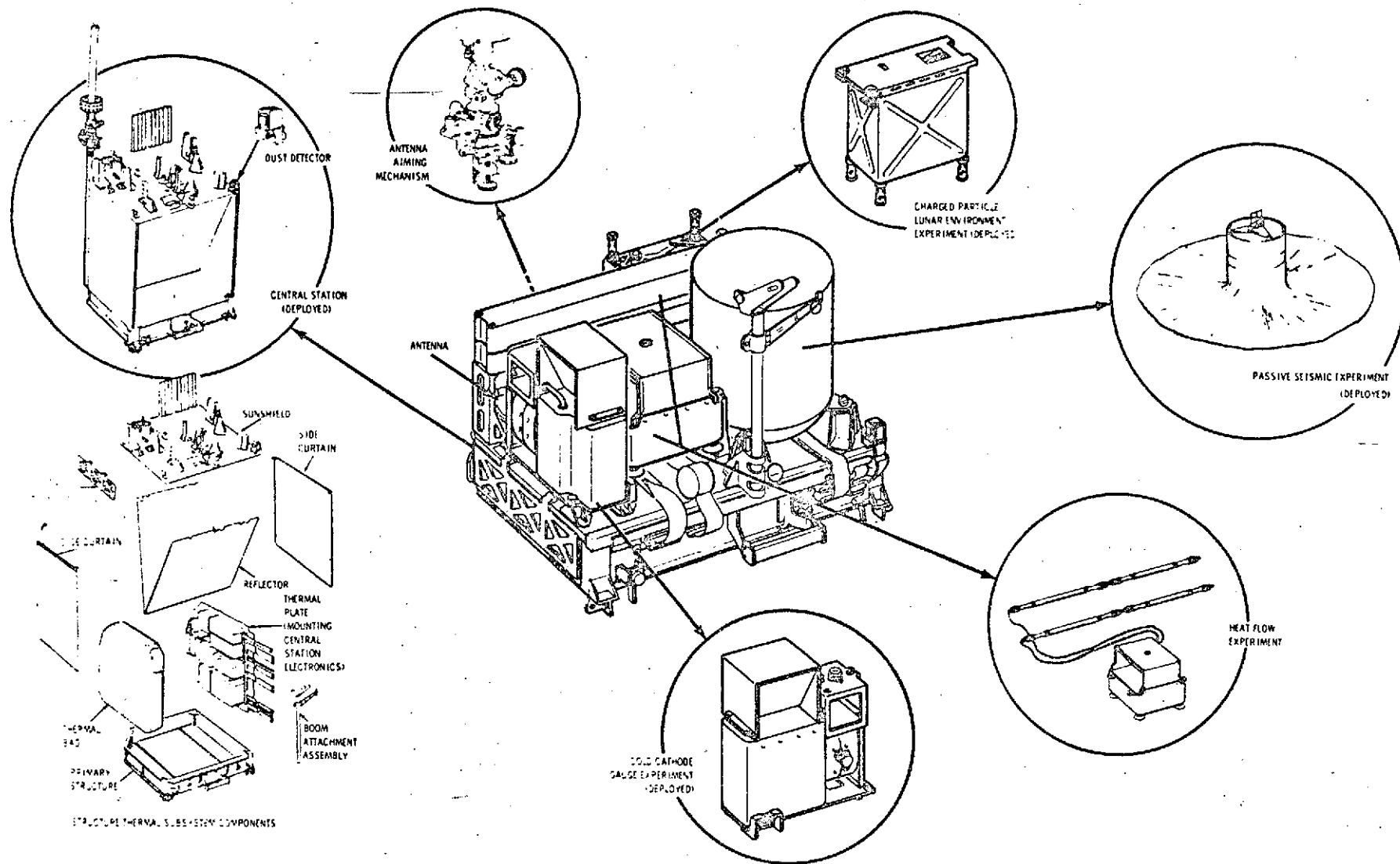
Figure 3 ALSEP Subpackage 1 (Array B Configuration)
