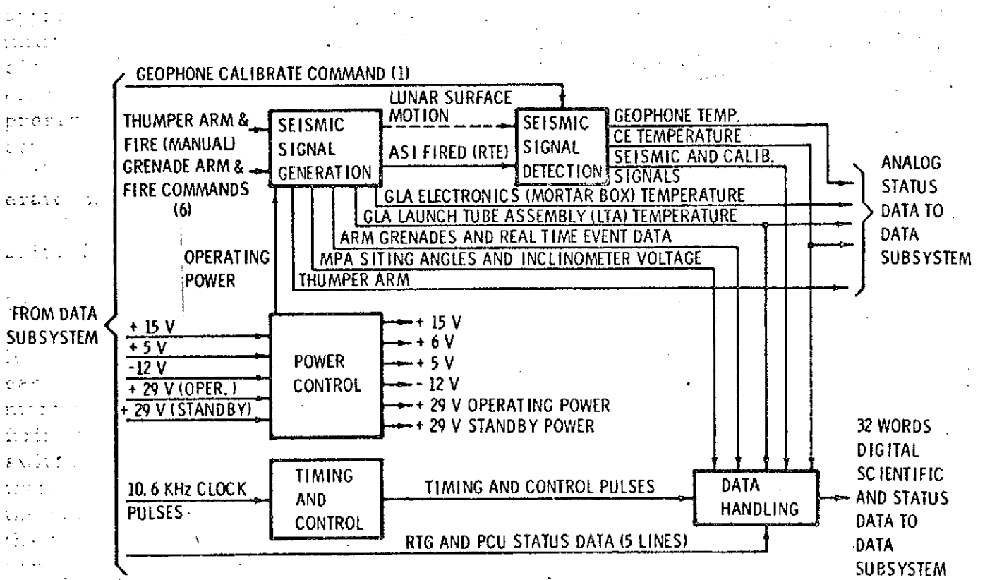
Figure 11 Active Seismic Experiment, Functional Block Diagram
