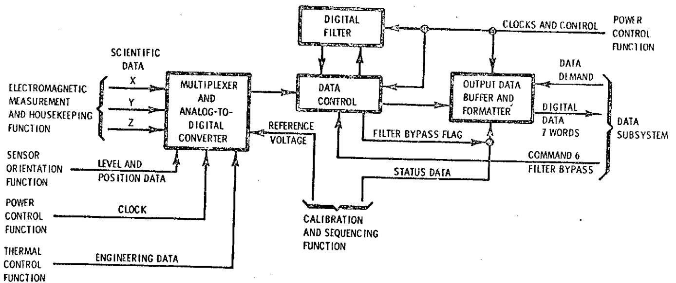
Figure 2.8-2 LSM Data Handling Function, Block Diagram
