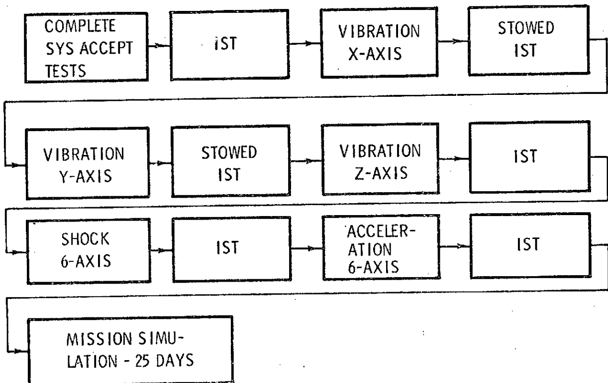
Figure 21 System Level Qualification Tests, Flow Diagram
