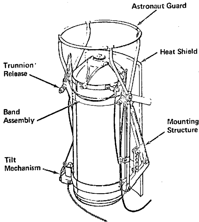
Figure 8 Fuel Cask Assembly
