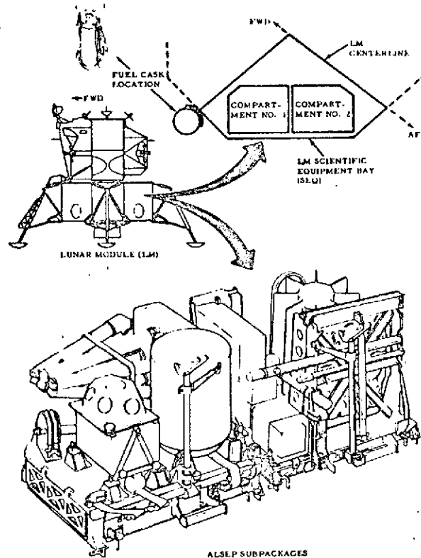
Figure 1 ALSEP/Lunar Module Interface
