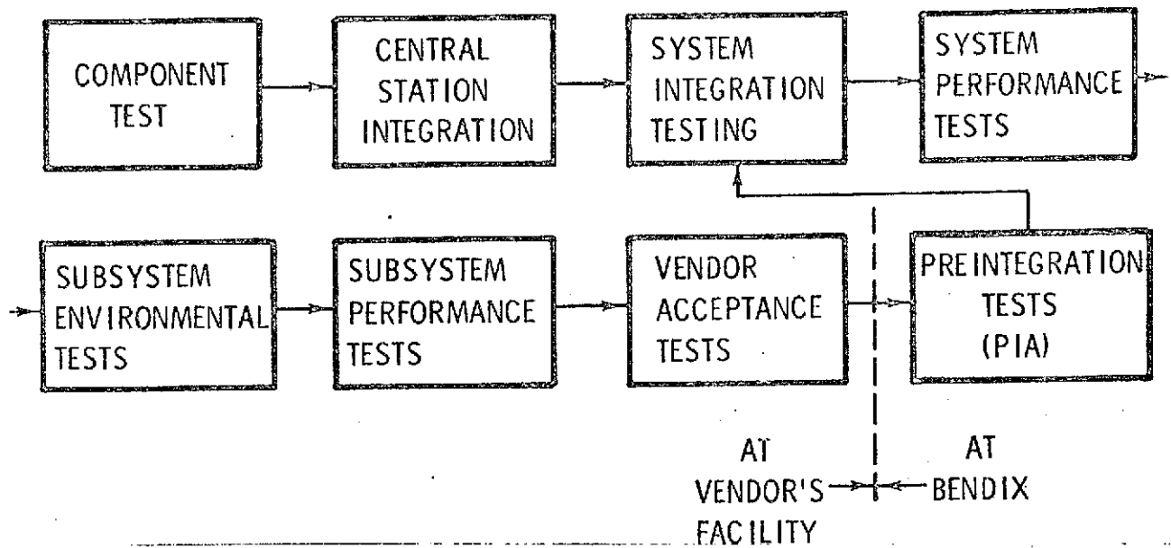
Figure 22 Flight System Acceptance Tests, Flow Diagram
