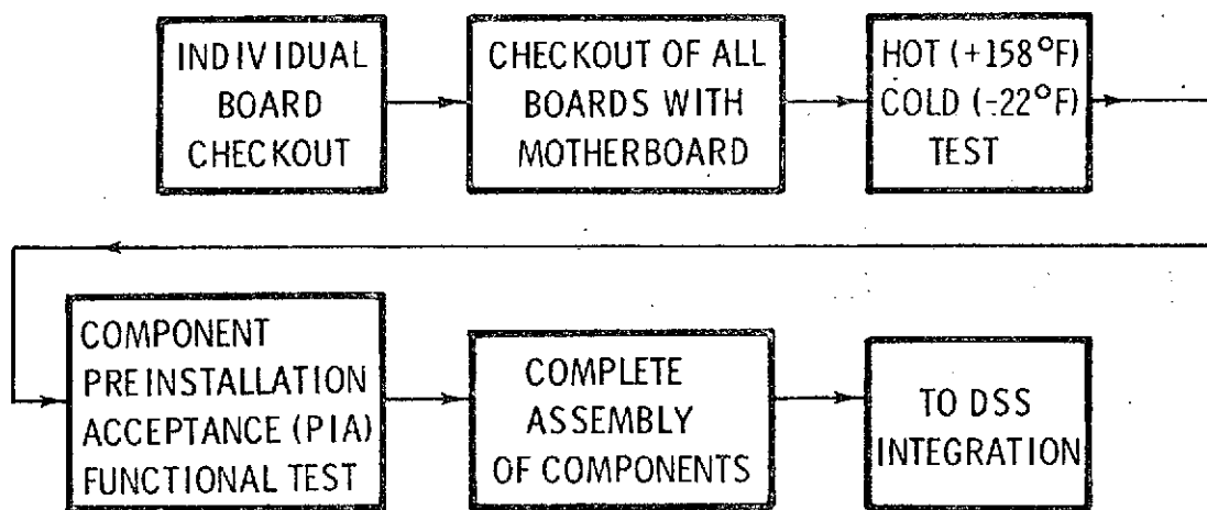
Figure 23 Component Acceptance Tests, Flow Diagram
