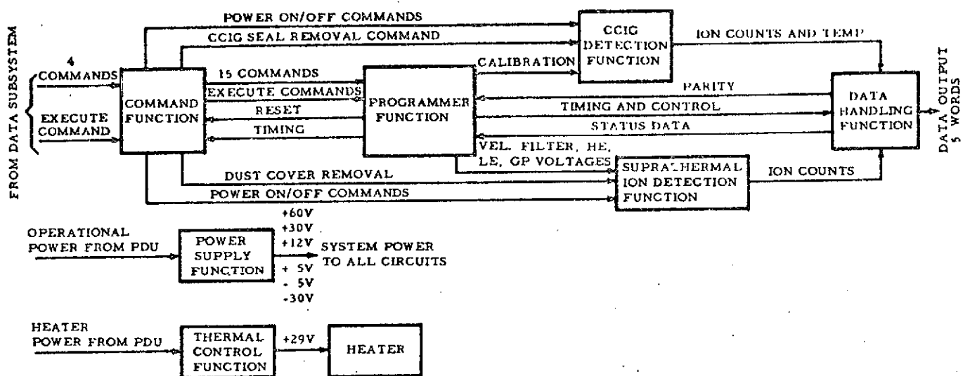
Figure 2.9-1 Suprathermal Ion Detector Experiment, Functional Block Diagram
