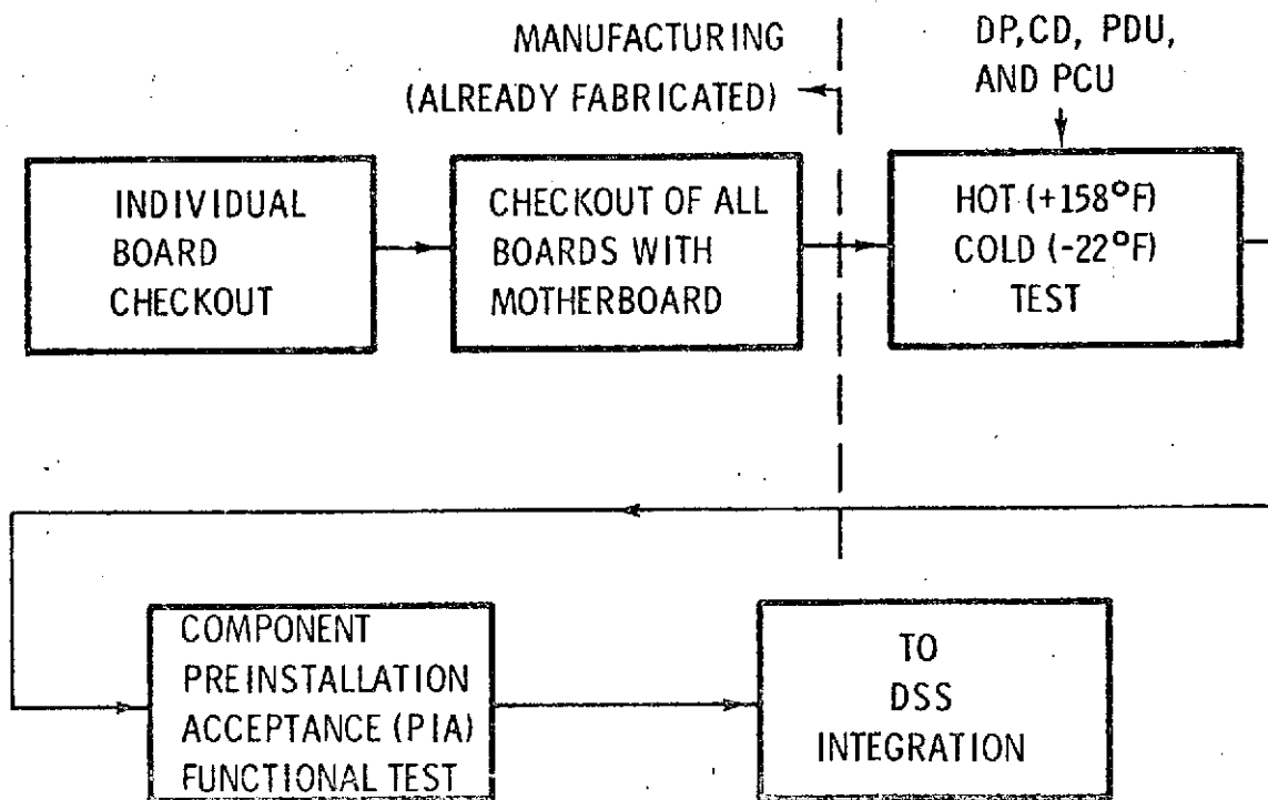
Figure 17 Prototype Component Tests, Flow Diagram
