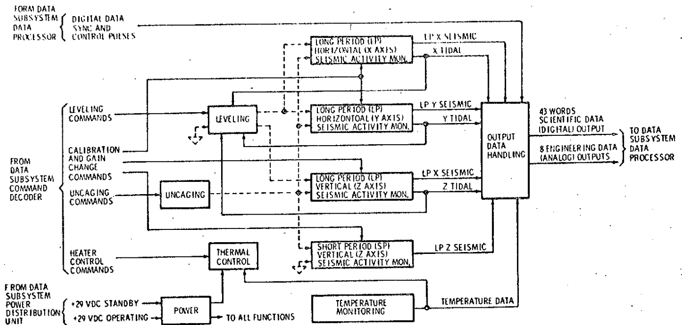
Figure 10 Passive Seismic Experiment, Functional Block Diagram
