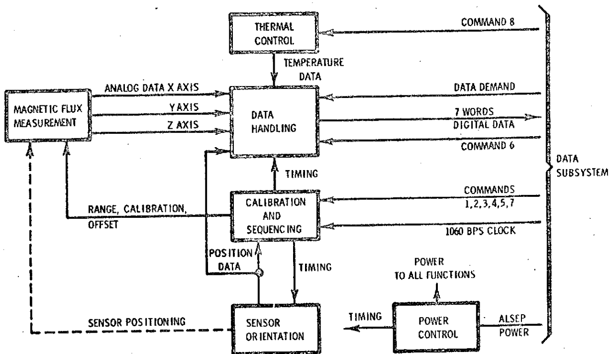
Figure 2.8-1 Magnetometer Experiment, Functional Block Diagram
