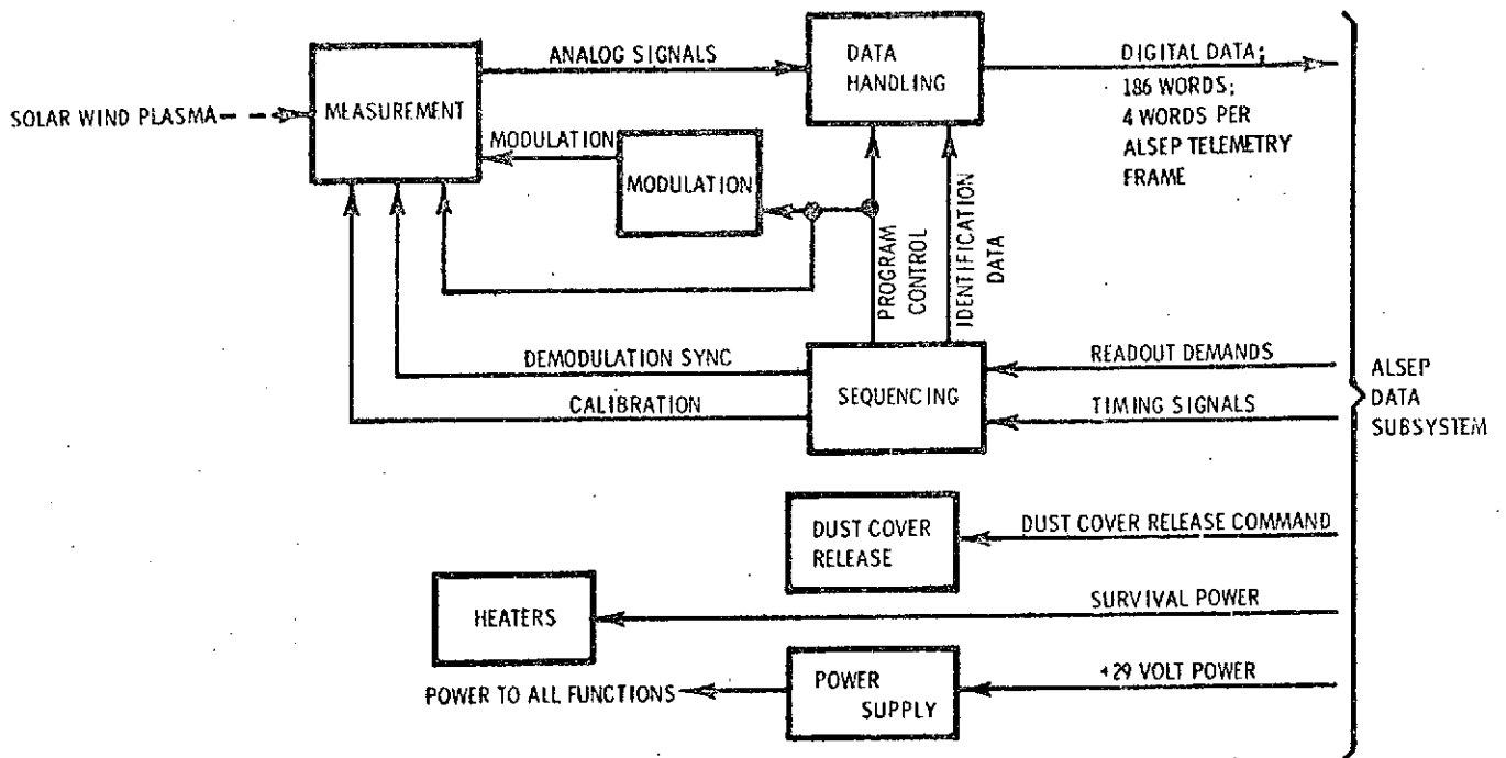
Figure 2.10-2 SWE, Functional Block Diagram
