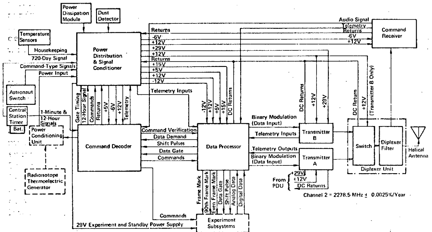
Figure 9 ALSEP Data Subsystem
