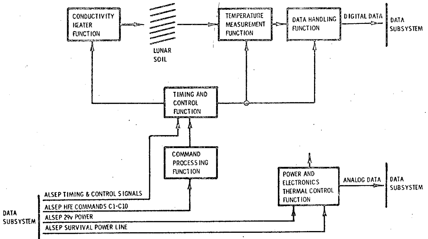
Figure 13 Heat Flow Experiment, Functional Block Diagram
