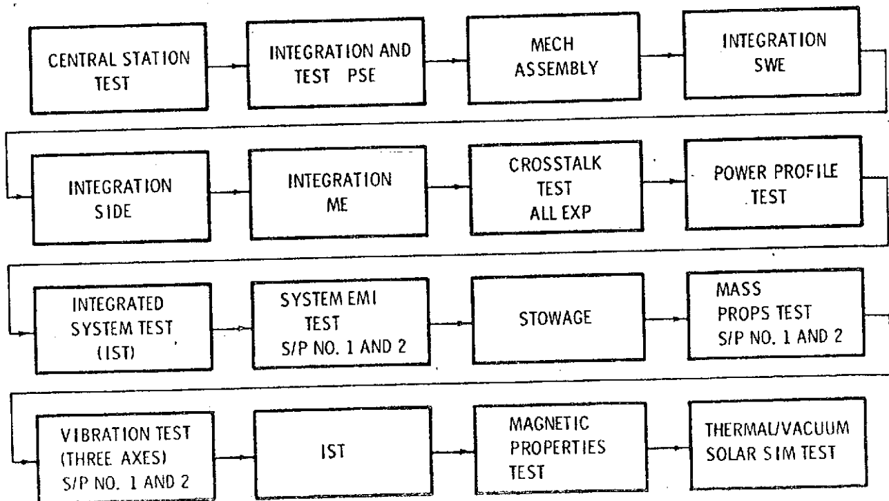
Figure 20 Prototype System Integration and Tests, Flow Diagram
