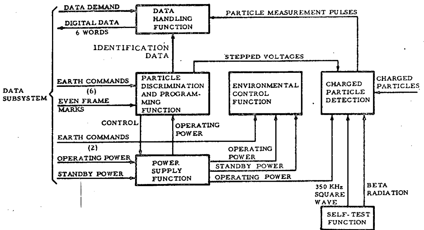
Figure 12 Charged Particle Lunar Environment Experiment, Functional Block Diagram
