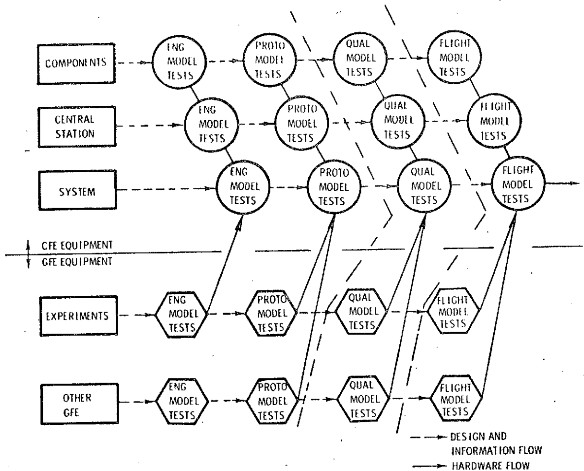
Figure 15 ALSEP Test Program, Flow Diagram
