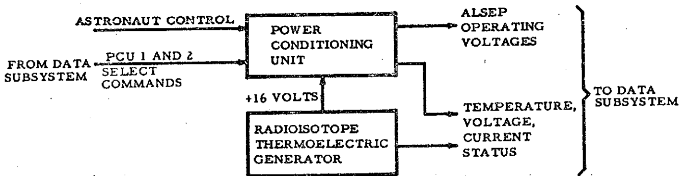
Figure 2.3-1 Electrical Power Subsystem, Functional Block Diagram
