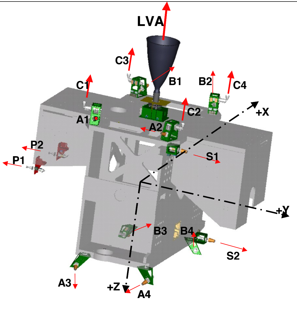
Figure 1 Thruster Locations and Thrust Directions
