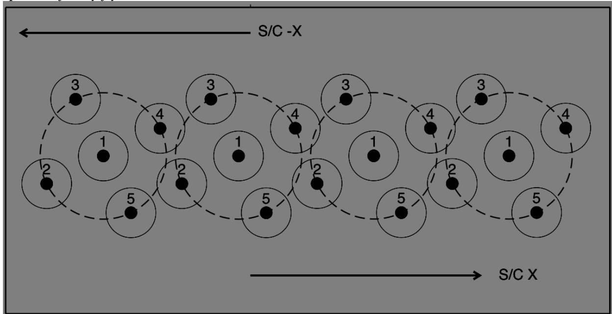
Figure 1: LOLA ground spot pattern sample of four successive shots, with channels numbered. Spacecraft may fly in either +X or -X direction.
