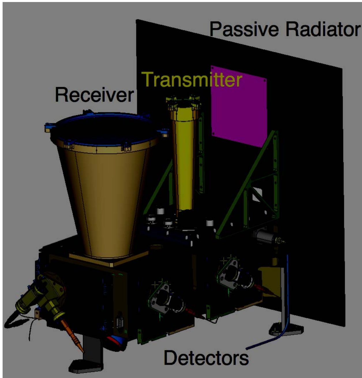
Figure 2: LOLA Optical Transceiver Assembly.
