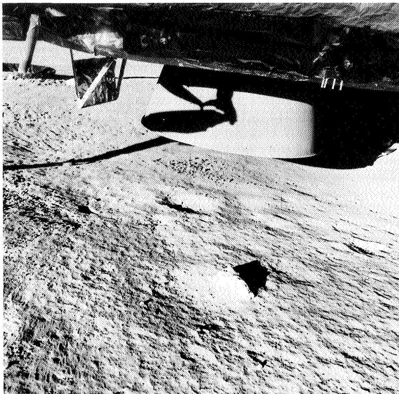
FIGURE 1-10.—The LM-inspection procedure included detailed examination and documentation of the surface materials eroded by the plume of the descent engine. The grooving that indicates radial transport of material from the point below the engine is evident. The erosion did not destroy small craters under the engine bell. The prominent rock in the foreground was later collected as a sample (AS14-66-9261).
