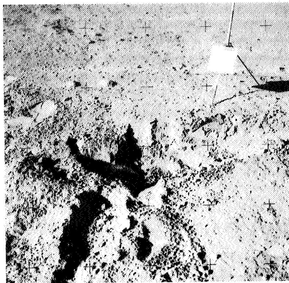
FIGURE 4-17.—View of the trench from the northeast. The steepest sidewalls are estimated at 65^{\circ} to 80^{\circ} . A pile of excavated material is at the end of the trench at the left in the photograph (AS14-64-9161).
