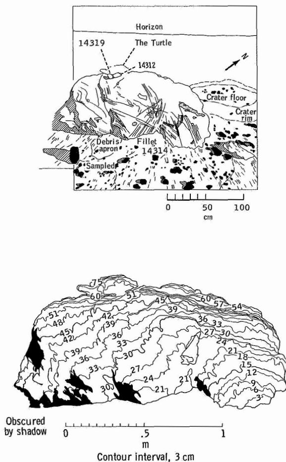
FIGURE 3-25.—Fillet on Turtle Rock at station H.
