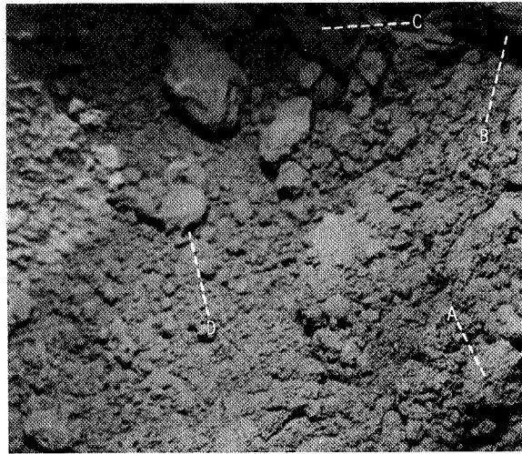
FIGURE 14-11.—Soil-covered rock surface (AS14-77-10373).
