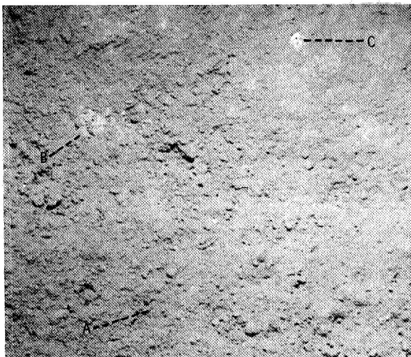
FIGURE 14-10.—Soil-covered rock surface (AS14-77-10372).
