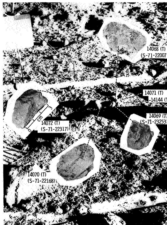
FIGURE 3-39.—Samples 14068 to 14072 and sample 14144 before collection.
