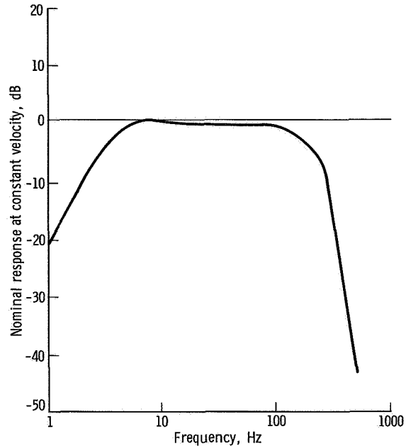
FIGURE 7-5.—Frequency response of the ASE.
