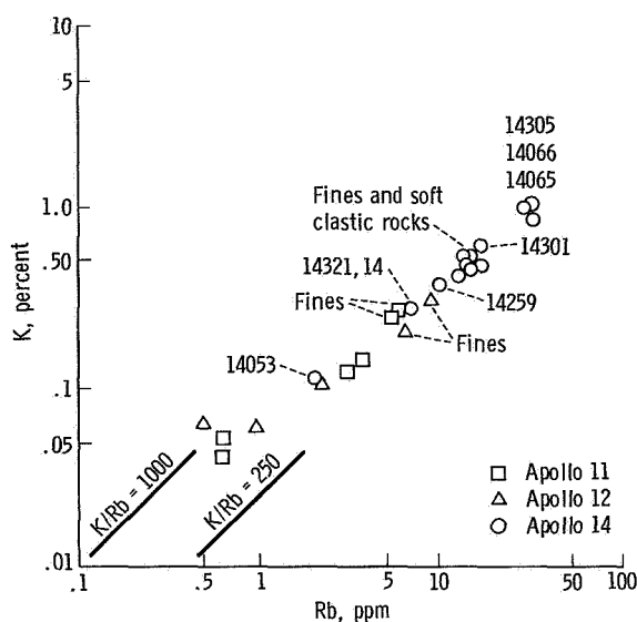
FIGURE 5-11.—The K/Rb relationship for Apollo 14 rocks and soils compared with selected Apollo 11 and 12 rocks and average soils.
