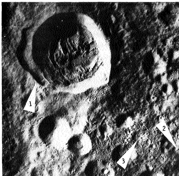
FIGURE 18-23.—Copernican-age crater (35-km diameter) forming one of the major ray systems on lunar far side. Point 1 indicates uppermost scarp of a series of slump terraces; point 2, a secondary crater loop; and point 3, radial-rim facies (north right of top center; AS14-70-9671).
