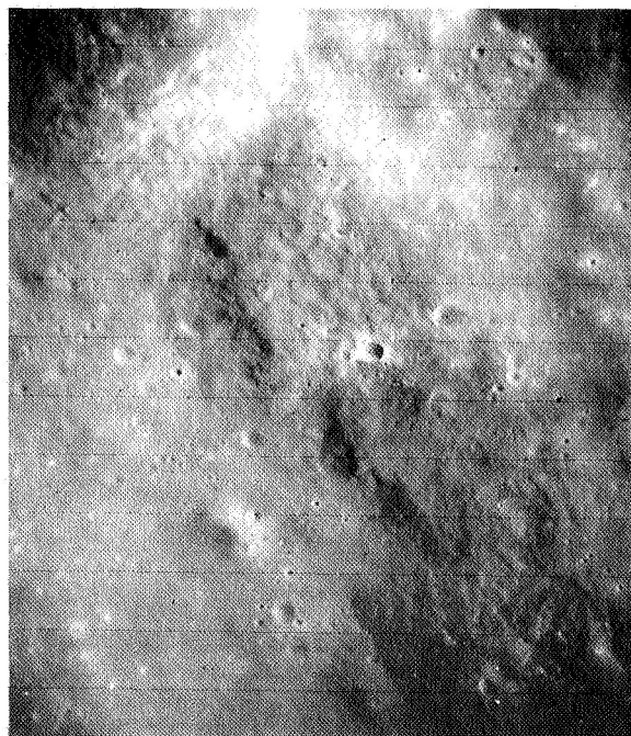
FIGURE 18-31.—Numerous linear arrangements of blocks on the rim of Theophilus Crater (AS14-80-10441).
