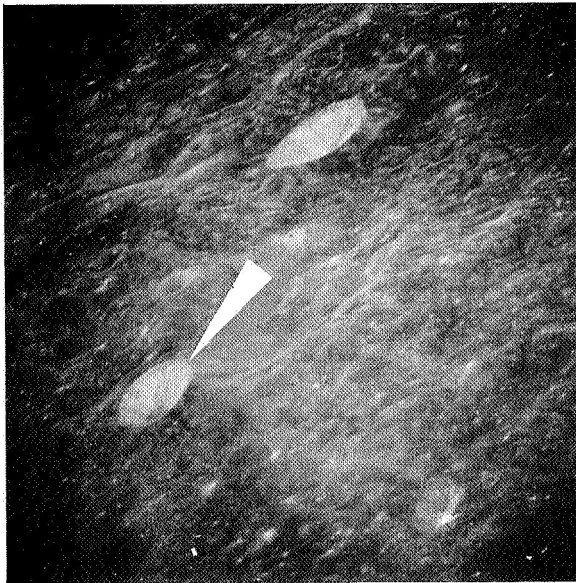
FIGURE 18-14.—Cyrillus G Crater (7.5-km diameter) near Beaumont L Crater (north toward lower right; AS14-73-10047).
