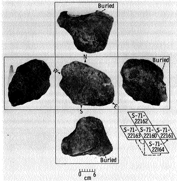
FIGURE 3-54.—Orthogonal views of sample 14321 in approximate lunar orientation.
