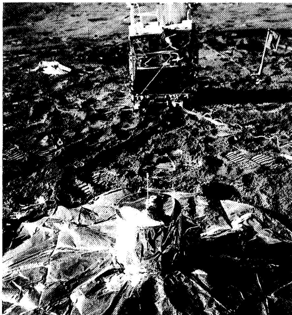
FIGURE 6-2.—Seismometer after deployment on the lunar surface (AS14-67-9363).
