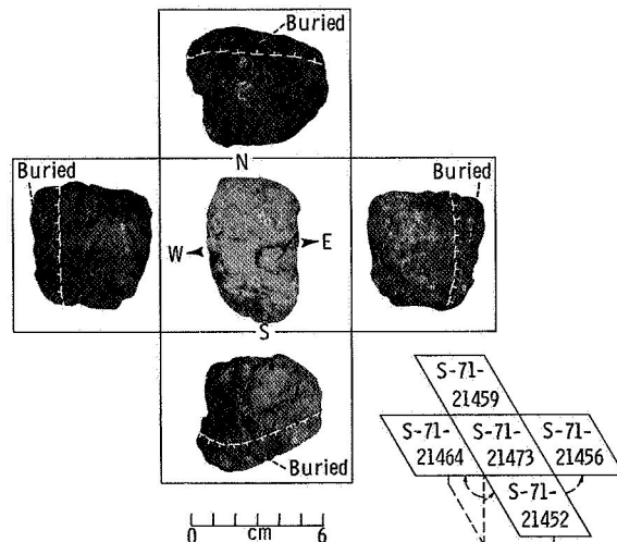
FIGURE 3-37.—Orthogonal views of sample 14051 in approximate lunar orientation.
