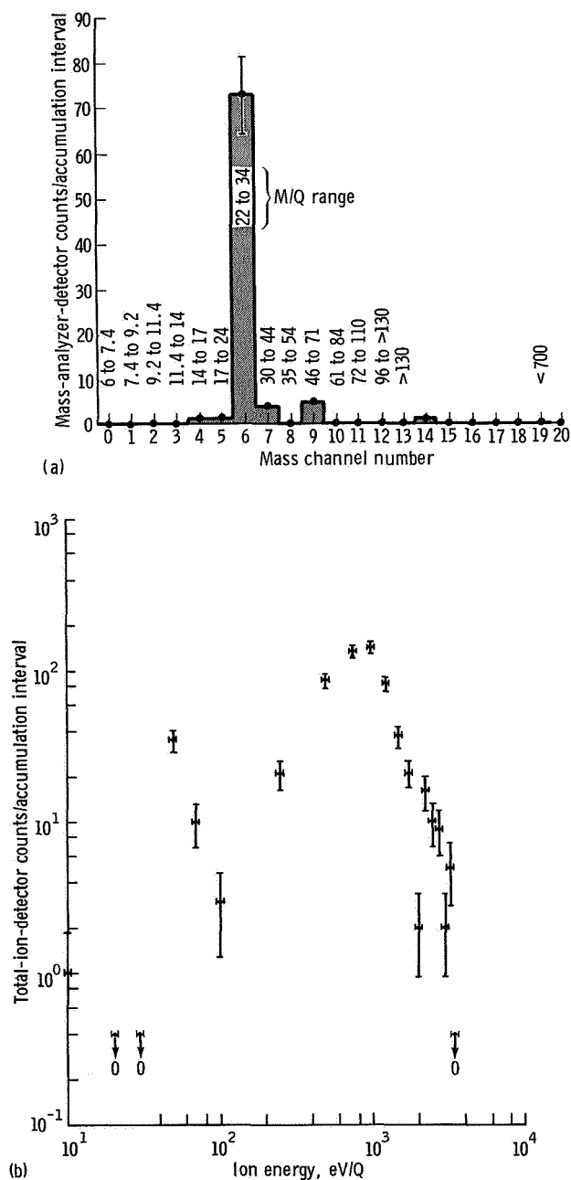
FIGURE 8-8.—Spectra recorded as a result of the ionization of the vented LM oxygen atmosphere at the beginning of the second period of EVA, February 6. (a) Mass-analysis-detector spectrum recorded 08:38:25 to 08:38:48 G.m.t., at 48.6 eV. (b) Total-ion-detector energy spectrum recorded 08:38:26 to 08:38:49 G.m.t.
