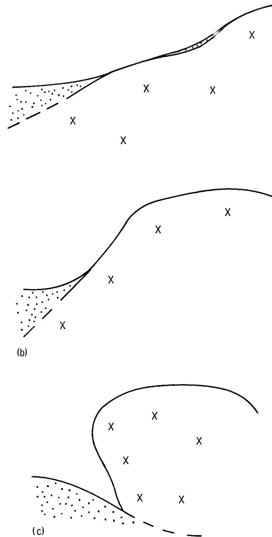
FIGURE 3-18.—Types of fillet contacts between rocks and soil. (a) Shallow, with thin pockets of dust high on rock surface. (b) Steep, with concave fillet against base of rock. (c) Overhanging, with little or no resulting fillet.
