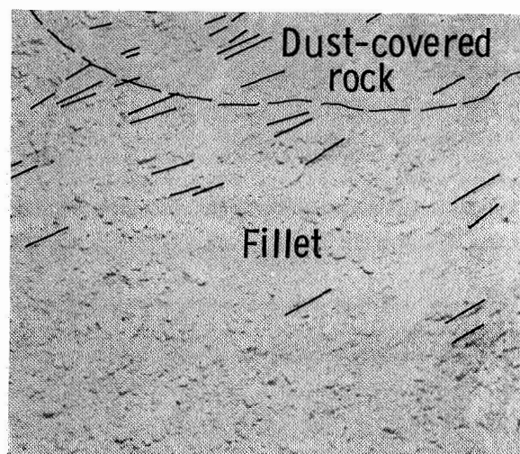
FIGURE 3-26.—Closeup photograph of fillet on Sloping Rock.
