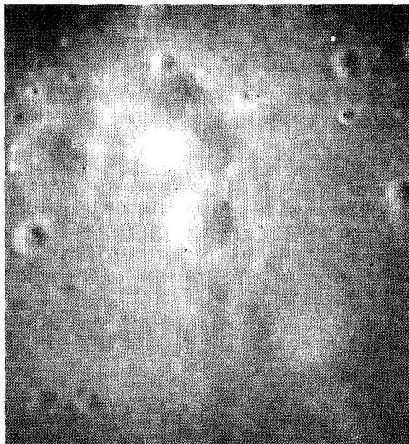
FIGURE 18-33.—Blocks on the crater rims and basal slopes of central peaks of several large craters in floor of Theophilus Crater (AS14-80-10466).
