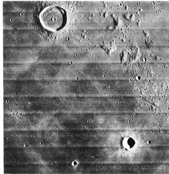
FIGURE 18-49.—Lunar Orbiter 4 high-resolution photograph of area.
