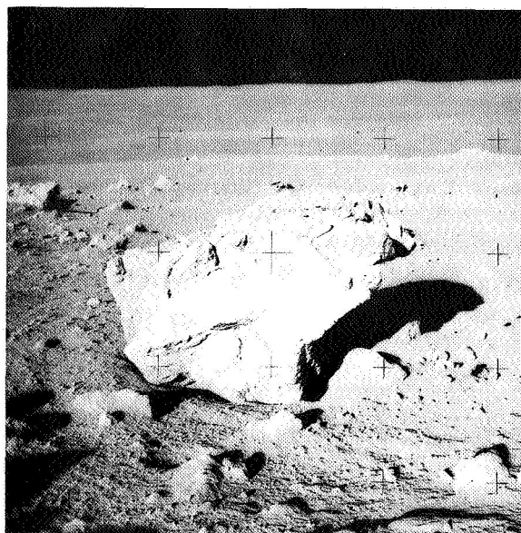
FIGURE 3-21.—Closeup view of fillet on Contact Rock.
