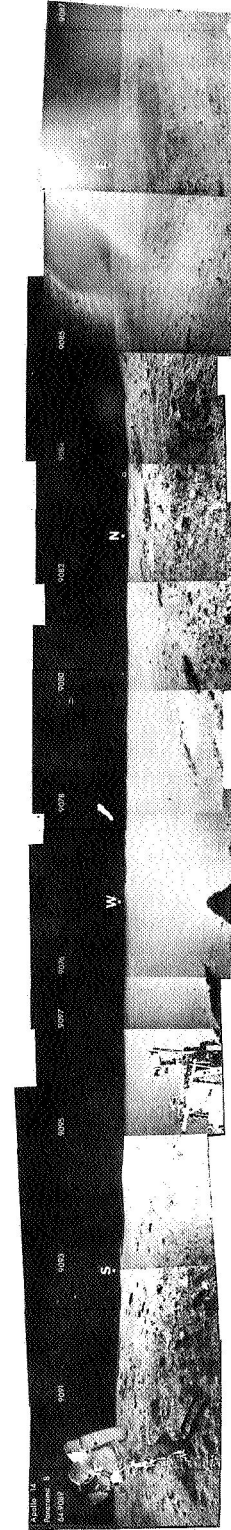
FIGURE 3-5.—Panorama 8, taken at station B1.
