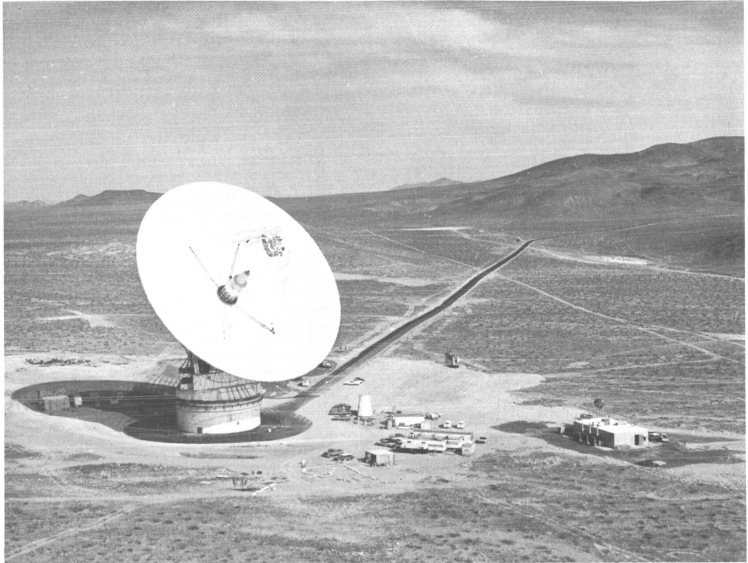
FIGURE 2-3. — The 64-m (210-ft) antenna at the Goldstone, Calif., tracking station. This is the most sensitive communications antenna in the world and has the capability of communicating with a spacecraft at the edge of the solar system.
