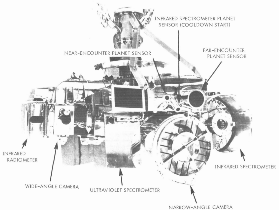
FIGURE 4-1.—Relative positions of scientific instruments carried on Mariners 6 and 7.
