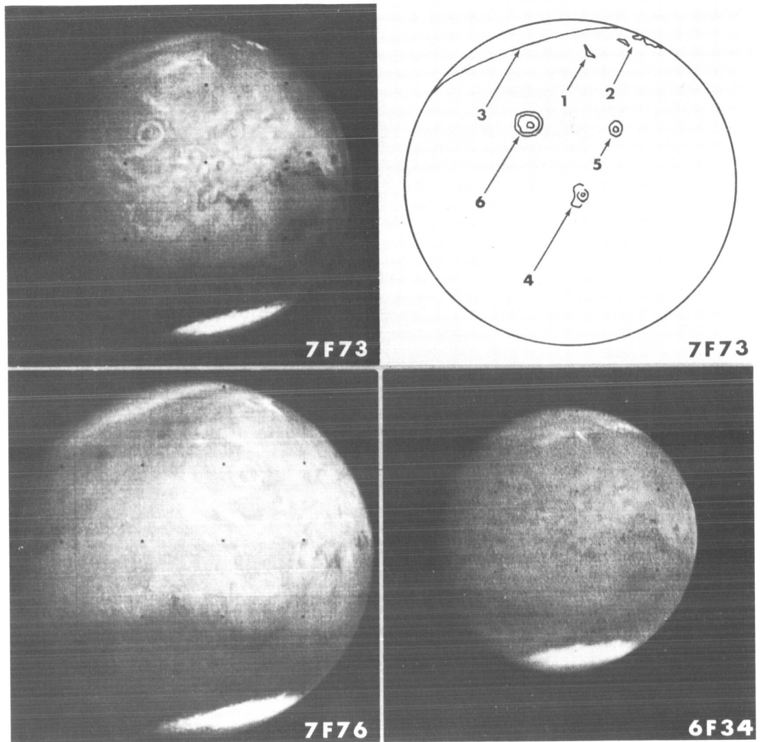
FIGURE 5-8. — FE pictures showing atmospheric and atmosphere/surface effects. Picture times were: 6F34, July 30, 07:32 G.m.t.; 7F73, August 4, 11:15 G.m.t.; and 7F76, August 4, 13:36 G.m.t.
