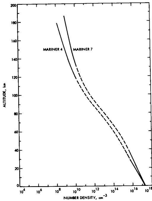
FIGURE 9-12.—Number density vs altitude. The Mariner 4 (1965) data were obtained near 50^\circ S latitude at 13:00 (local time) in late winter. The solar zenith angle was 67^\circ . The Mariner 7 (1969) data were obtained near 58^\circ S latitude at 14:30 (local time) in early spring. The solar zenith angle was about 56^\circ .
