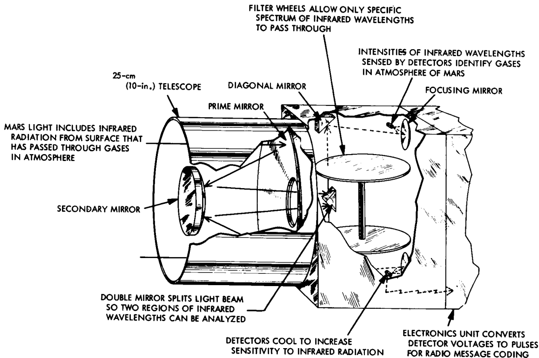
FIGURE 4-2.—Diagram of infrared spectrometer.
