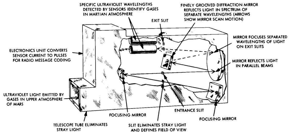
FIGURE 4-3.—Diagram of ultraviolet spectrometer.
