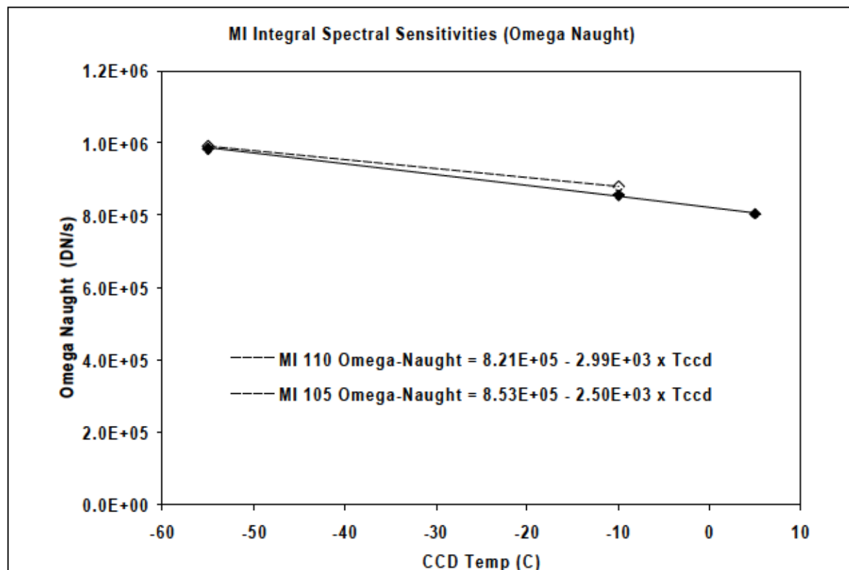
Figure 3.2.2f. Dependence of \bullet_0 on CCD temperature ( ^{\circ}\text{C} ) for both MI cameras: \bullet_0 is in units of DN/s and is defined as the expected signal for a 100% diffusely reflecting target at 1 A.U. from the Sun (see text).
