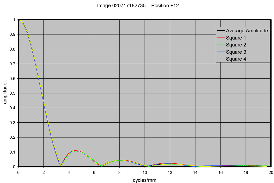
Figure 21.19. MTF curves for image with MI 105 CCD 88 mm from target
