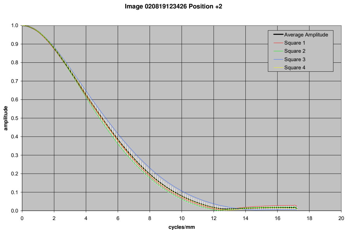
Figure 21.49. MTF curves for image taken with MI 110 CCD 98 mm from the target
