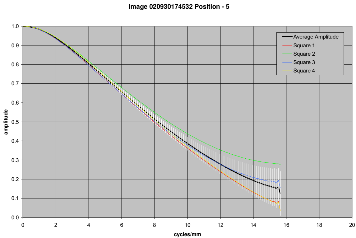
Figure 21.72. MTF curves for image taken with MI 110 CCD 105 mm from the target
