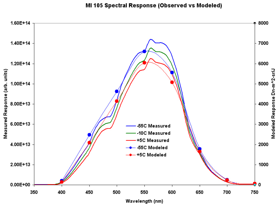
Figure 3.2.2c. MI 105 measured relative spectral response (left ordinate) and modeled absolute spectral response (right ordinate).
