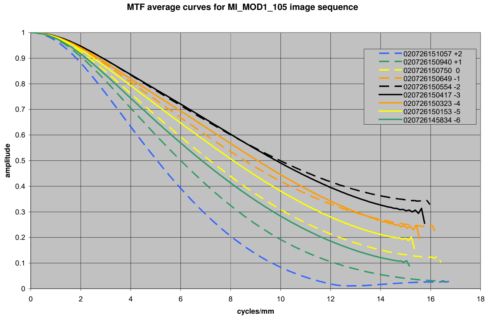
Figure 21.20. MTF average curves for MI_MOD1_105 image sequence. Each curve shows data for positions (in mm) relative to target distance from CCD of 100 mm.
