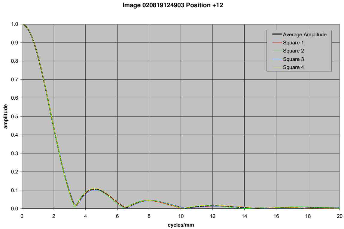
Figure 21.55. MTF curves for image taken with MI 110 CCD 88 mm from the target
