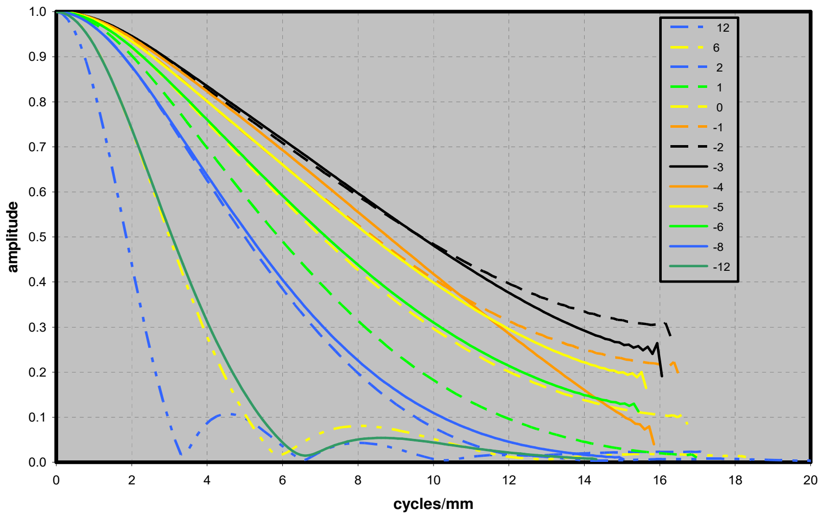
Figure 21.56. MTF average curves for MI_MOD1_110 image sequence. Each curve shows data for positions (in mm) relative to target distance from CCD of 100 mm.
