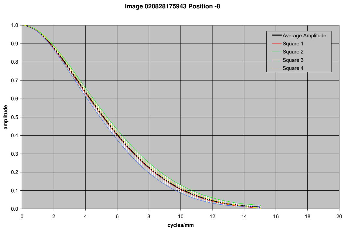
Figure 21.58. MTF curves for image taken with MI 110 CCD 108 mm from the target
