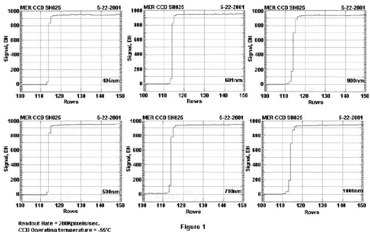
Figure 2.1.1a. Edge response of CCD serial # 25 (not used in flight cameras) at various wavelengths.
