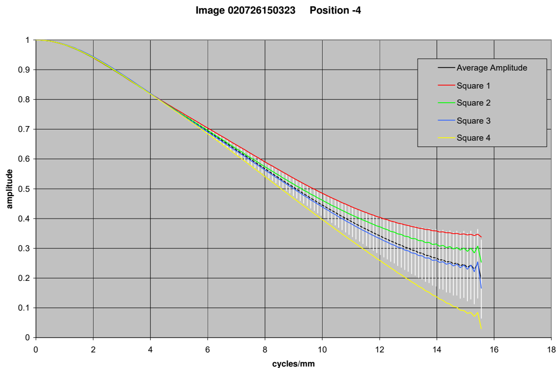
Figure 21.23. MTF curves for image with MI 105 CCD 104 mm from target
