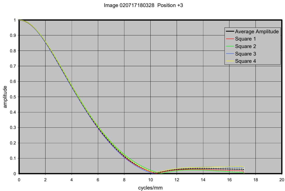
Figure 21.14. MTF curves for image with MI 105 CCD 97 mm from target
