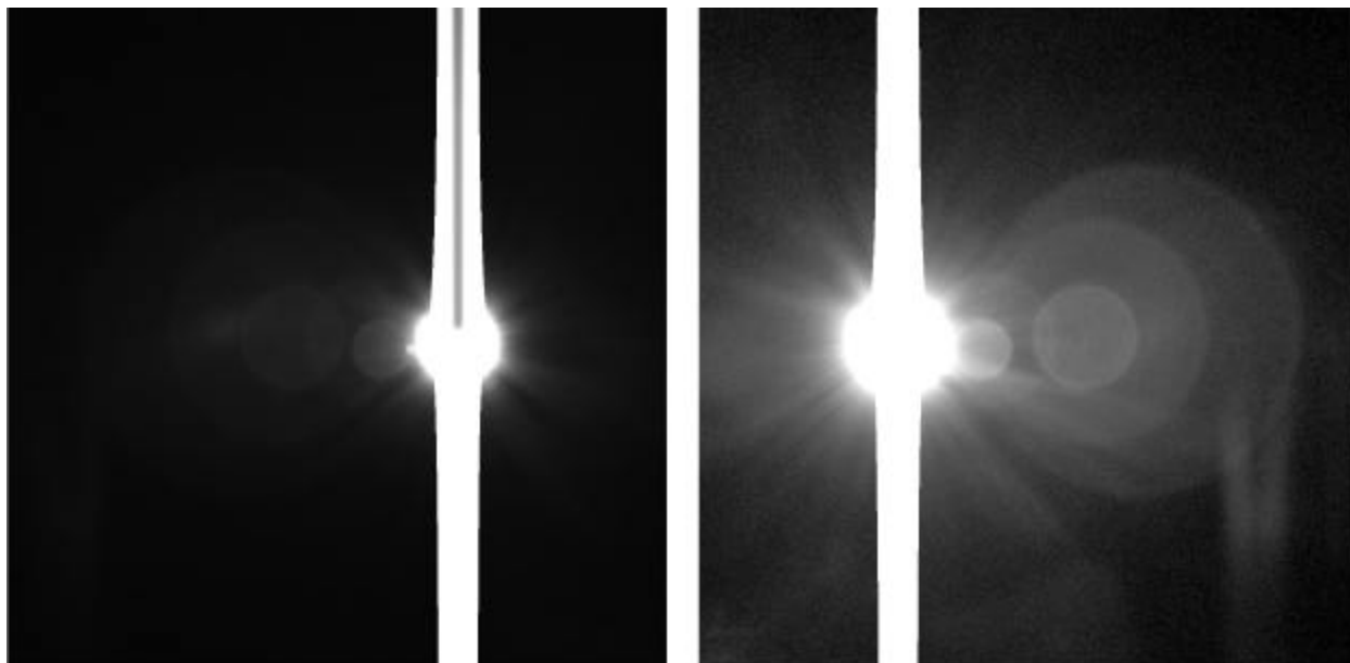
Figure 3.2.9h. Worst-case ghost images in MI serial # 110 images, corrected for transfer smear and stretched hard to show ghosts. (left) Image 020819170945, yaw +4.5°, showing maximum “inner” ghost intensity of ~0.1% just left of saturated source image. (right) Image 020819174157, yaw -4.9, contrast enhanced to show more subtle “outer” ghosts.
