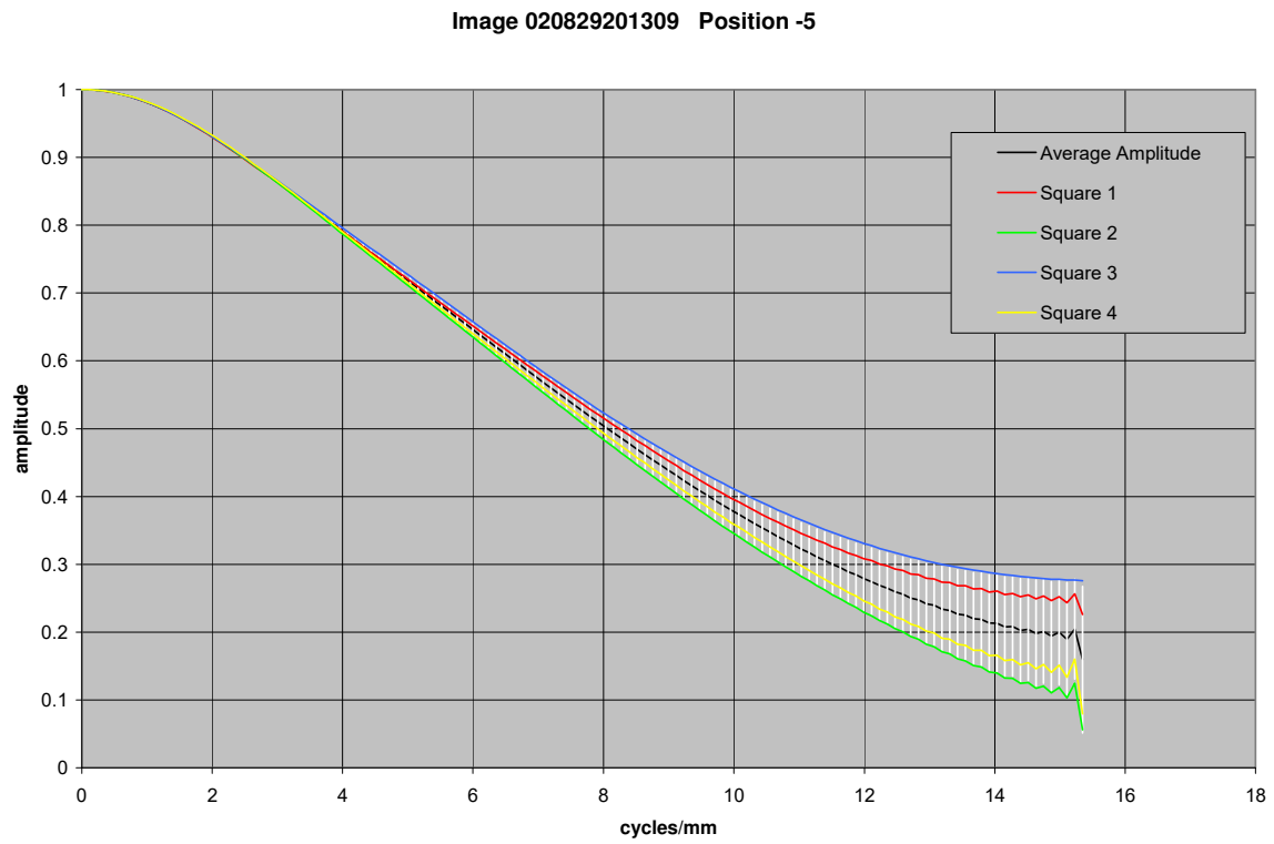
Figure 21.31. MTF curves for image with MI 105 CCD 105 mm from target
