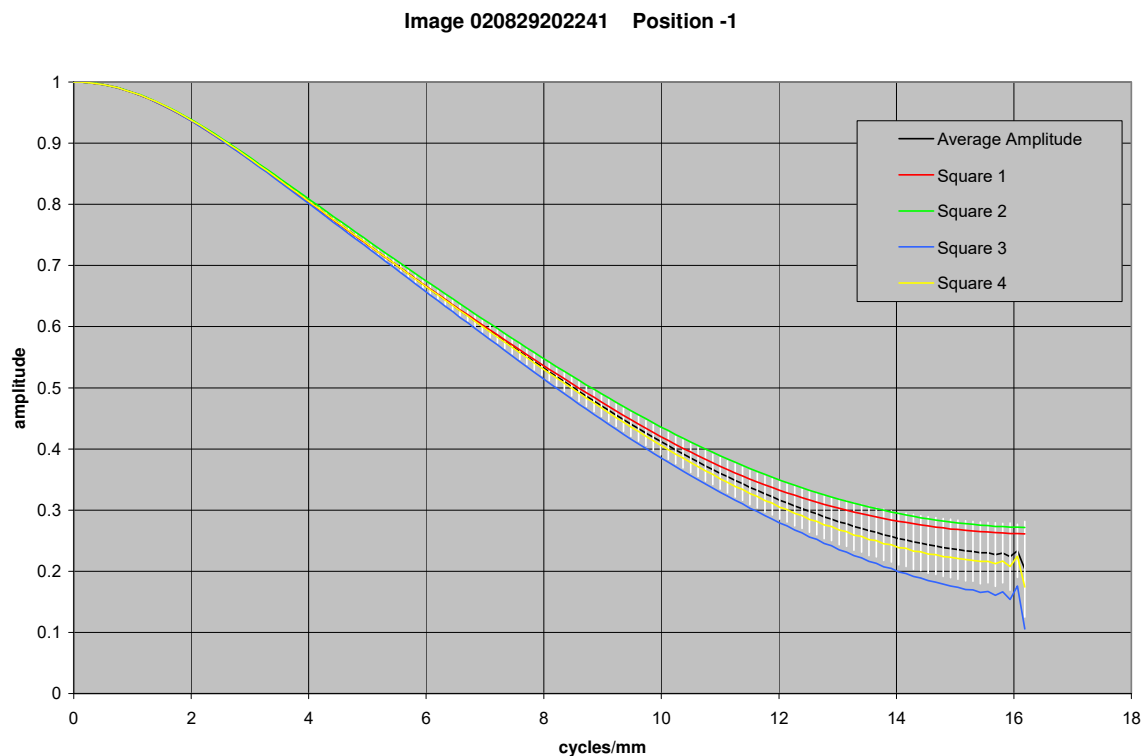
Figure 21.35. MTF curves for image with MI 105 CCD 101 mm from target
