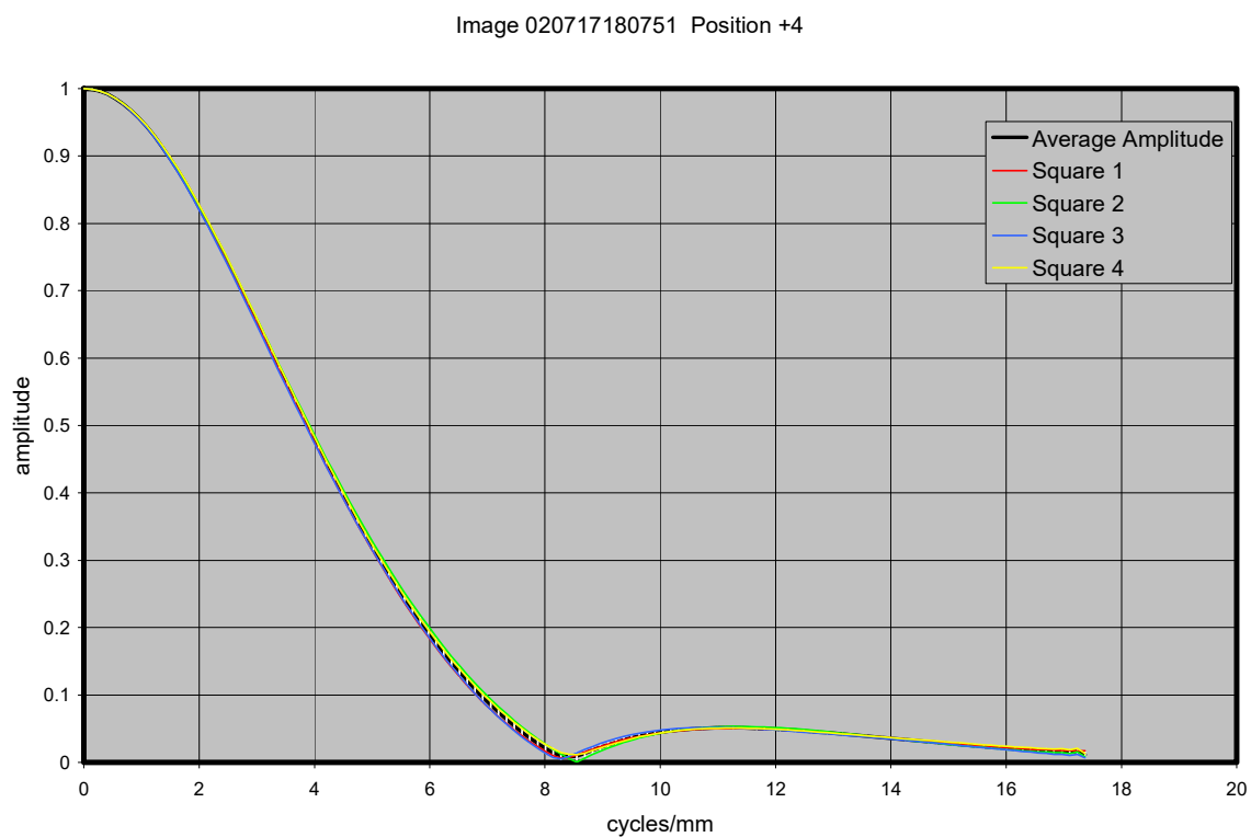
Figure 21.15. MTF curves for image with MI 105 CCD 96 mm from target
