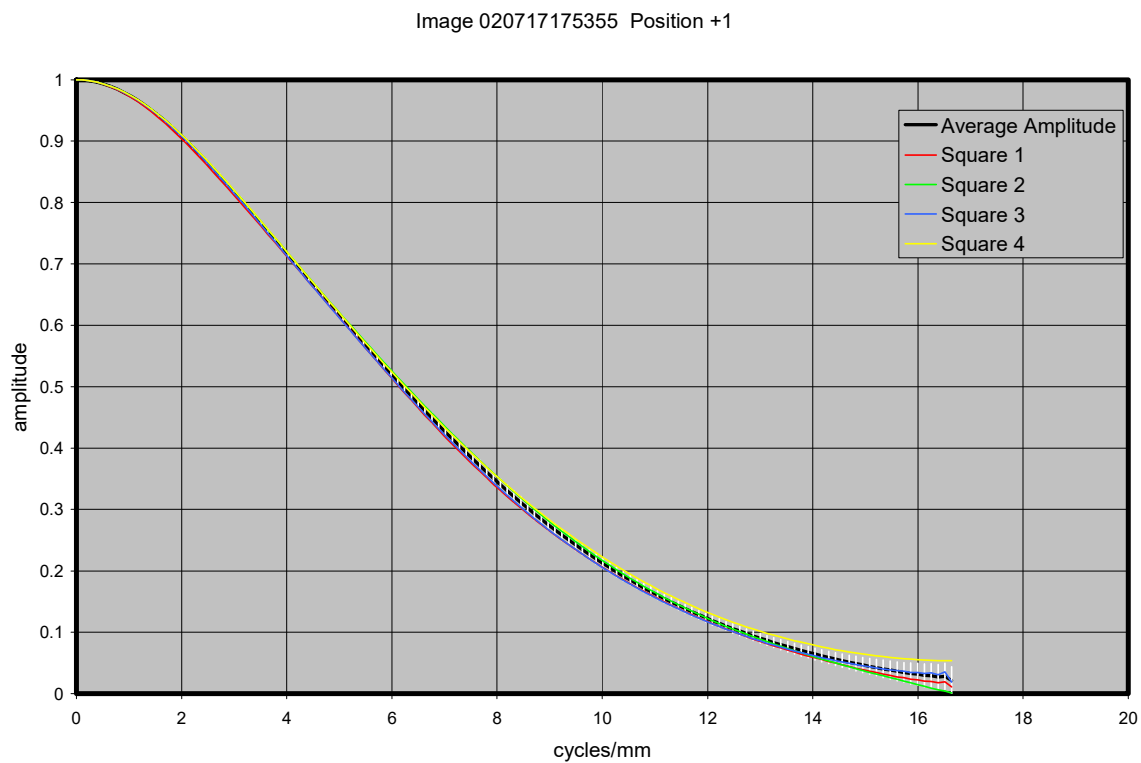
Figure 21.12. MTF curves for image with MI 105 CCD 99 mm from target
