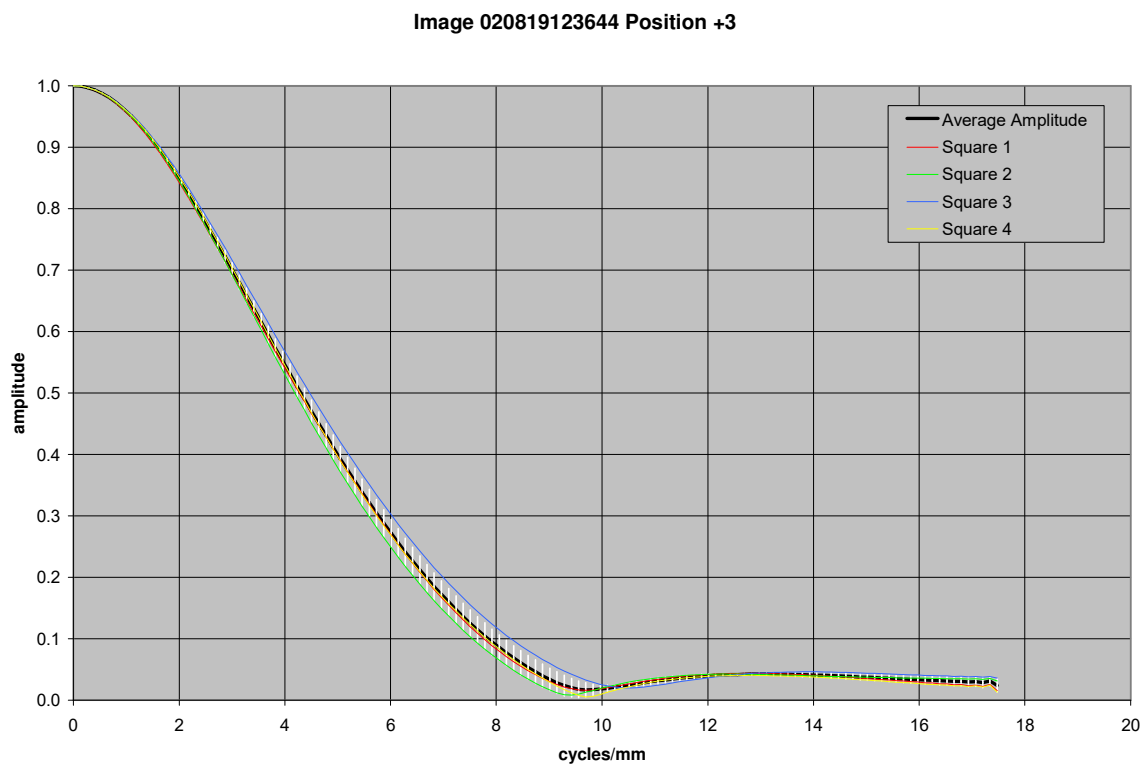
Figure 21.50. MTF curves for image taken with MI 110 CCD 97 mm from the target
