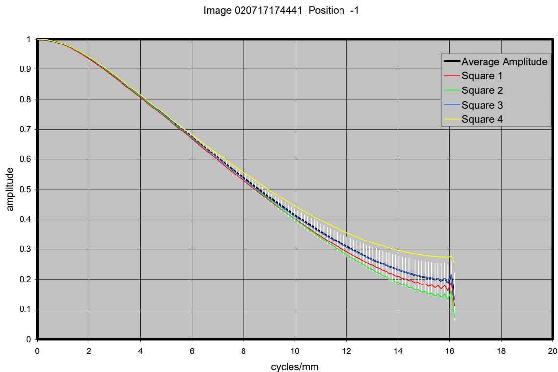
Figure 21.10 MTF curves for image with MI 105 CCD 101 mm from target
