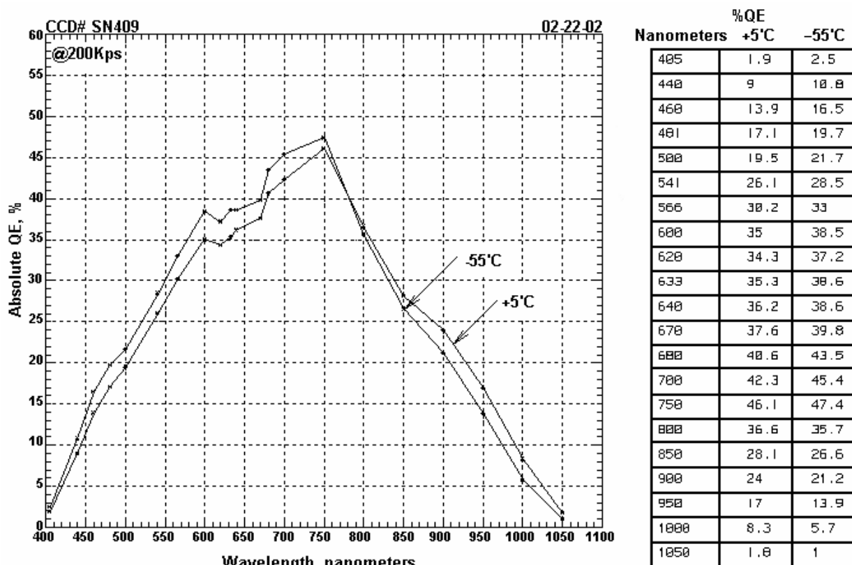
Figure 2.1.8a. Spectral quantum efficiency of CCD serial # 409 (used in MI serial # 105).
