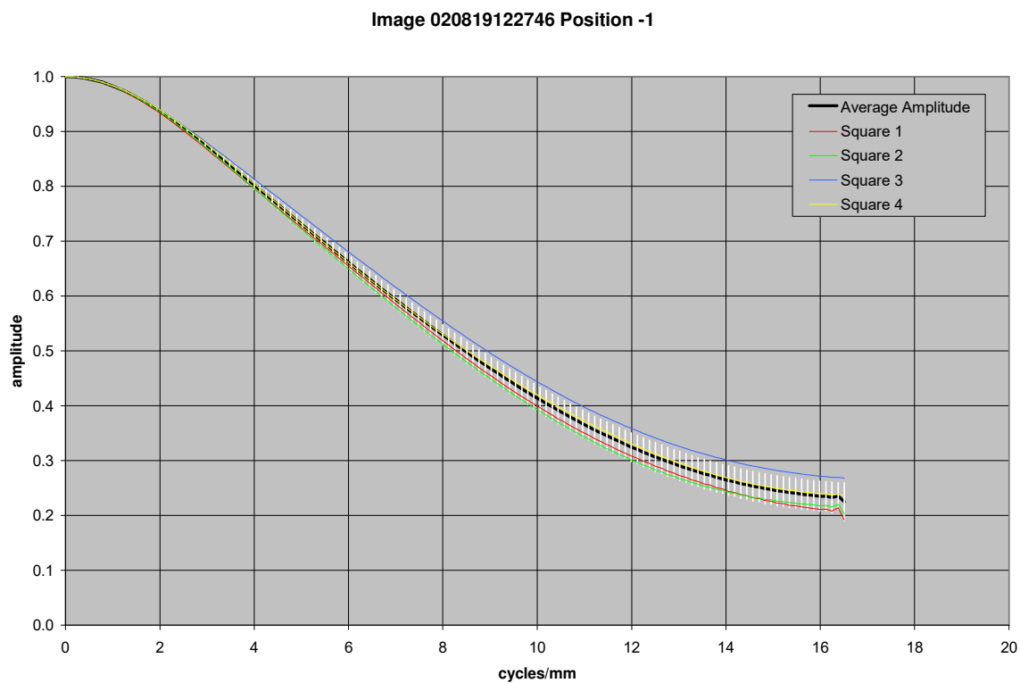
Figure 21.46. MTF curves for image taken with MI 110 CCD 101 mm from the target
