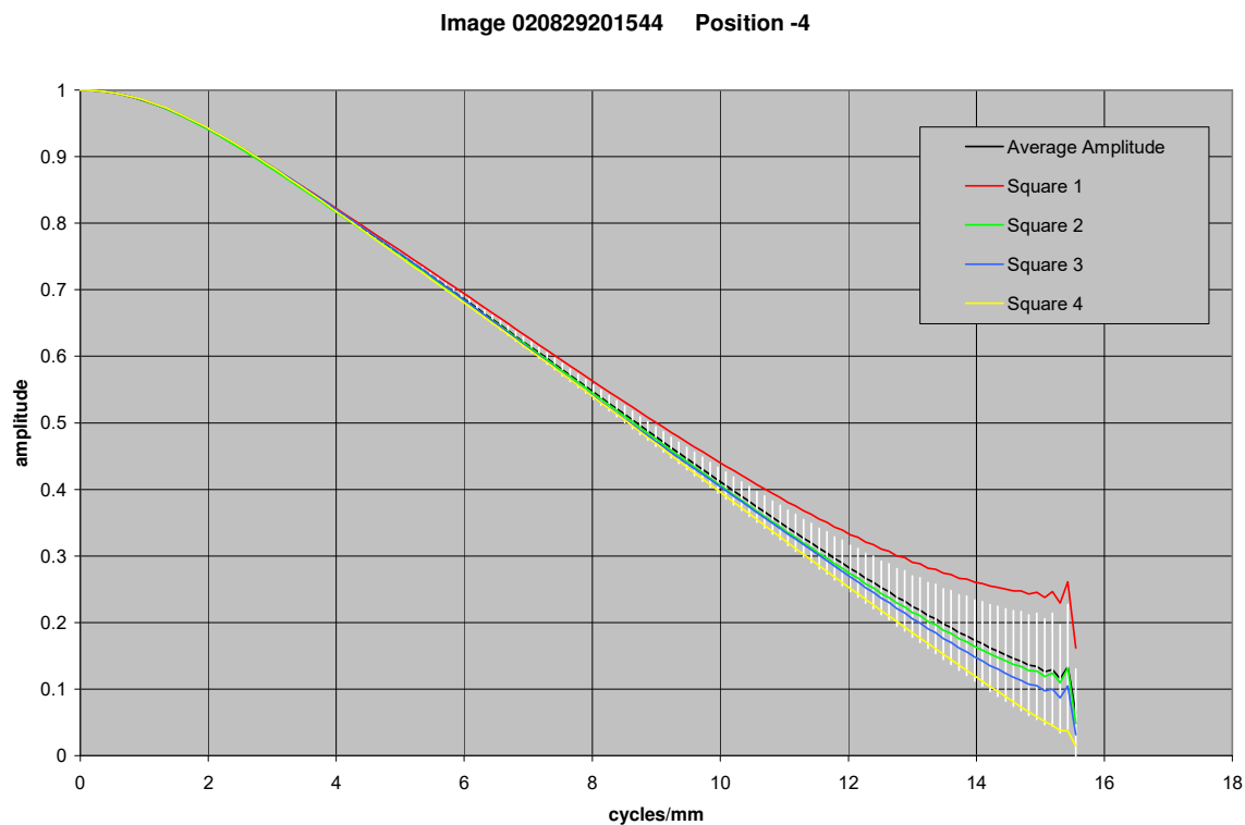
Figure 21.32. MTF curves for image with MI 105 CCD 104 mm from target
