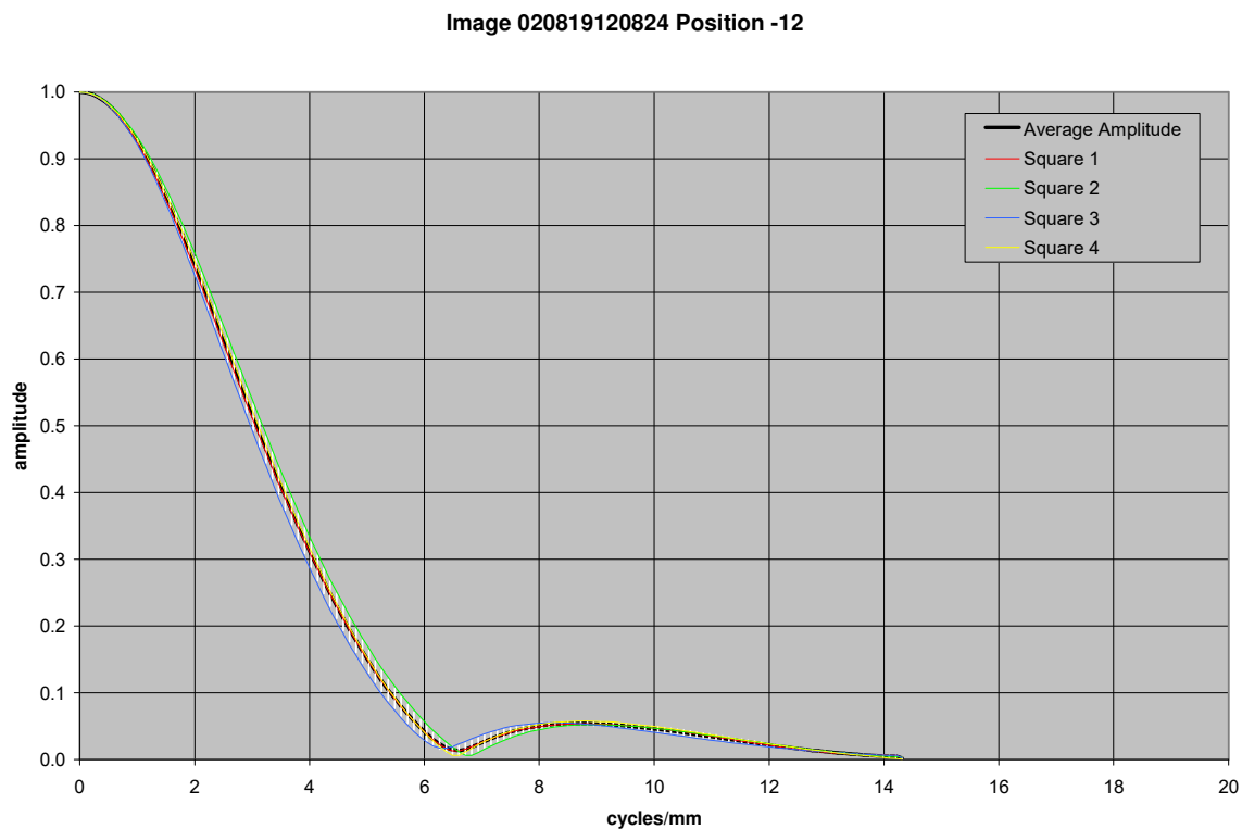
Figure 21.39. MTF curves for image taken with MI 110 CCD 112 mm from target
