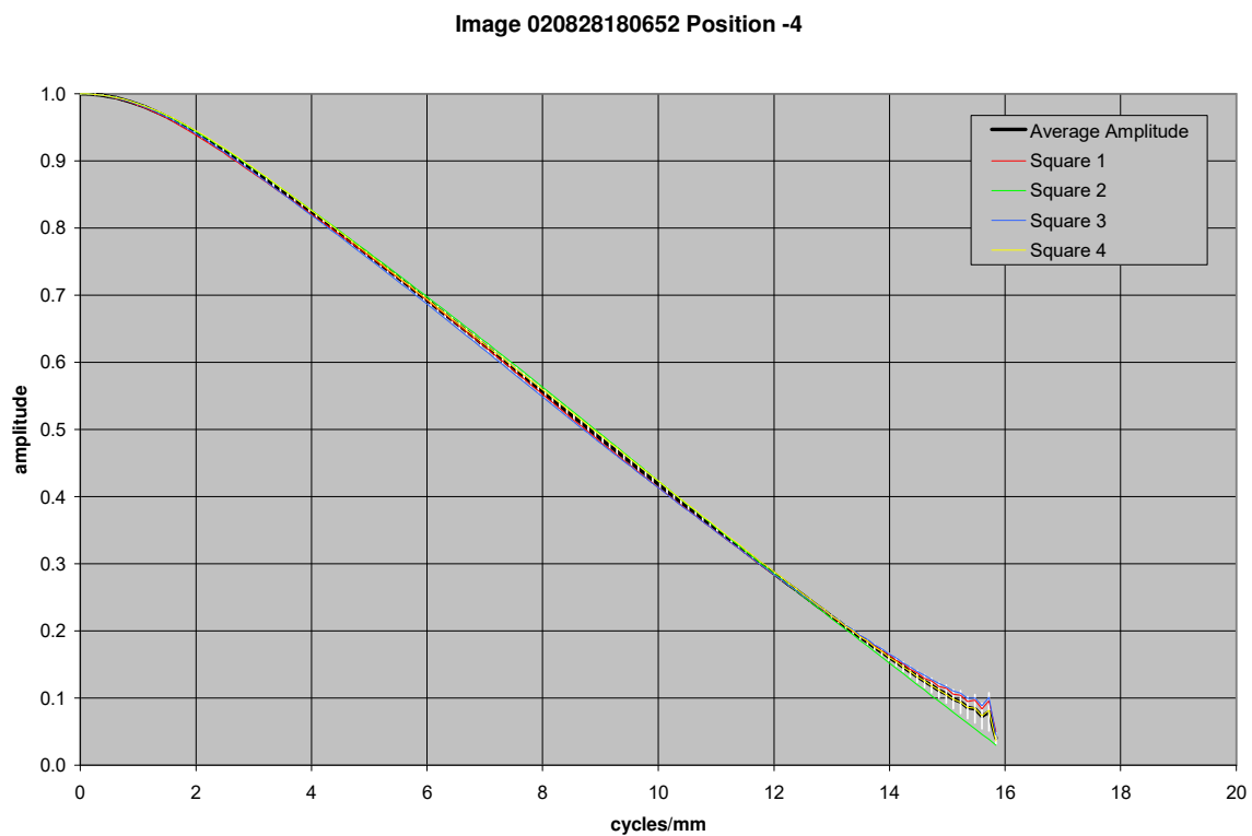
Figure 21.61. MTF curves for image taken with MI 110 CCD 104 mm from the target
