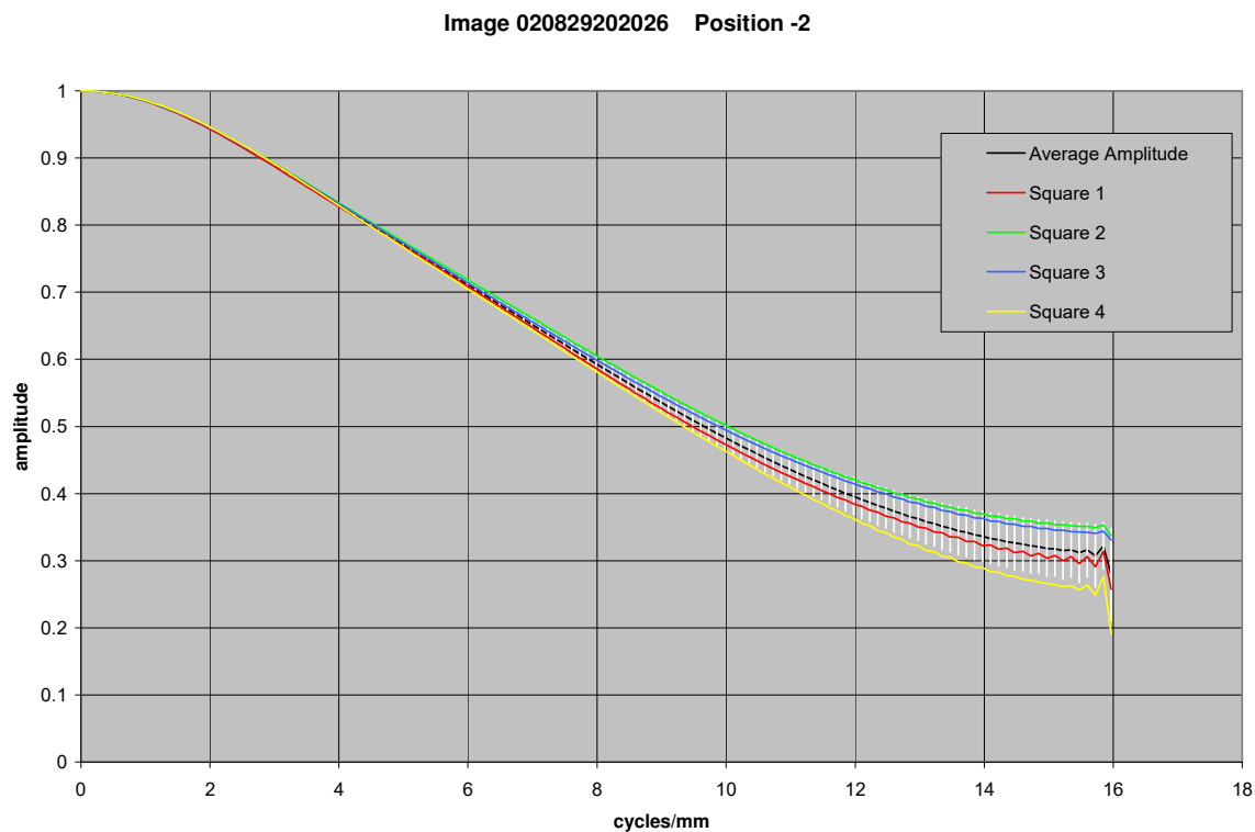
Figure 21.34. MTF curves for image with MI 105 CCD 102 mm from target
