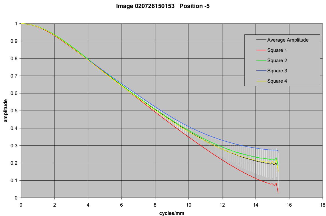
Figure 21.22. MTF curves for image with MI 105 CCD 105 mm from target
