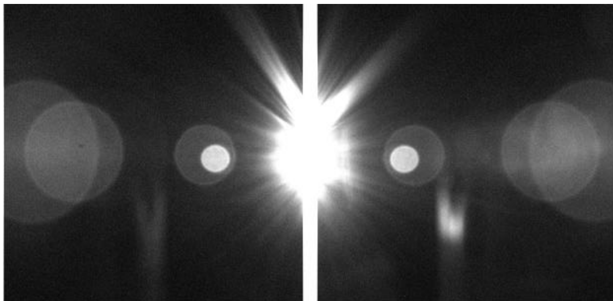
Figure 3.2.9i. Typical ghost images in MI serial # 110 images, corrected for transfer smear and stretched hard to show ghosts. (left) Image 020819171336, yaw +14.5. (right) Image 020819173811, yaw -14.5.
