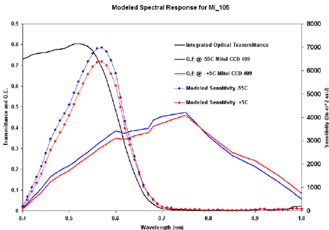
Figure 3.2.2.a. MI 105 response model. In addition to the transmittance and QE curves shown, the following values were used: Gain = 47.9 \text{ e}^-/\text{DN} and A^* = 5.03 \times 10^{13} \text{ m}^2 .
