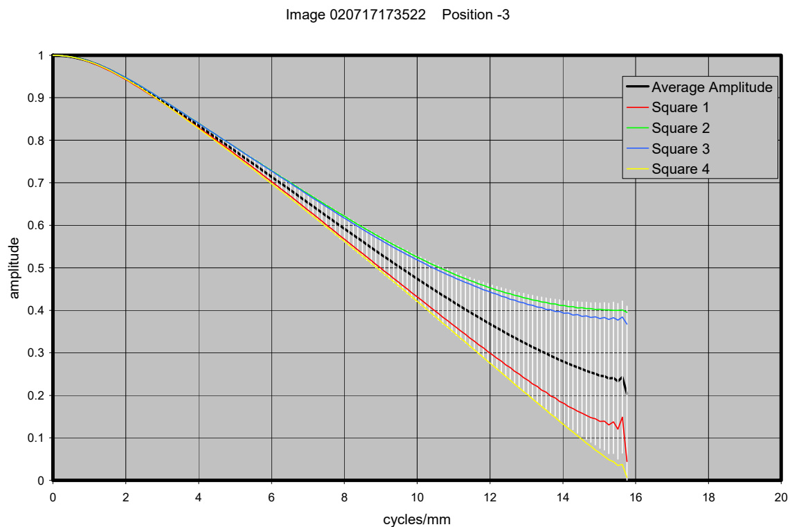
Figure 21.8. MTF curves for image with MI 105 CCD 103 mm from target
