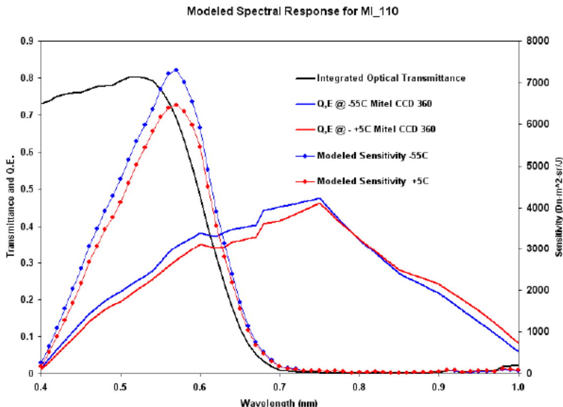
Figure 3.2.2.b. MI 110 response model. In addition to the transmittance and QE curves shown, the following values were used: Gain = 47.1 e - /DN and A* = 5.03 × 10 13 m 2 .
