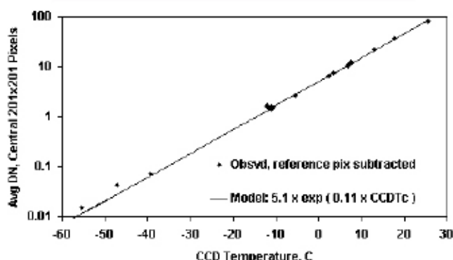
Figure 3.2.1i. Average MI serial # 110 zero-exposure dark current (for central 201x201 pixels) compared with exponential model.
