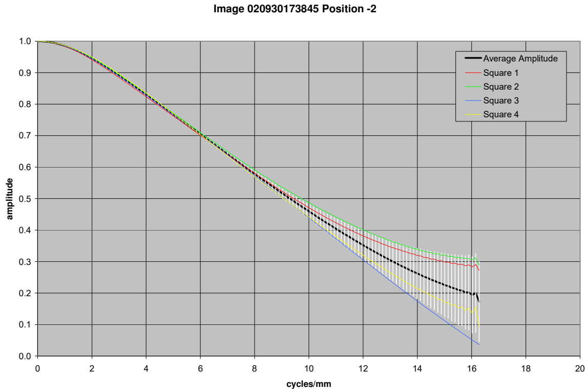
Figure 21.75. MTF curves for image taken with MI 110 CCD 102 mm from the target
