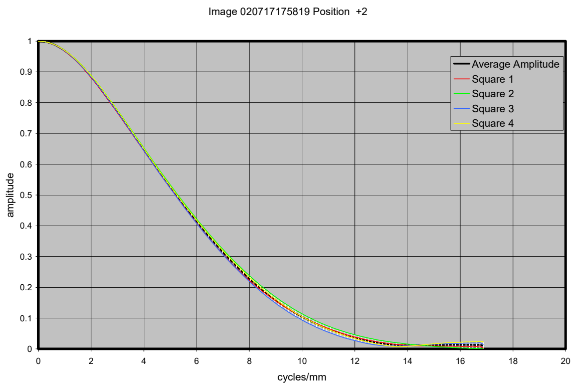
Figure 21.13. MTF curves for image with MI 105 CCD 98 mm from target
