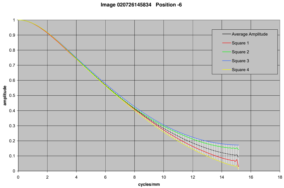
Figure 21.21. MTF curves for image with MI 105 CCD 106 mm from target
