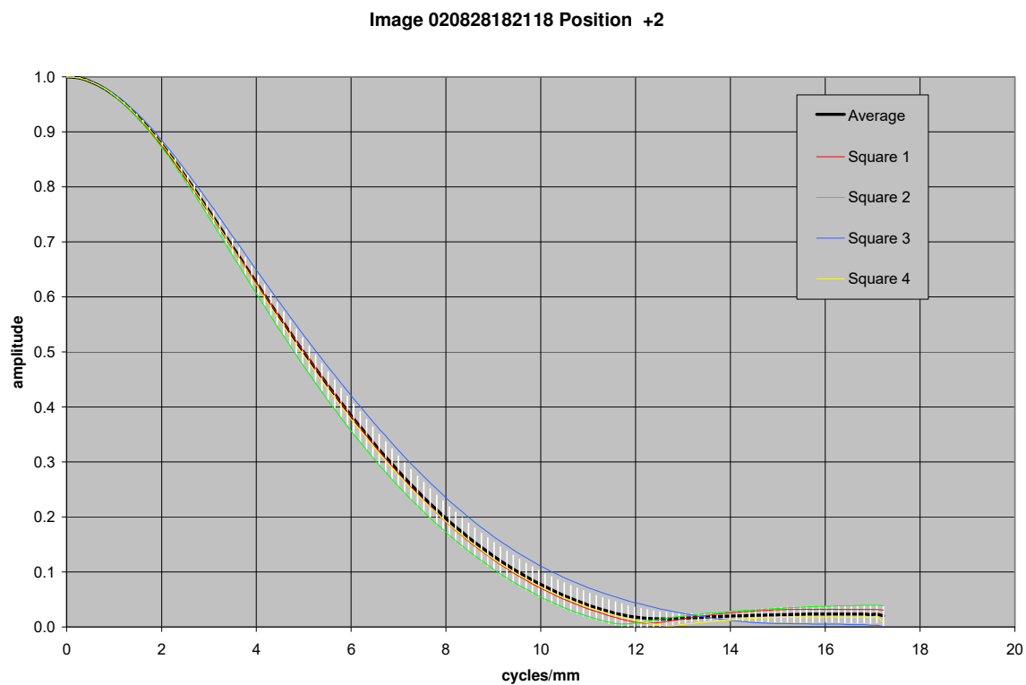
Figure 21.67. MTF curves for image taken with MI 110 CCD 98 mm from the target
