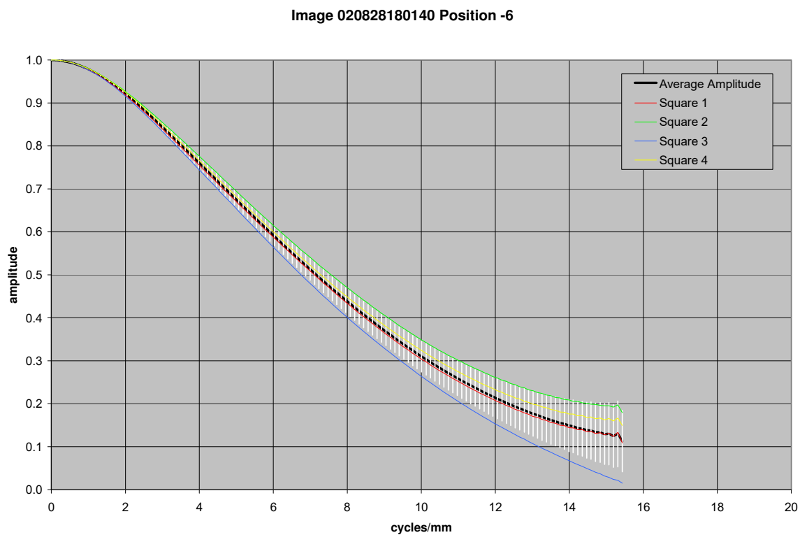
Figure 21.59. MTF curves for image taken with MI 110 CCD 106 mm from the target
