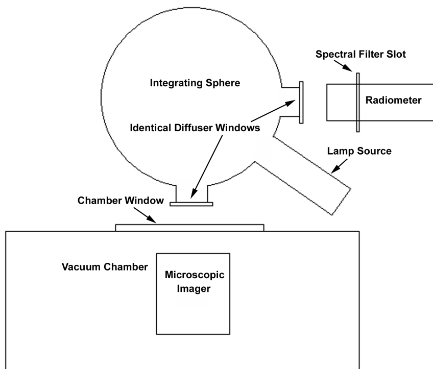
Figure 3.2.2e. Schematic diagram of laboratory setup used to measure absolute response of the integrated MI camera systems.
