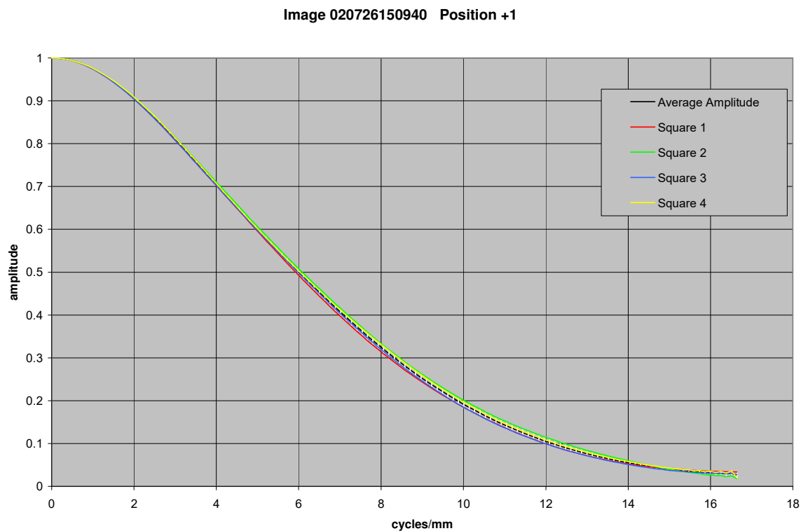
Figure 21.28. MTF curves for image with MI 105 CCD 99 mm from target
