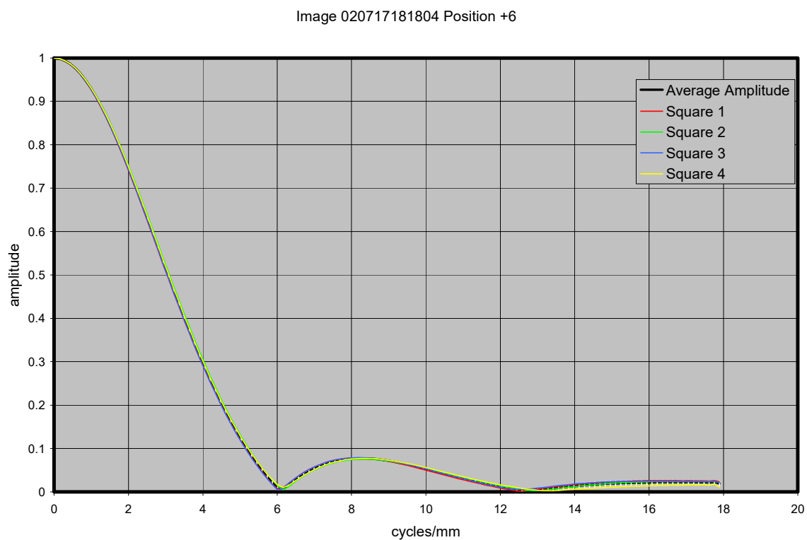
Figure 21.19. MTF curves for image with MI 105 CCD 94 mm from target
