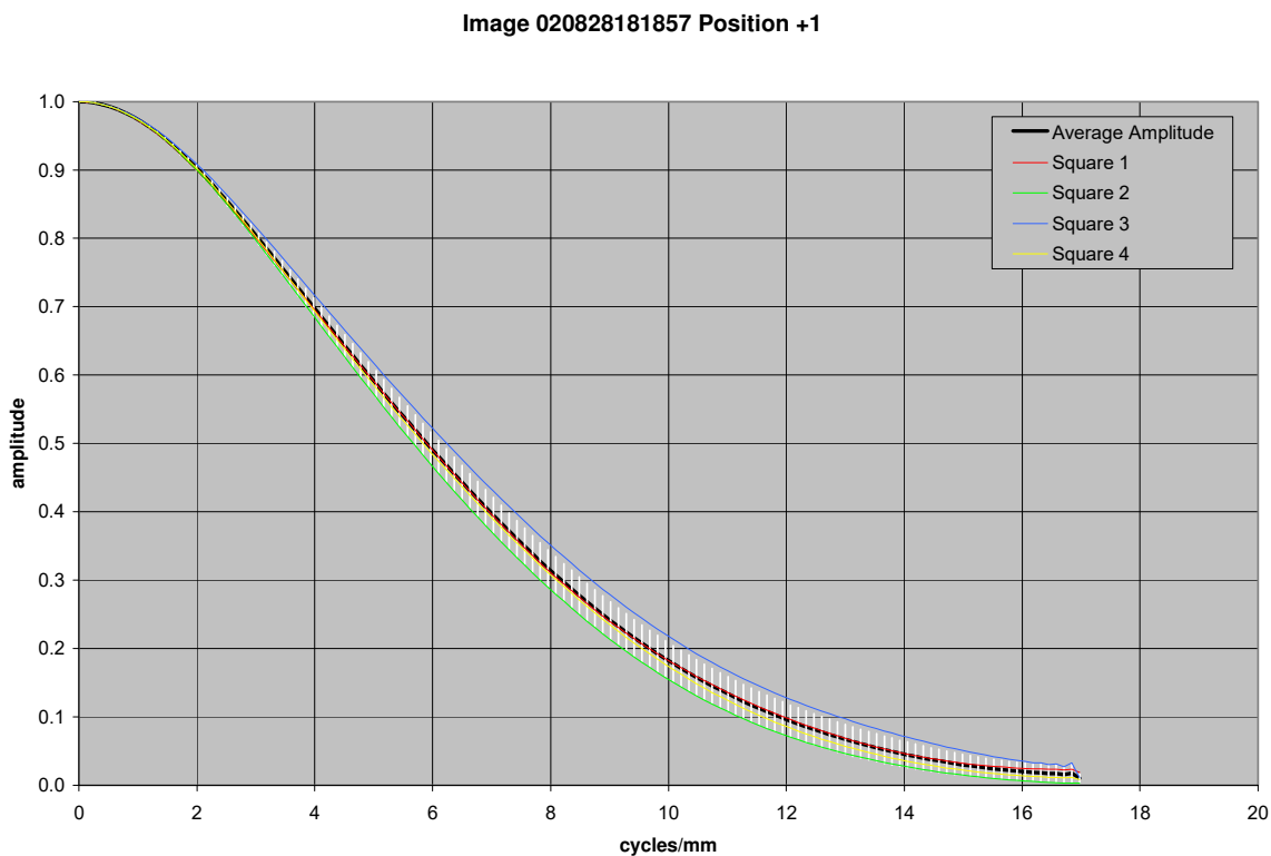
Figure 21.66. MTF curves for image taken with MI 110 CCD 99 mm from the target
