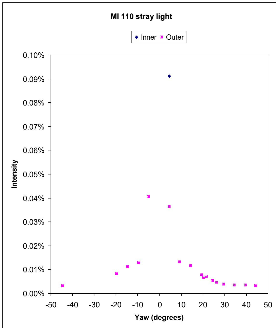
Figure 3.2.9g. Maximum intensity of ghost images in MI serial # 110, relative to intensity of fiber source. The “inner” data point is for the brightest ghost, shown in the left image of Figure 3.2.9h.
