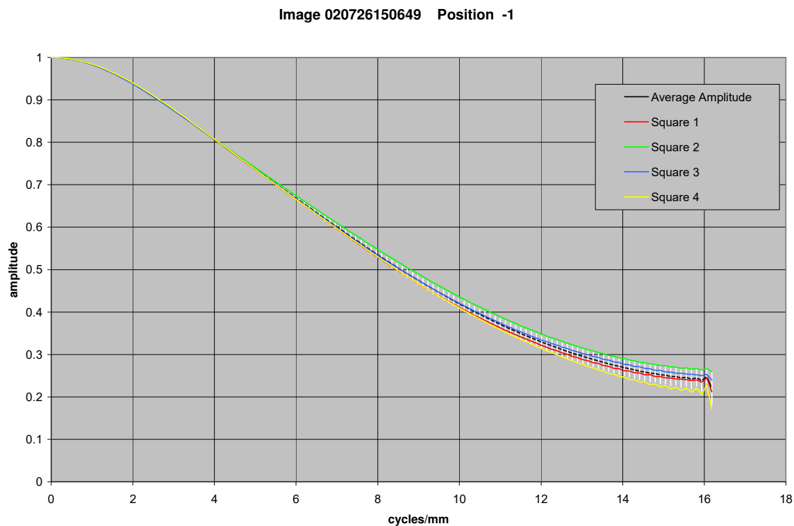
Figure 21.26. MTF curves for image with MI 105 CCD 101 mm from target
