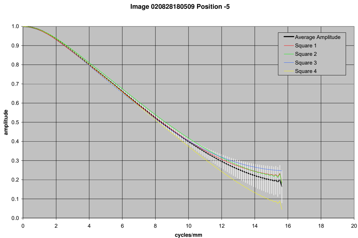
Figure 21.60. MTF curves for image taken with MI 110 CCD 105 mm from the target
