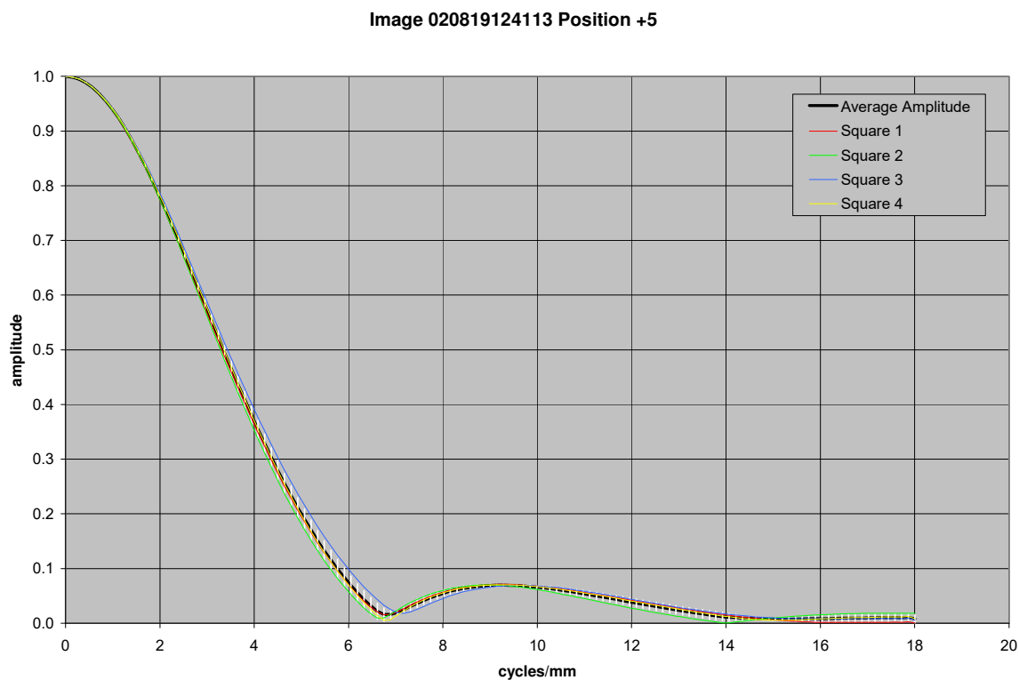
Figure 21.52. MTF curves for image taken with MI 110 CCD 95 mm from the target
