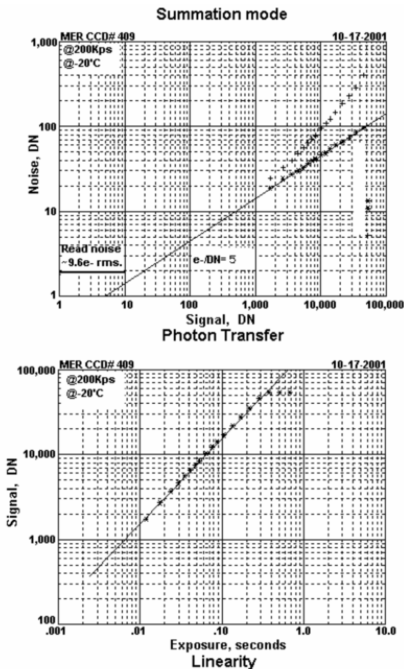
Figure 2.1.4c. CCD serial # 409 (MI serial # 105) summation (4+1) mode. (top) Photon transfer plot with derived parameters. (bottom) Linearity plot.
