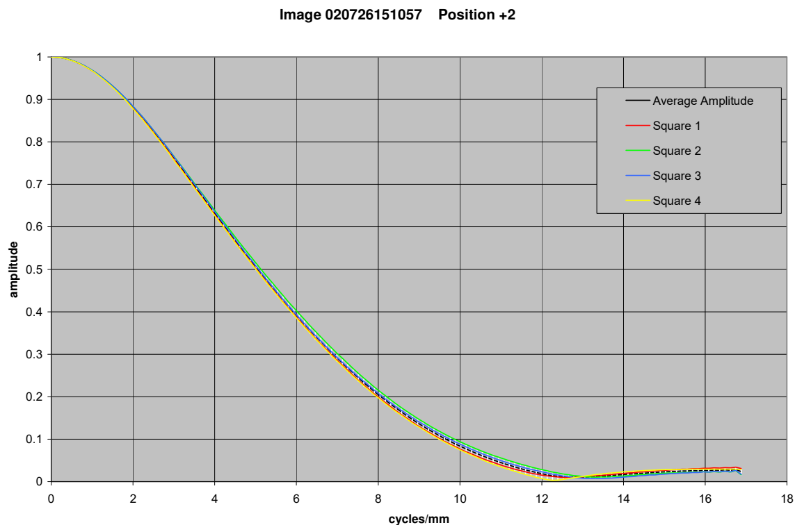
Figure 21.29. MTF curves for image with MI 105 CCD 98 mm from target
