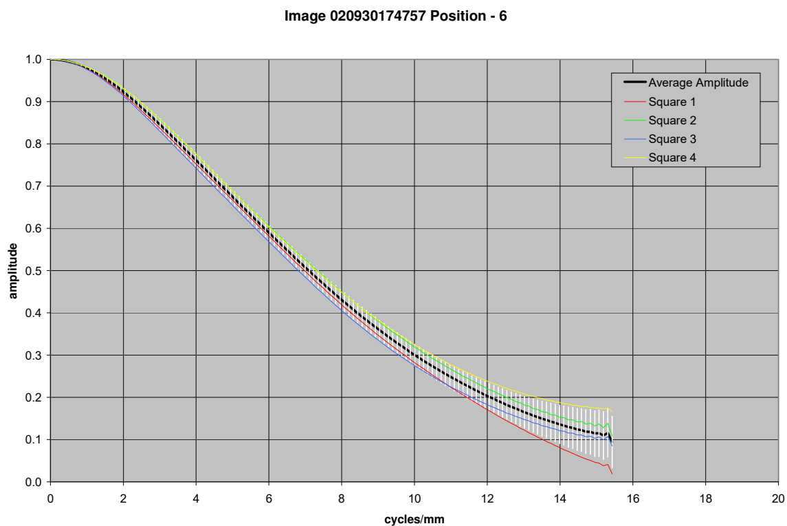
Figure 21.71. MTF curves for an image when the CCD is 106 mm from the target
