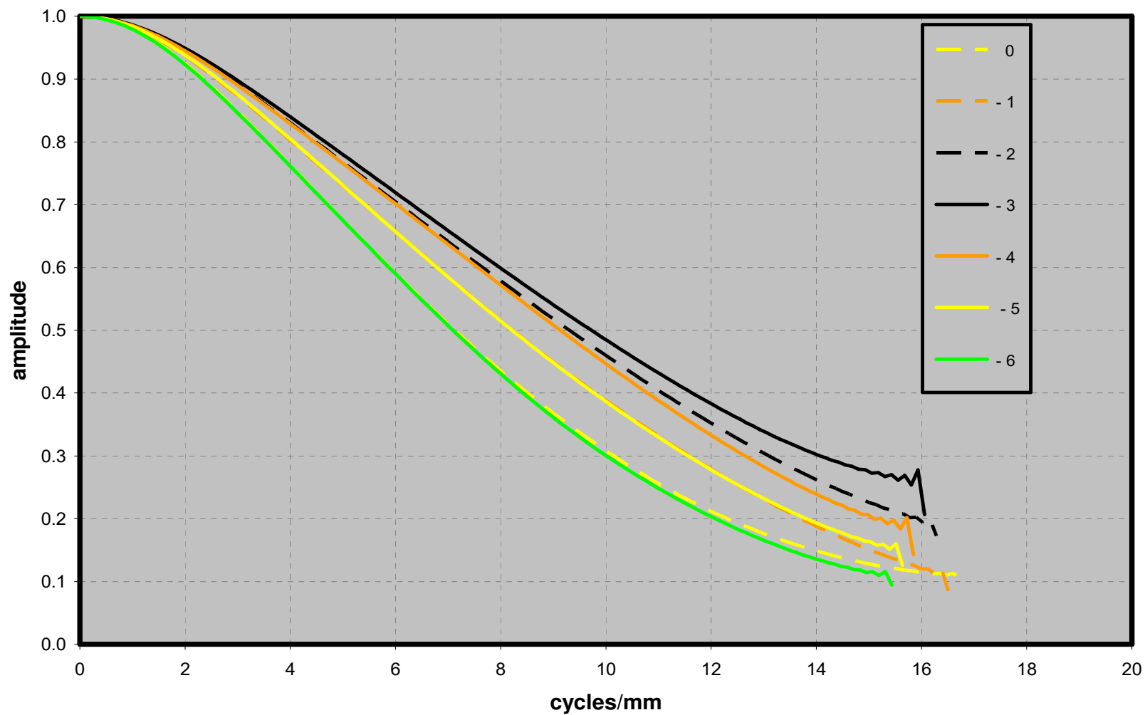
Figure 21.70. MTF average curves for MI_MOD2_110 image sequence. Each curve shows data for positions (in mm) relative to target distance from CCD of 100 mm.
