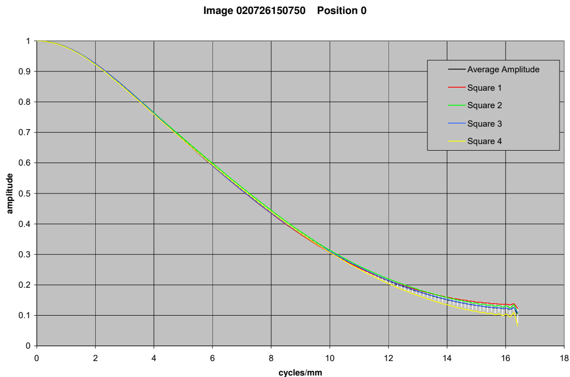
Figure 11.27. MTF curves for image with MI 105 CCD 100 mm from target
