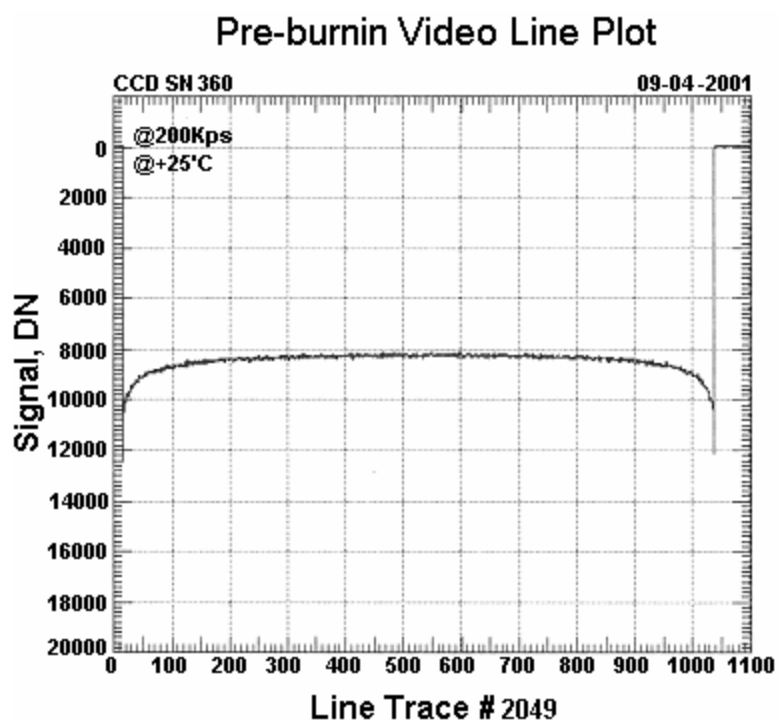
Figure 2.1.3a. Pre-burn-in video line plots for MI flight CCDs at room temperature. (top) CCD serial # 409, used in MI serial # 105. (bottom) CCD serial # 360, used in MI serial # 110.
