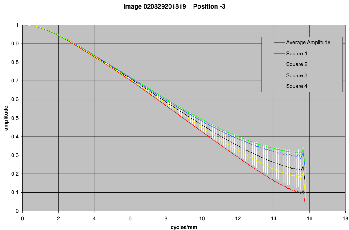
Figure 21.33. MTF curves for image with MI 105 CCD 103 mm from target
