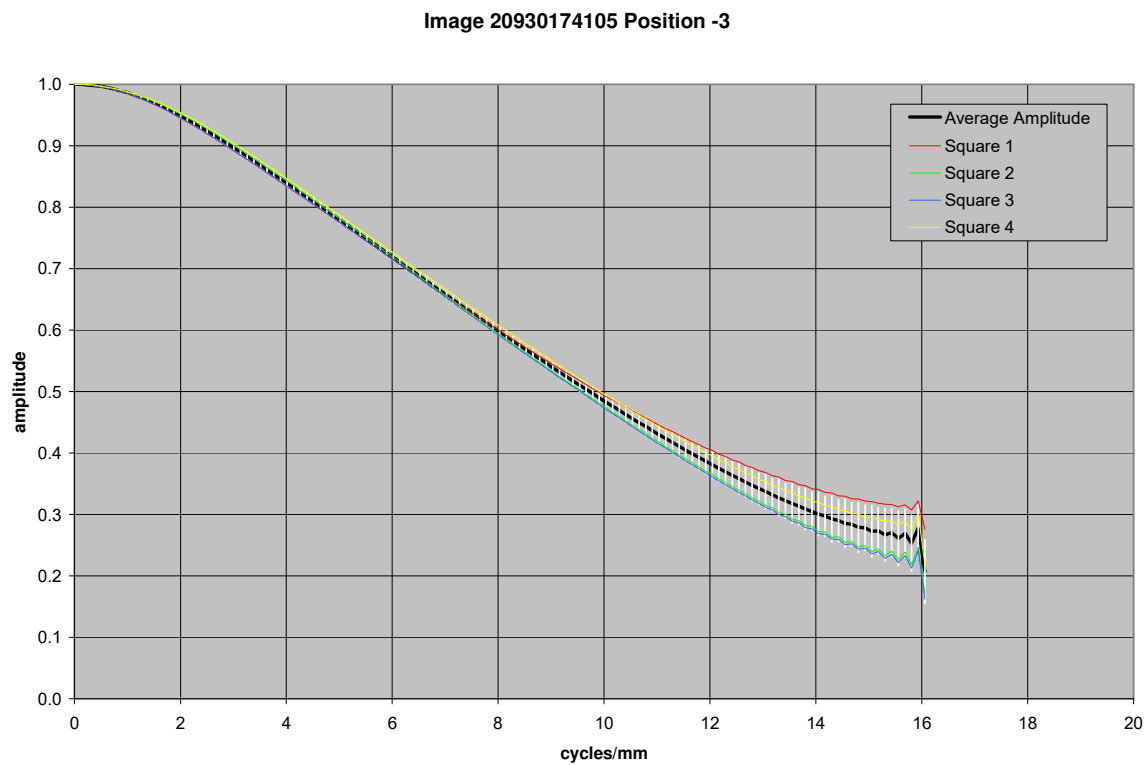
Figure 21.74. MTF curves for image taken with MI 110 CCD 103 mm from the target
