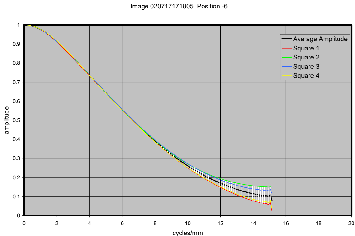
Figure 21.5. MTF curves for image with MI 105 CCD 106 mm from target
