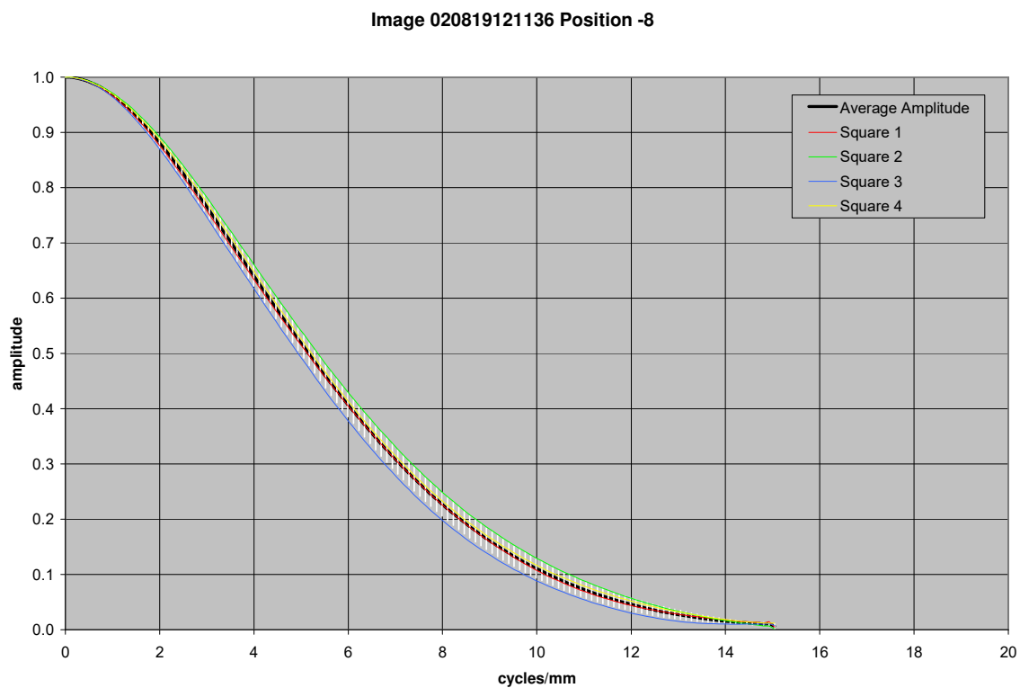
Figure 21.40. MTF curves for image taken with MI 110 CCD 108 mm from the target
