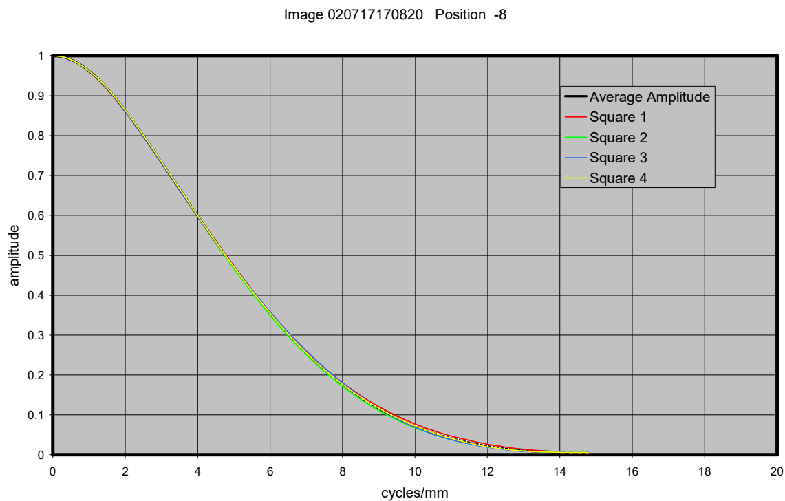
Figure 21.3. MTF curves for image with MI 105 CCD 112 mm from target
