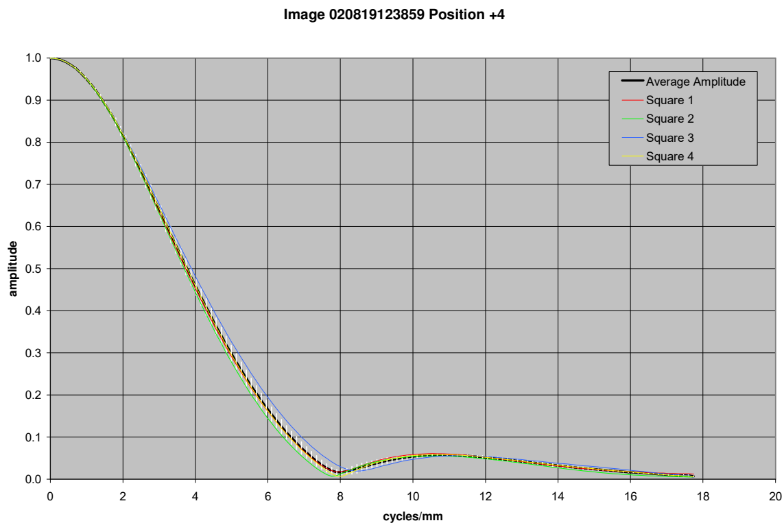
Figure 21.51. MTF curves for image taken with MI 110 CCD 96 mm from the target
