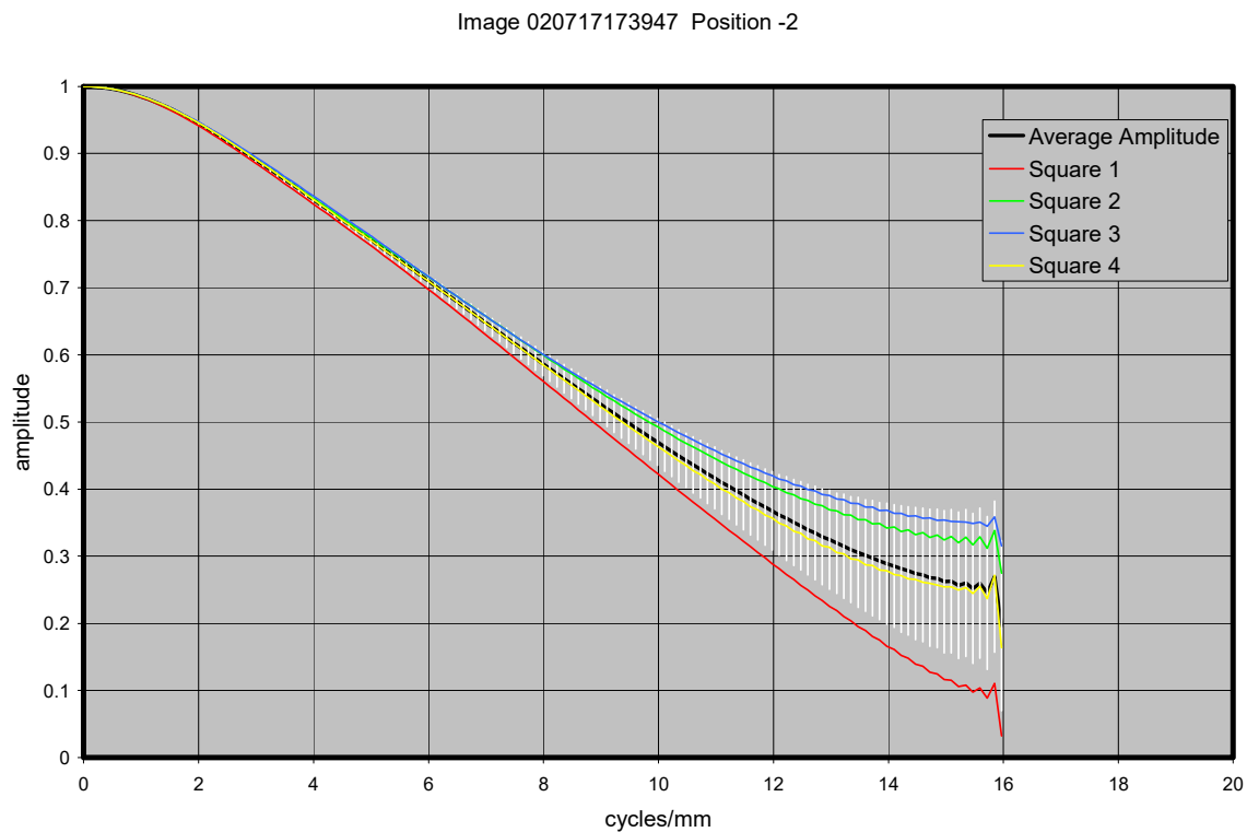
Figure 21.9. MTF curves for image with MI 105 CCD 102 mm from target
