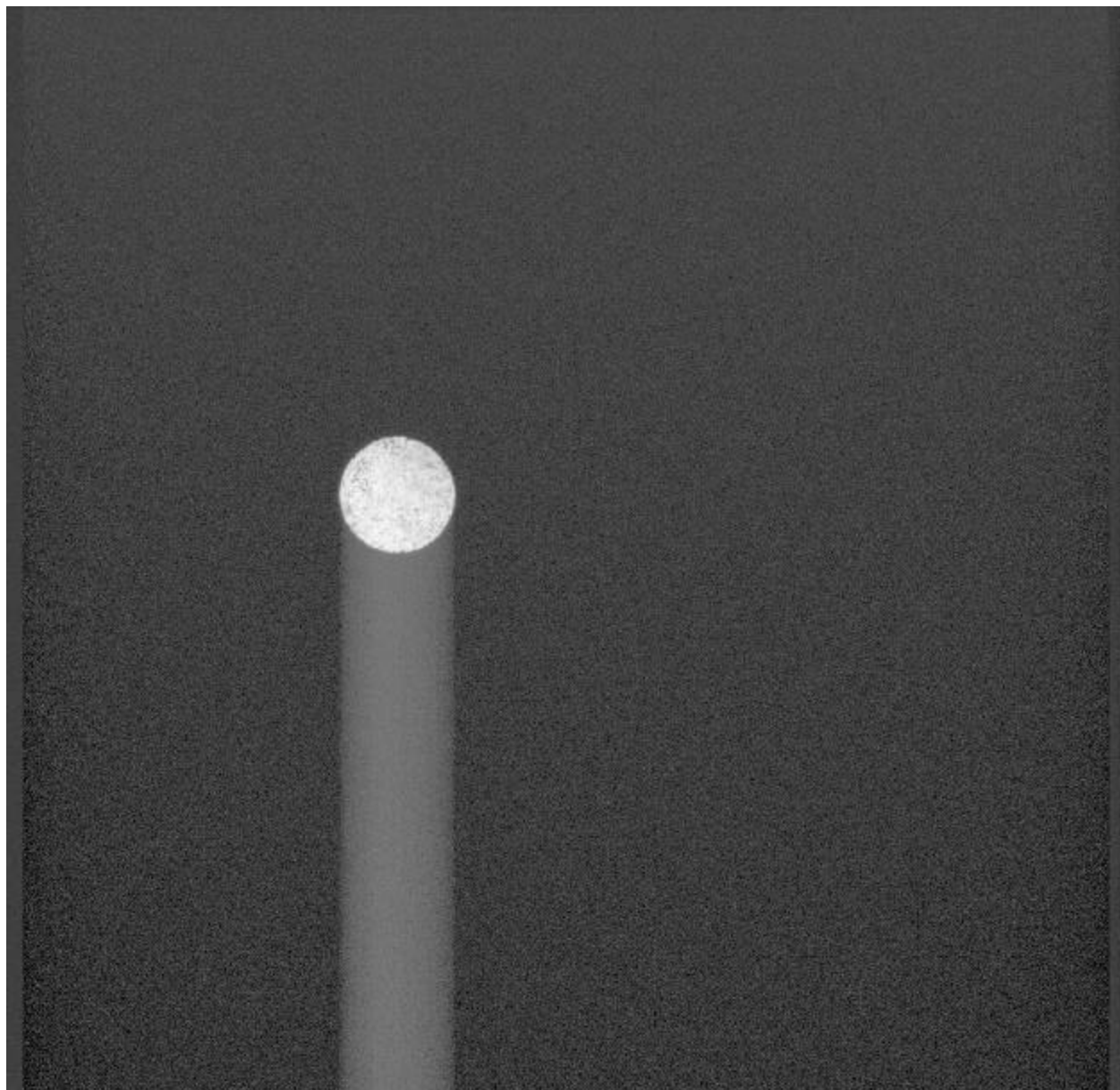
Figure 3.2.6a. MI serial # 105 image of fiber (020718092113_0000102) taken under ambient conditions with exposure time = 10.24 msec. Average zero-second dark frame has been subtracted to remove dark current accumulated during readout. Image transfer direction is toward top; note transfer smear below fiber image.
