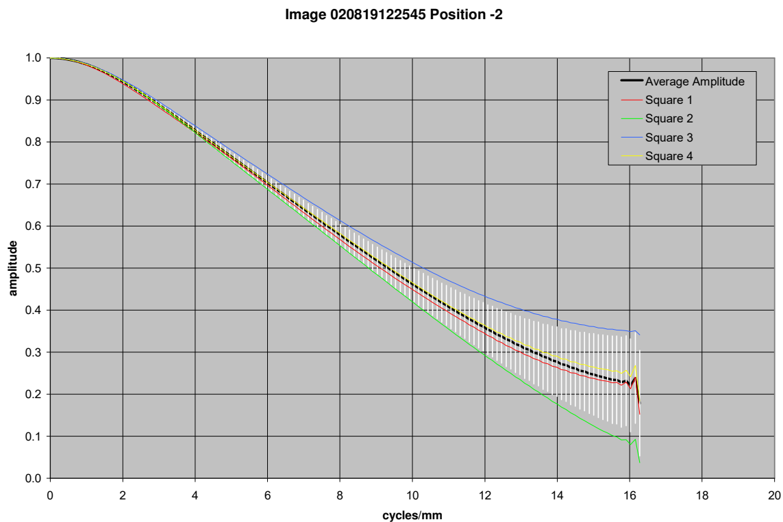
Figure 21.45 MTF curves for image taken with MI 110 CCD 102 mm from the target
