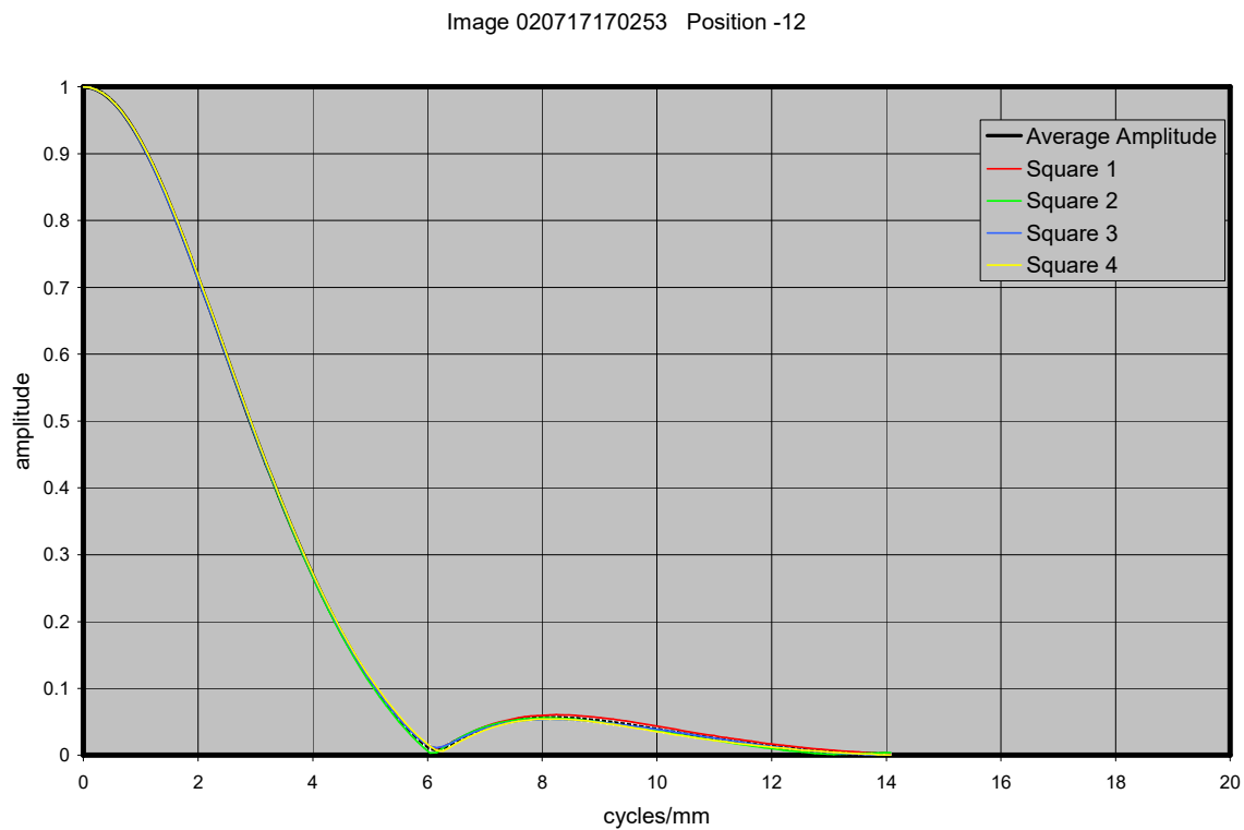
Figure 21.3. MTF curves for image with MI 105 CCD 112 mm from target
