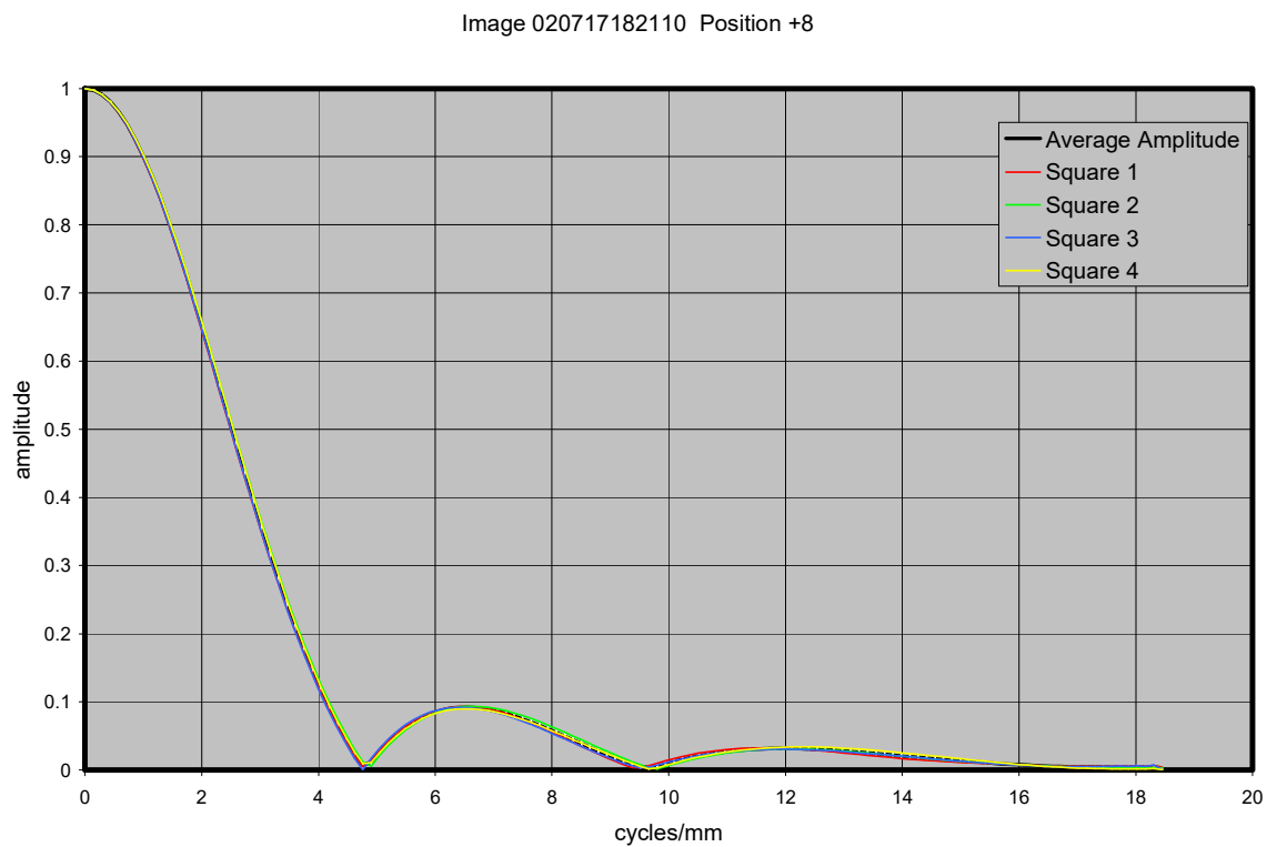
Figure 21.18. MTF curves for image with MI 105 CCD 92 mm from target
