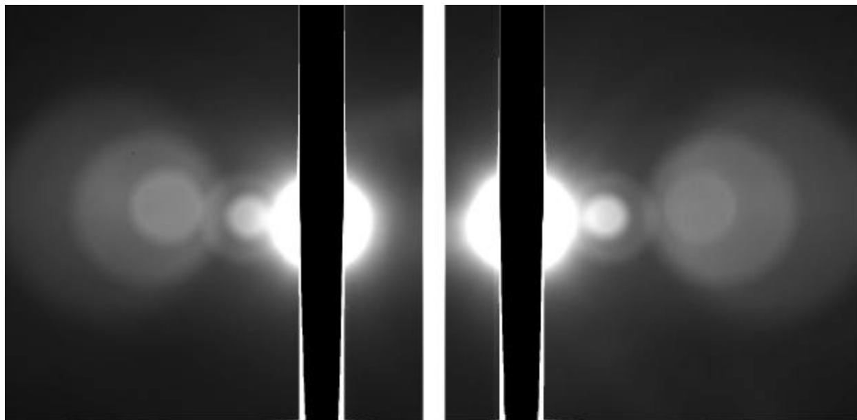
Figure 3.2.9c. Typical ghost images in MI serial # 105 images, corrected for transfer smear and stretched hard to show ghosts. Maximum ghost intensity \sim 0.02\% . (left) Image 020718082943, yaw +6.4^\circ . (right) Image 020718084958, yaw -7.8^\circ .
