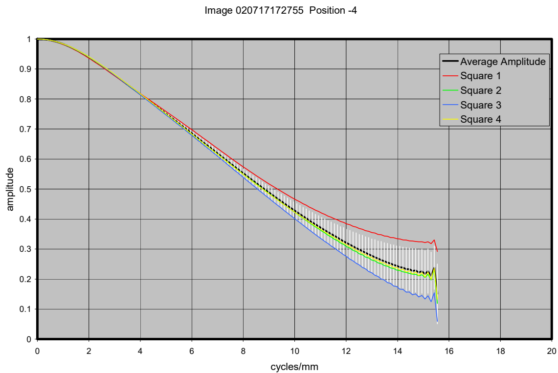
Figure 21.7. MTF curves for image with MI 105 CCD 104 mm from target
