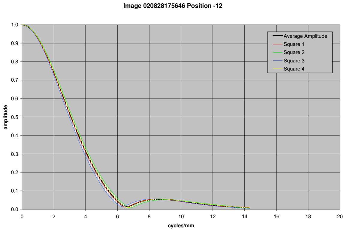
Figure 21.57. MTF curves for image taken with MI 110 CCD 112 mm from the target
