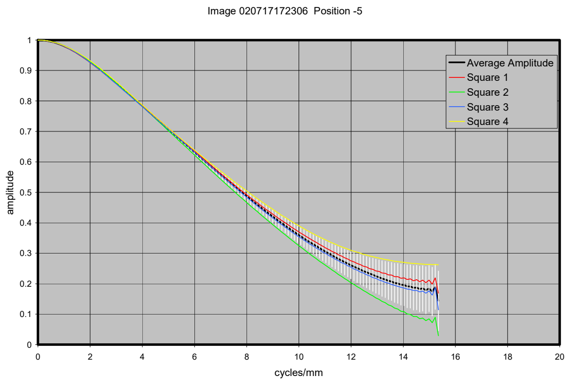
Figure 21.6. MTF curves for image with MI 105 CCD 105 mm from target
