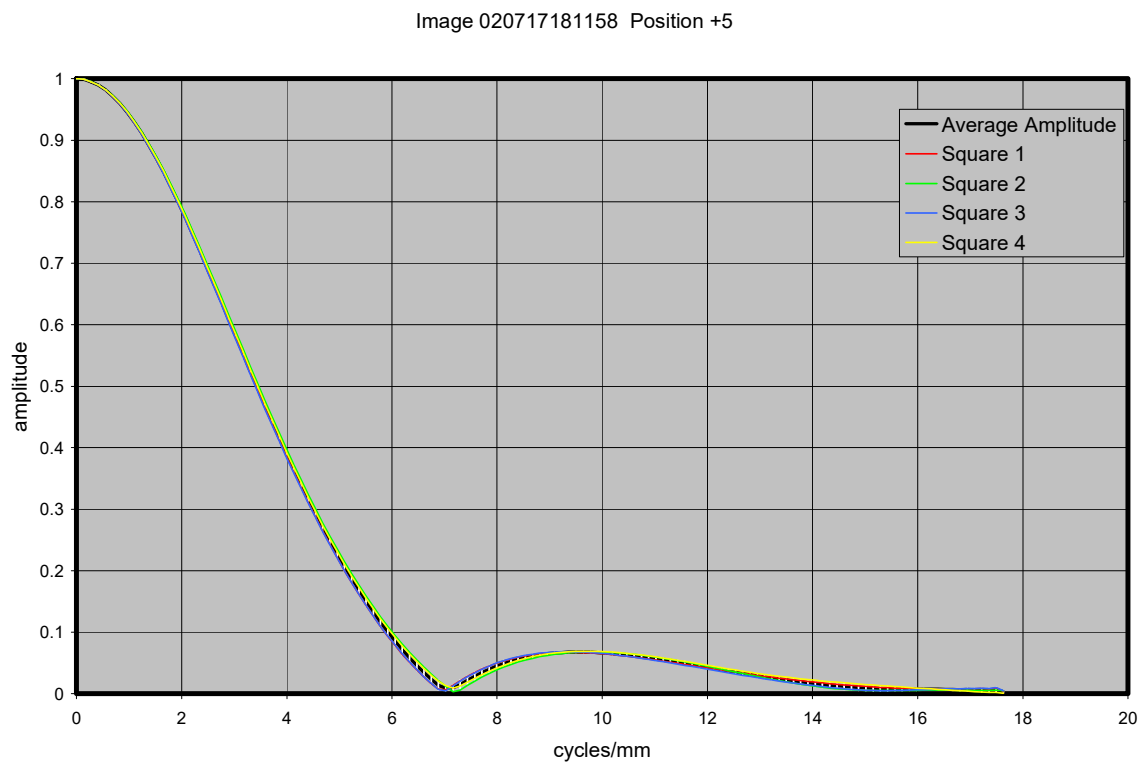
Figure 21.16. MTF curves for image with MI 105 CCD 95 mm from target
