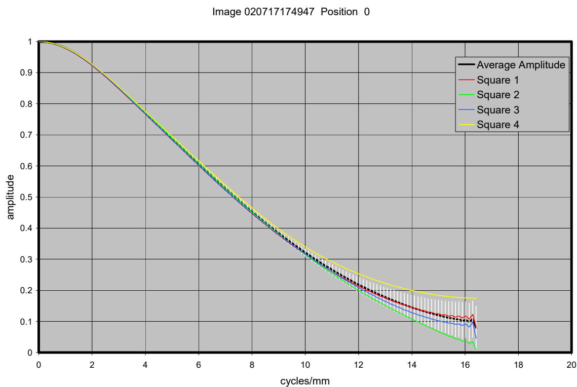
Figure 21.11. MTF curves for image with MI 105 CCD 100 mm from target
