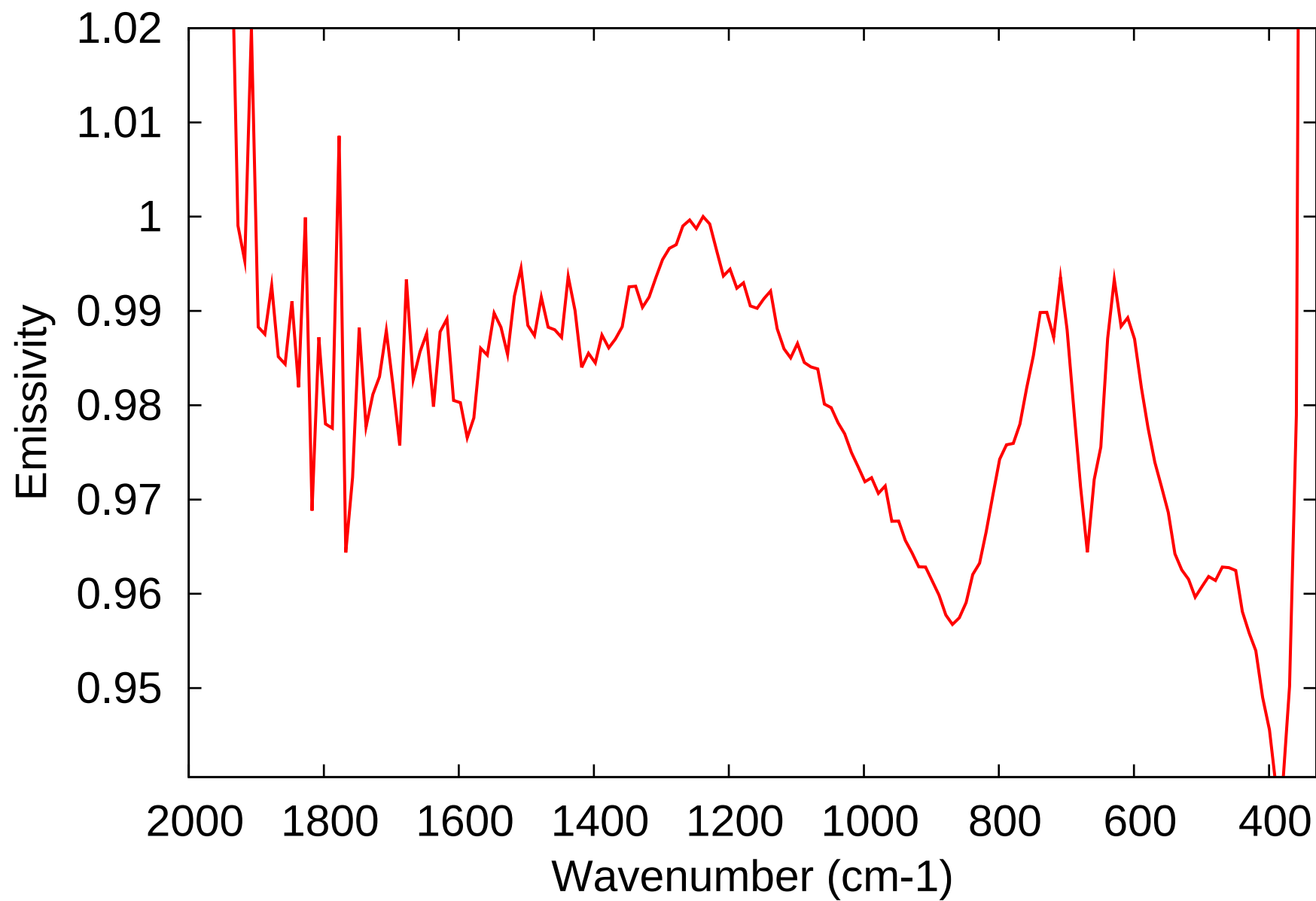
Mirror-dust-corrected Emissivity
