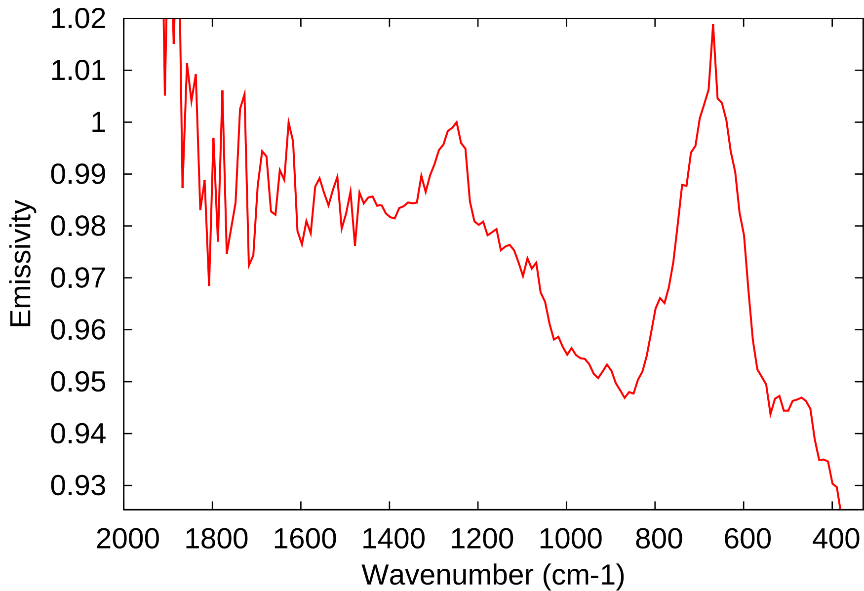
Mirror-dust-corrected Emissivity
