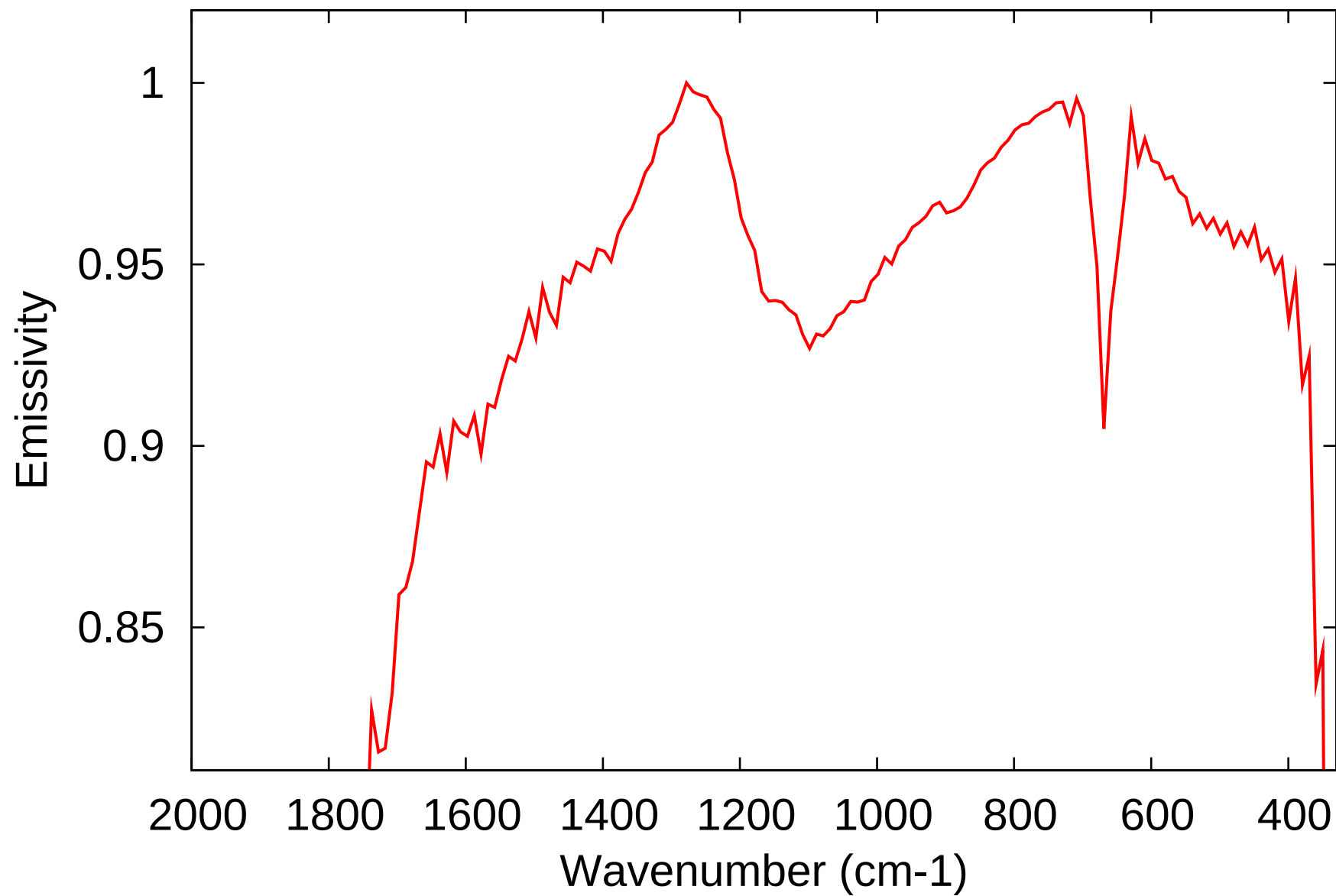
Mirror-dust-corrected Emissivity
