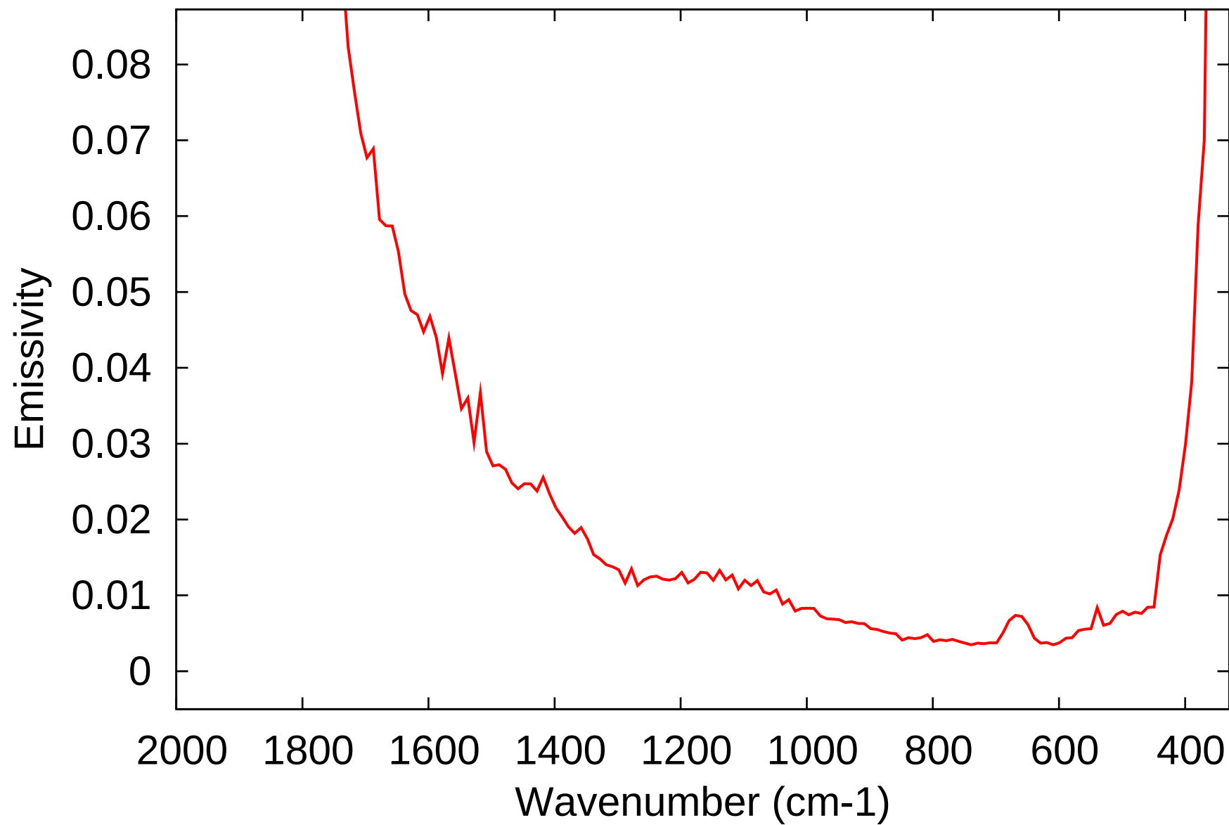
Mirror-dust-corrected Emissivity Standard Deviation
