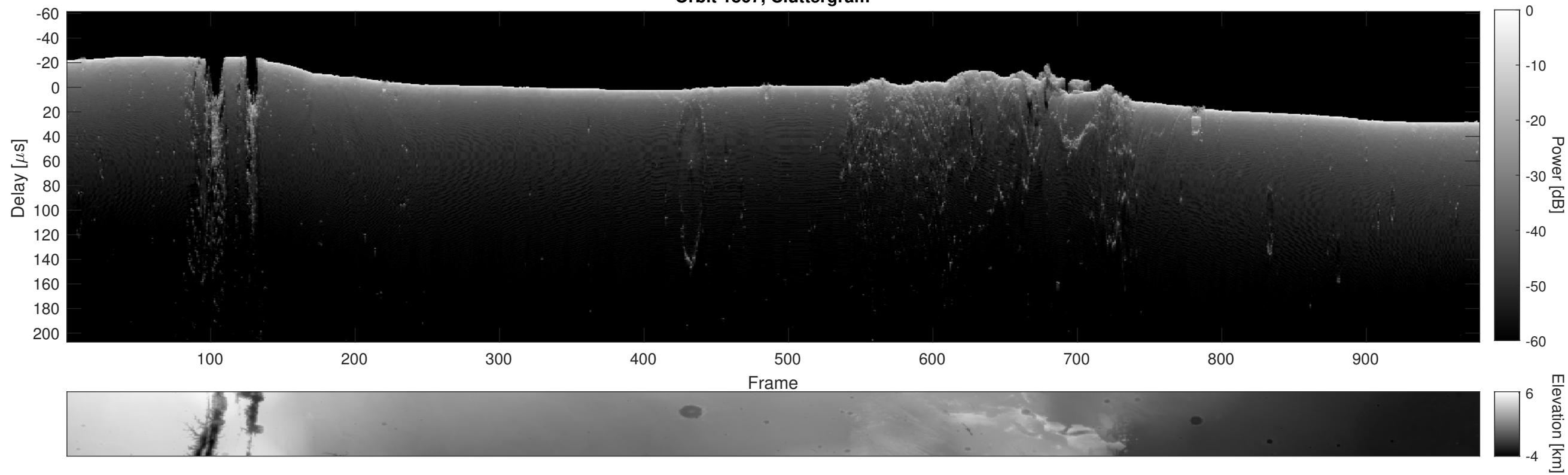
Orbit 1867, Cluttergram
