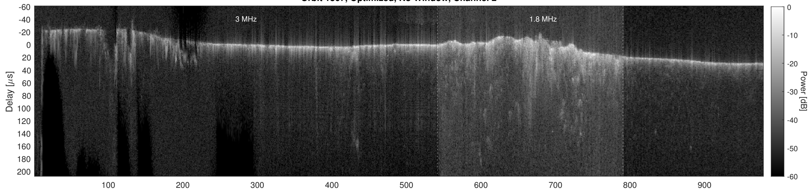
Orbit 1867, Cluttergram
