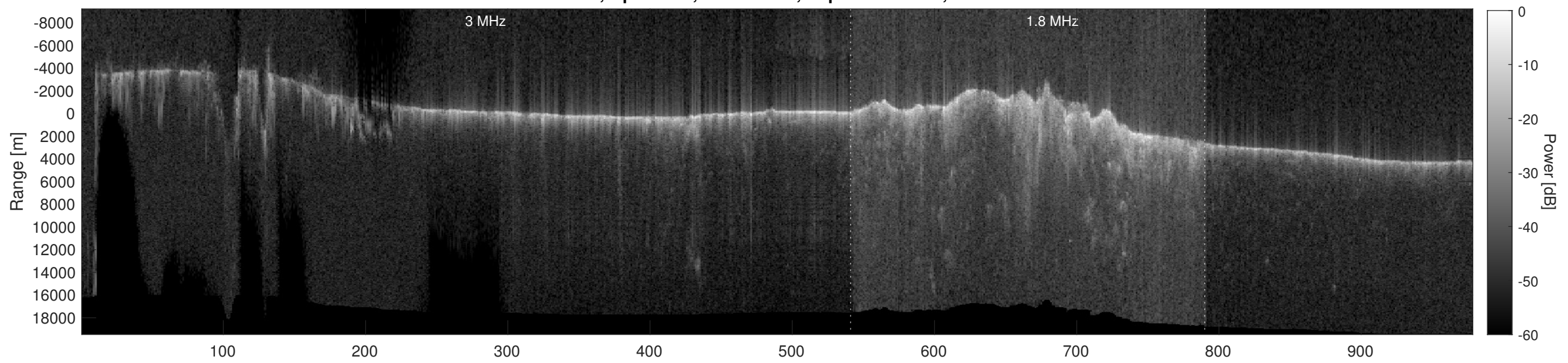
Orbit 1867, Depth-Corrected Cluttergram
