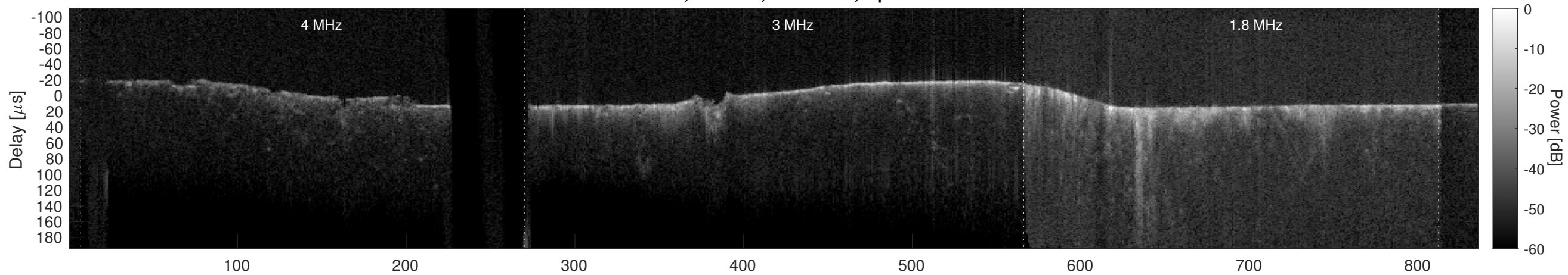
Orbit 1883, Cluttergram
