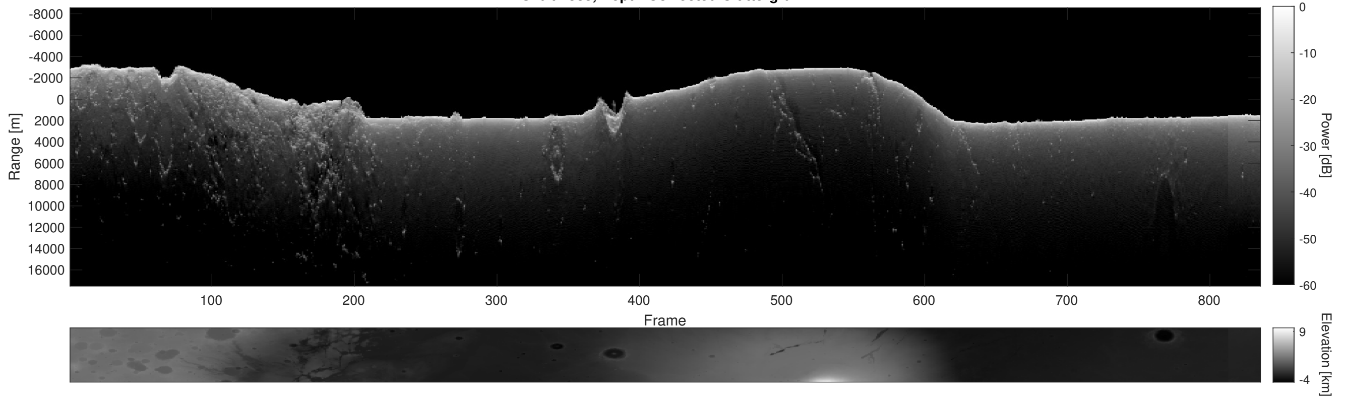
Orbit 1883, Depth-Corrected Cluttergram
