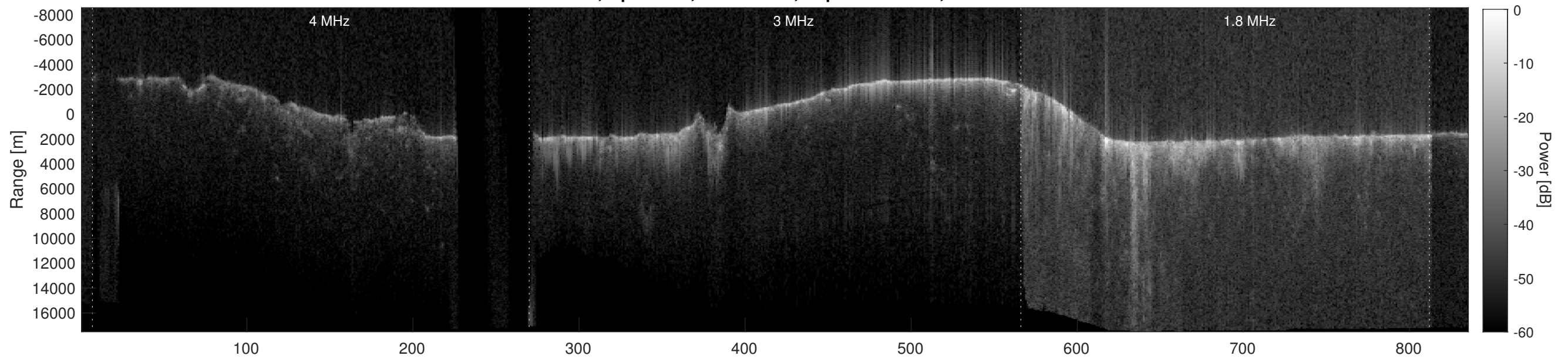
Orbit 1883, Depth-Corrected Cluttergram
