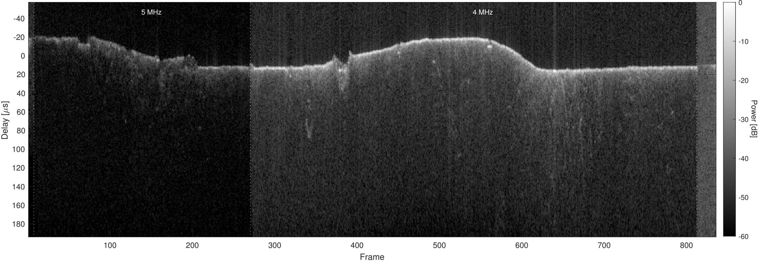
Orbit 1883, Optimized, Window, Channel 2
