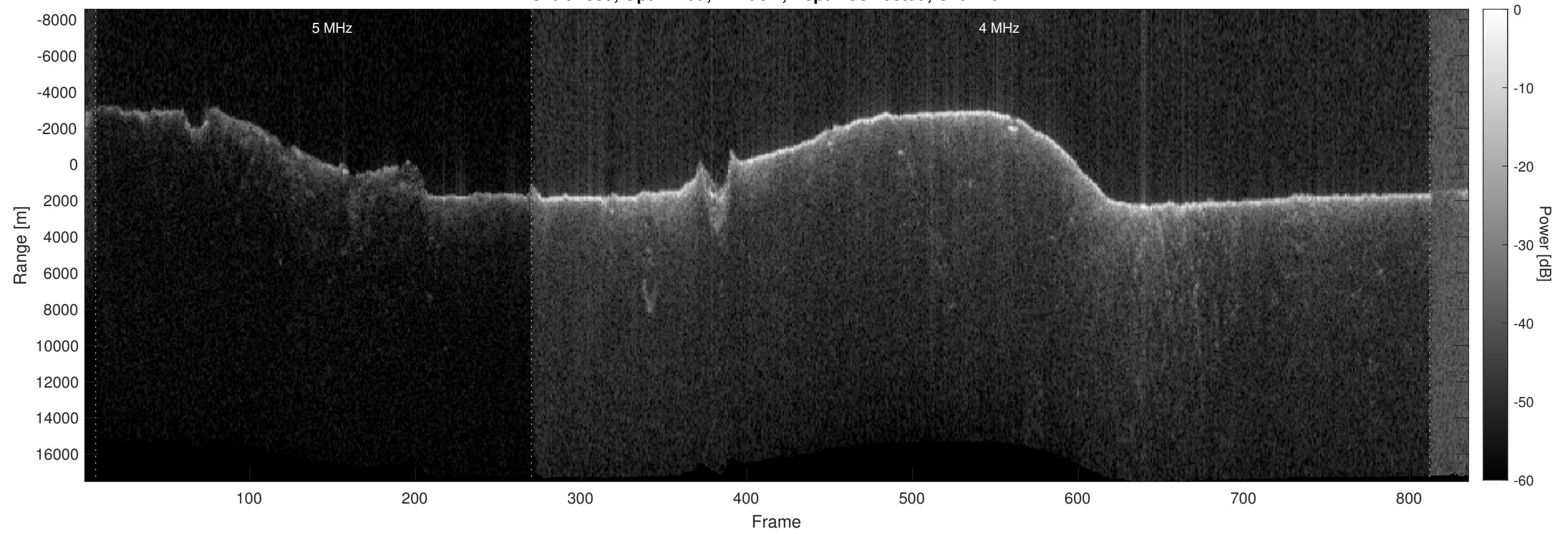
Orbit 1883, Optimized, Window, Depth-Corrected, Channel 2
