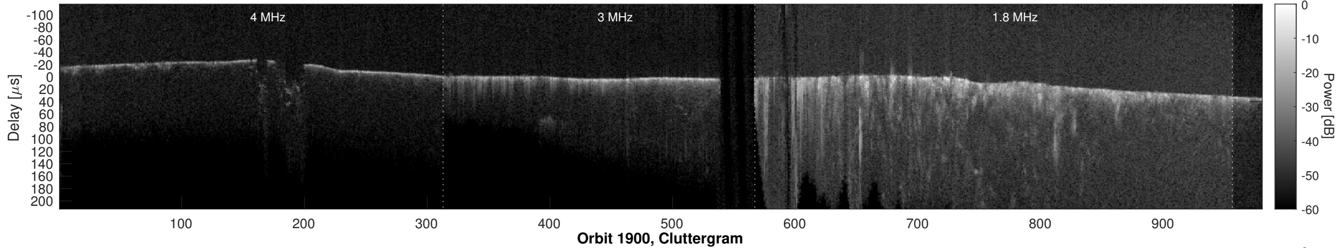
Orbit 1900, Window, Channel 2, Optimized
