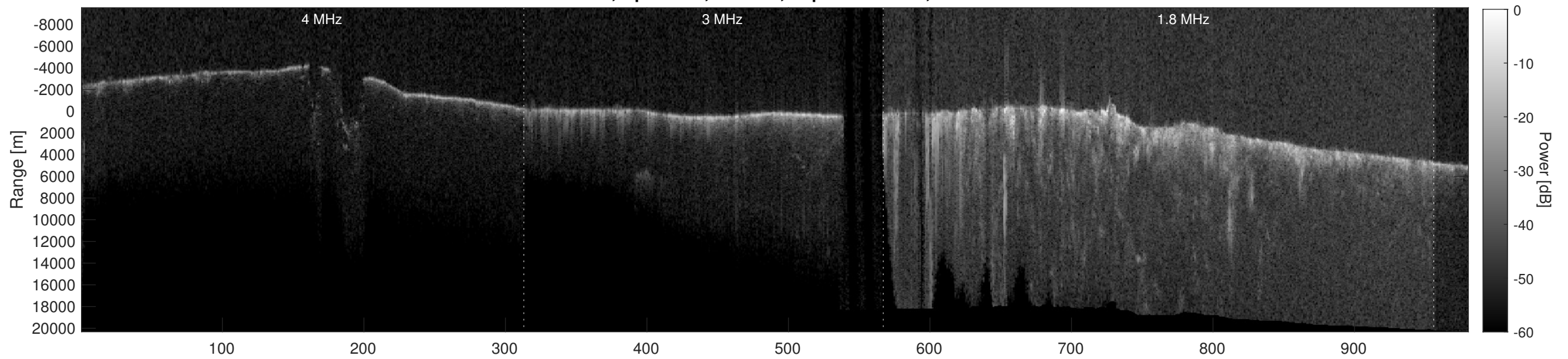
Orbit 1900, Depth-Corrected Cluttergram
