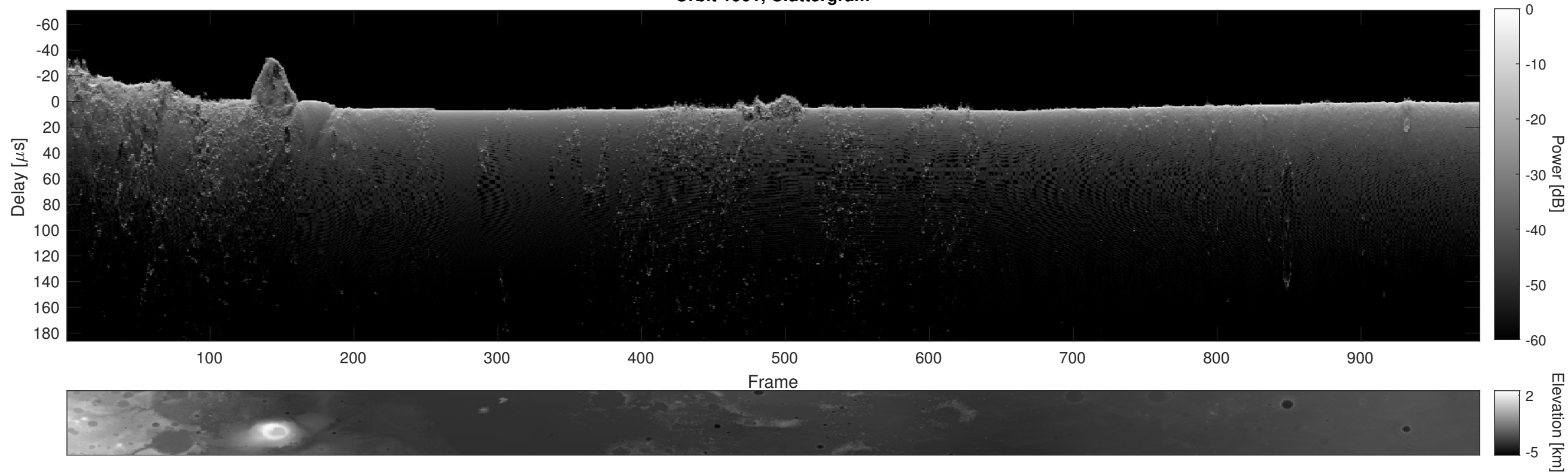
Orbit 1901, Cluttergram
