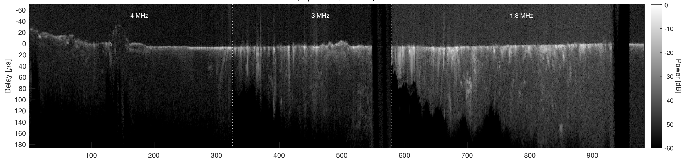
Orbit 1901, Cluttergram
