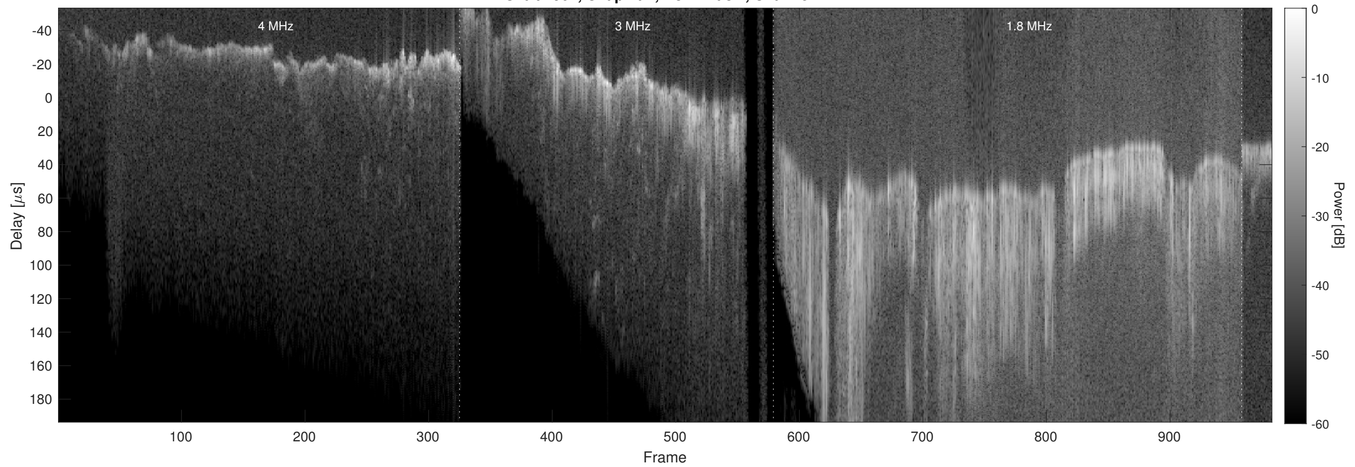
Orbit 1902, Chapman, No Window, Channel 2
