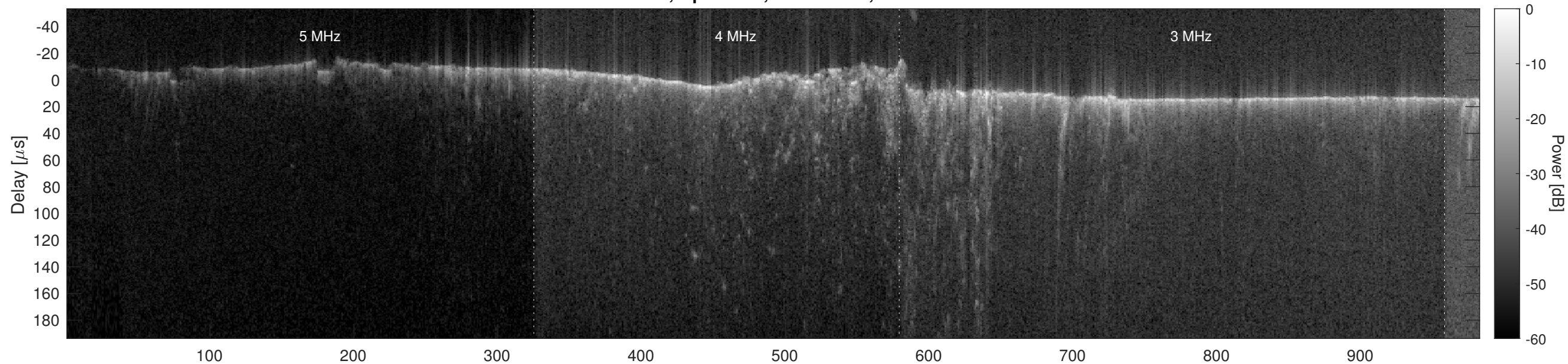
Orbit 1902, Optimized, No Window, Channel 2
