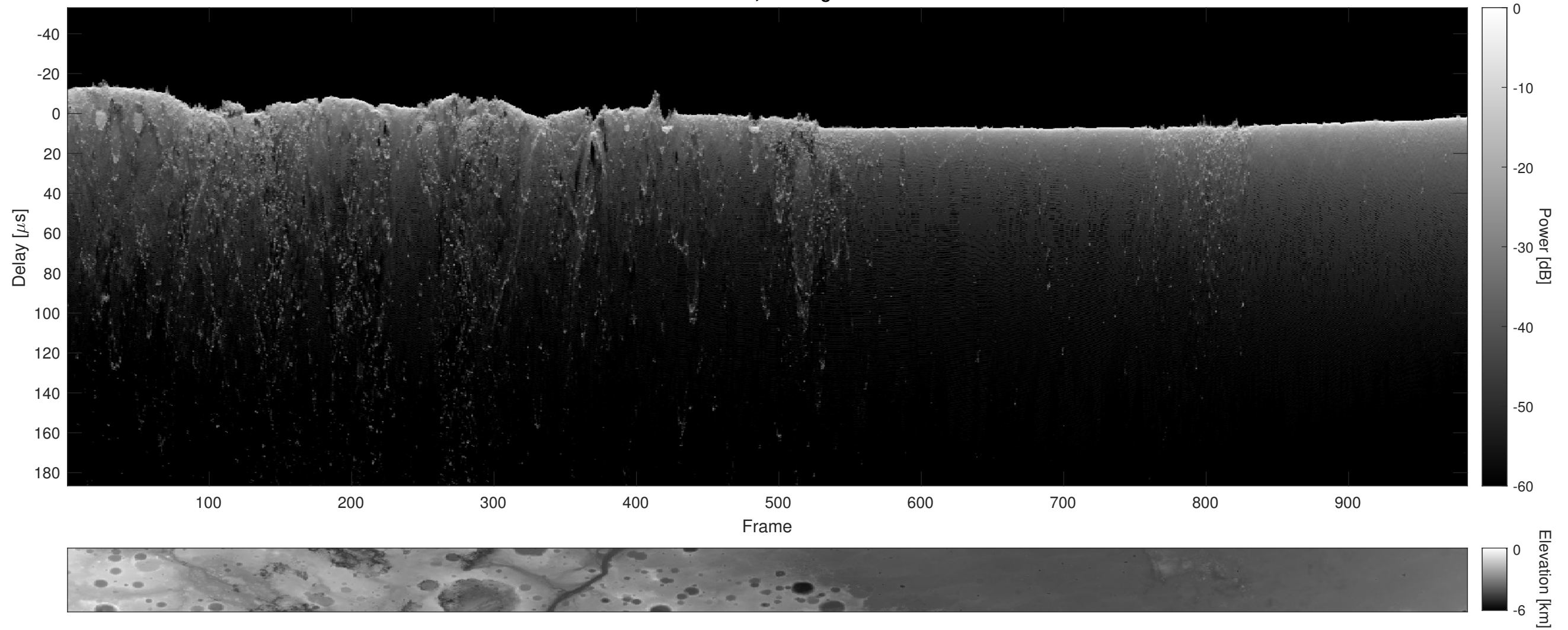
Orbit 1903, Cluttergram
