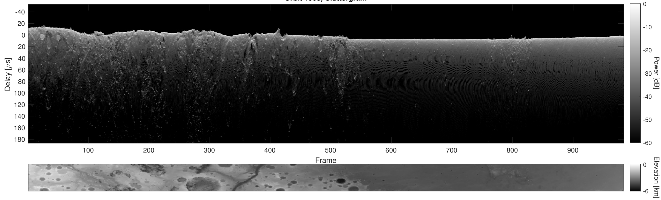
Orbit 1903, Cluttergram
