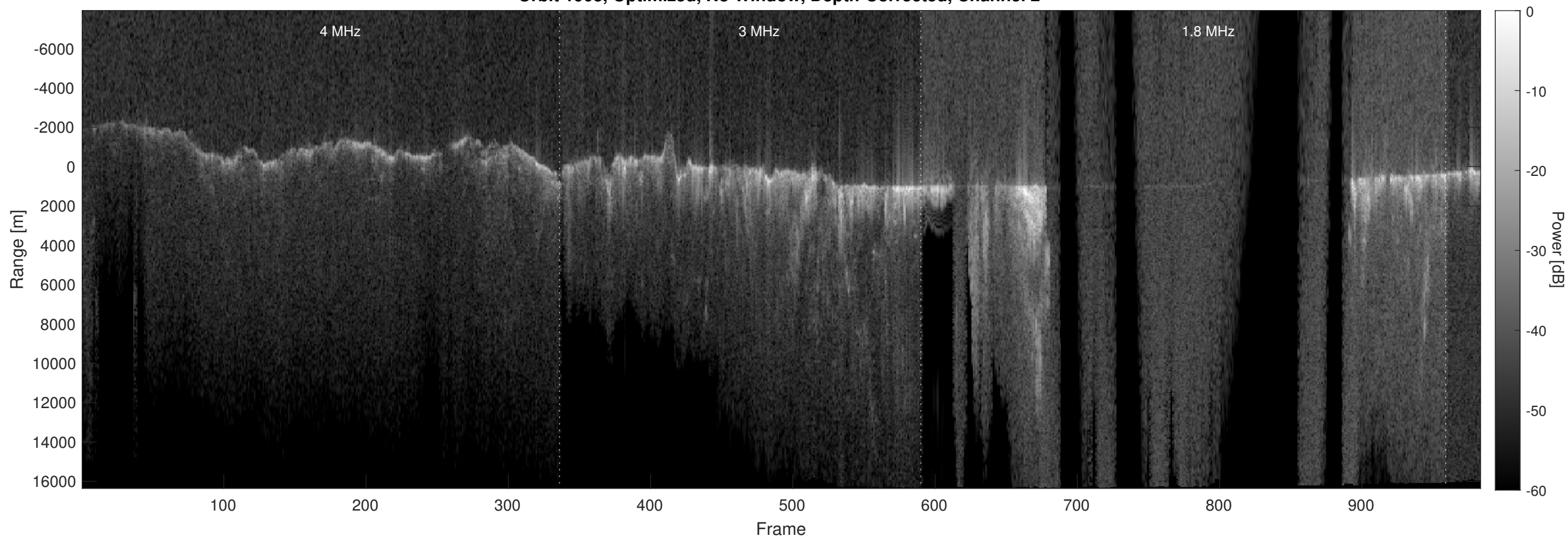
Orbit 1903, Optimized, No Window, Depth-Corrected, Channel 2
