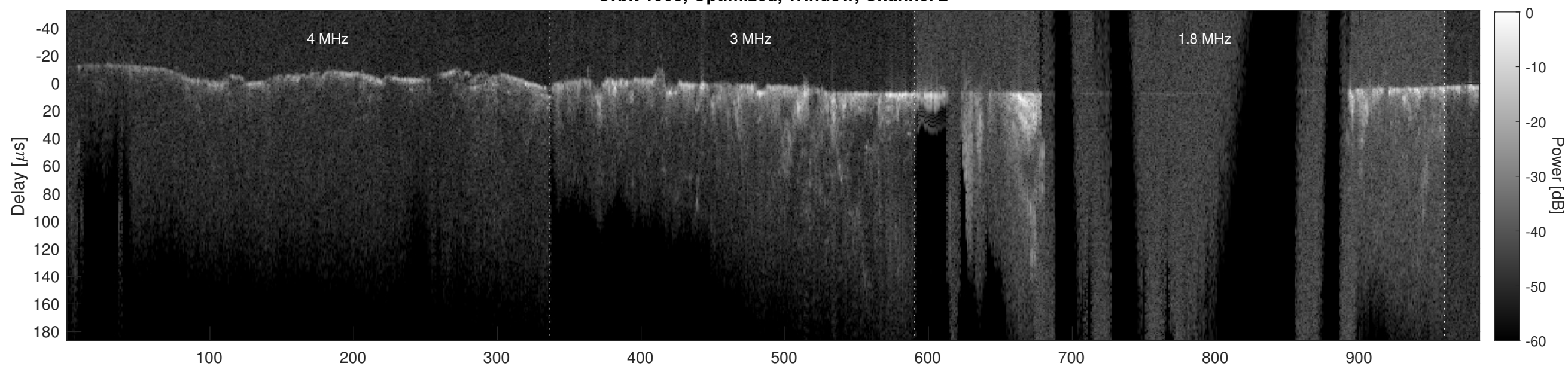
Orbit 1903, Cluttergram
