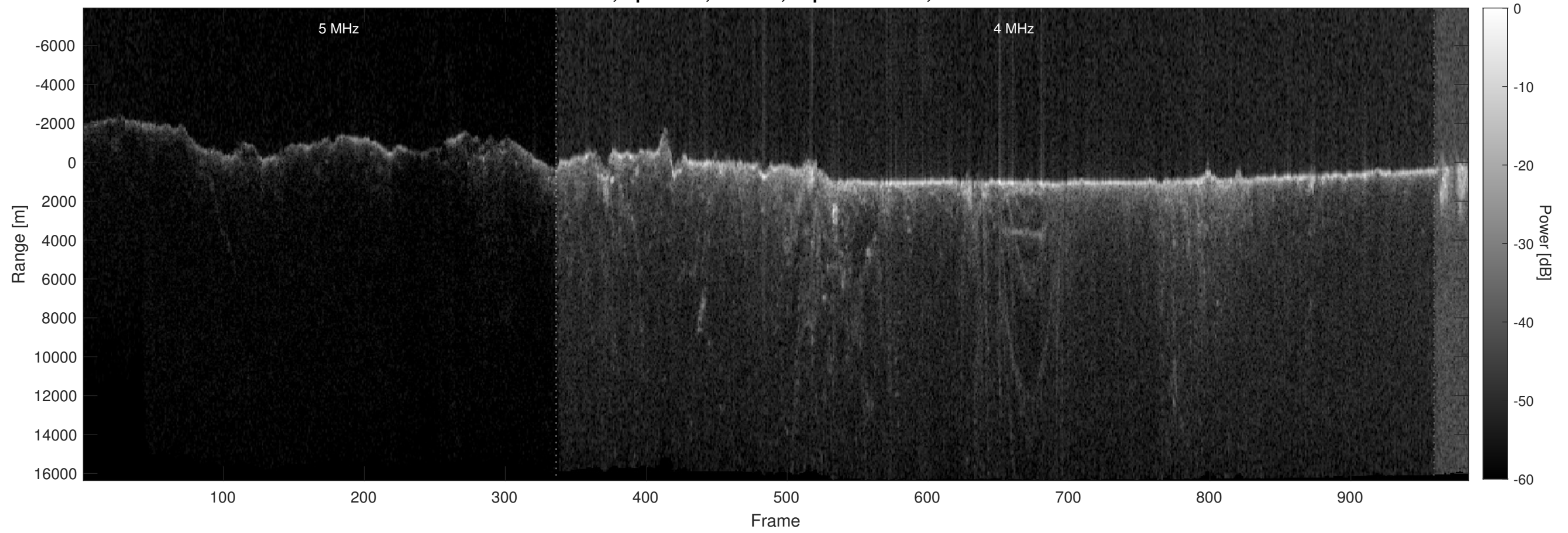
Orbit 1903, Optimized, Window, Depth-Corrected, Channel 2
