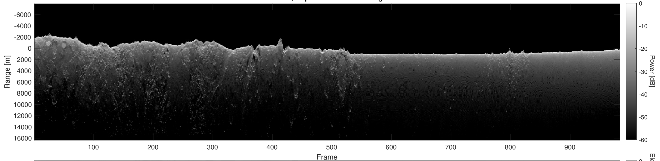
Orbit 1903, Depth-Corrected Cluttergram
