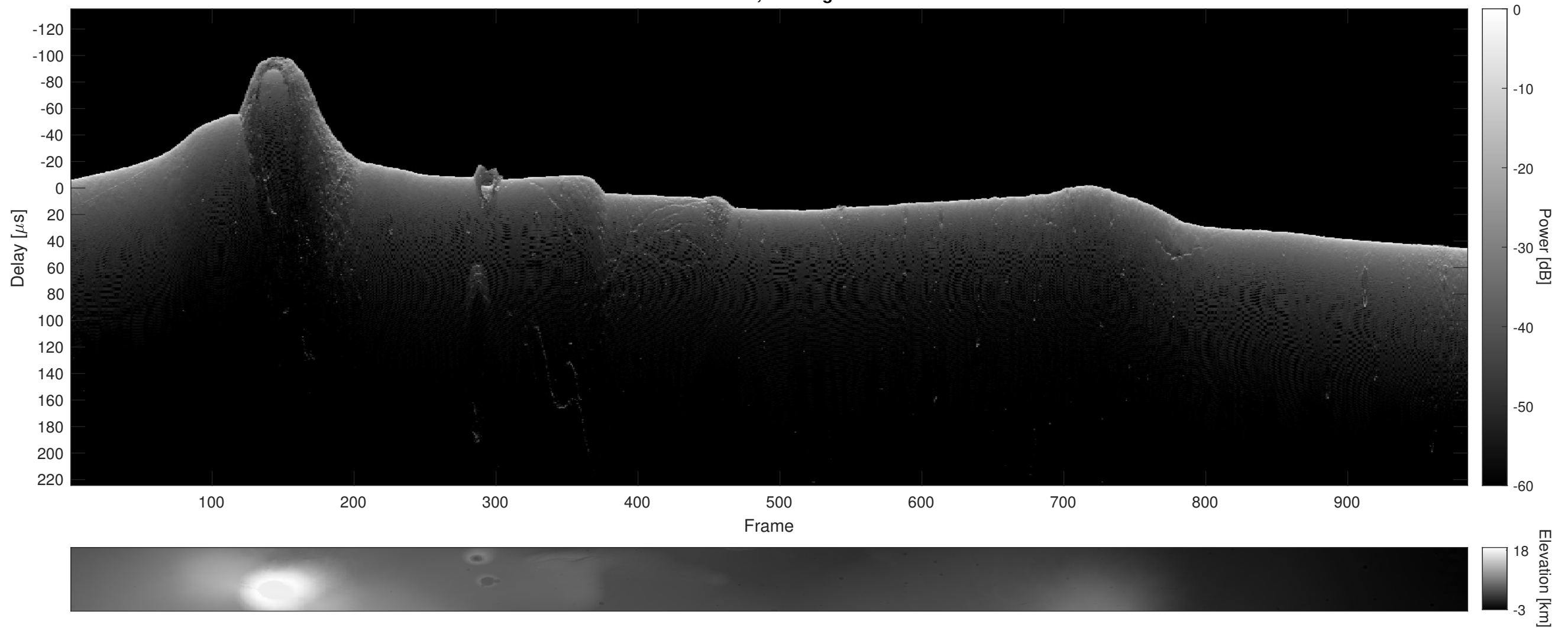
Orbit 1904, Cluttergram
