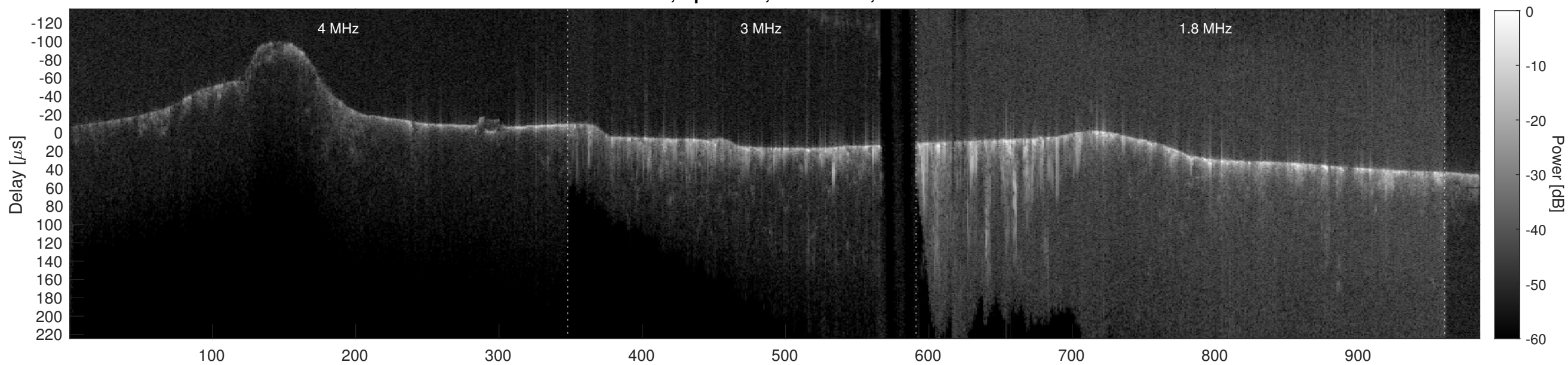
Orbit 1904, Cluttergram
