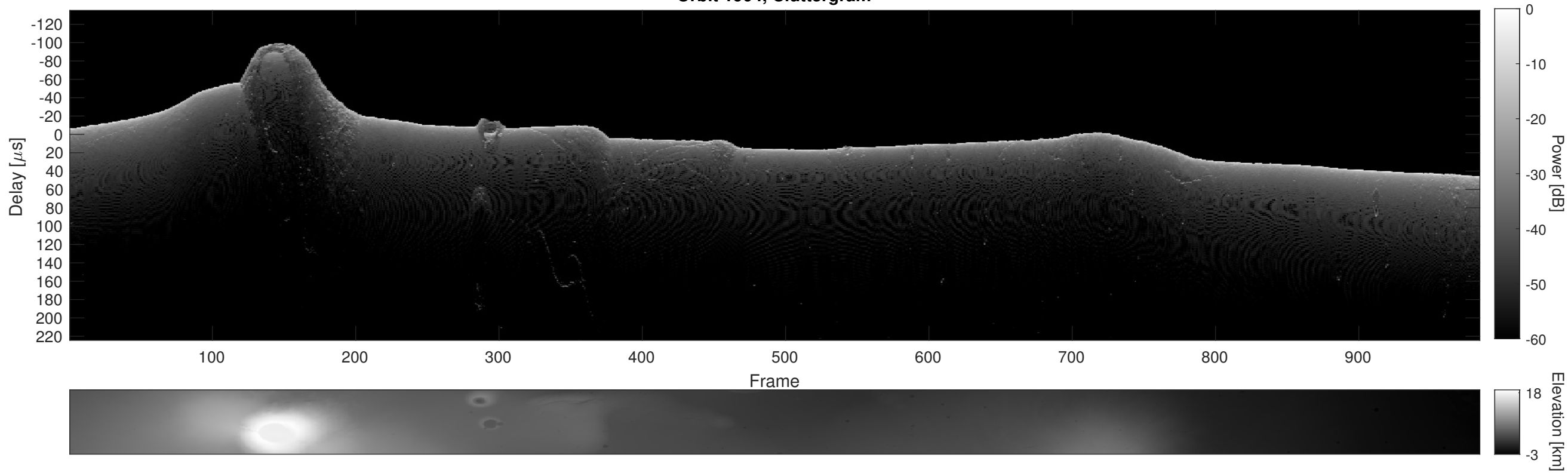
Orbit 1904, Cluttergram
