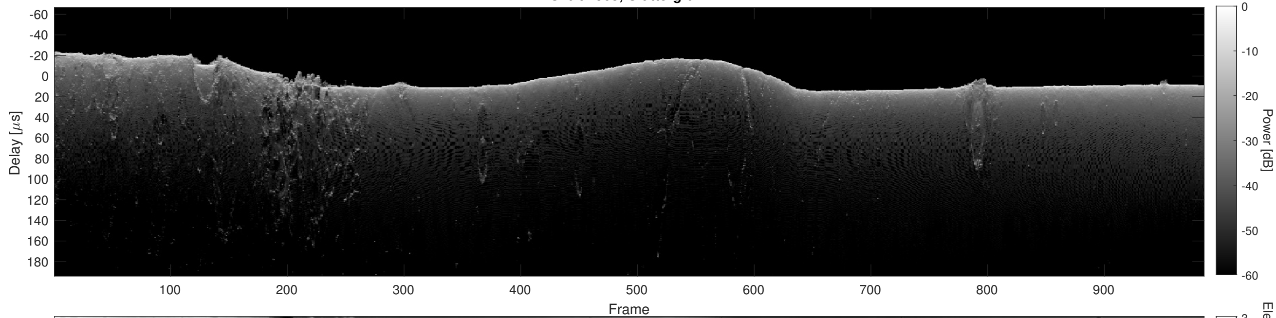
Orbit 1905, Cluttergram
