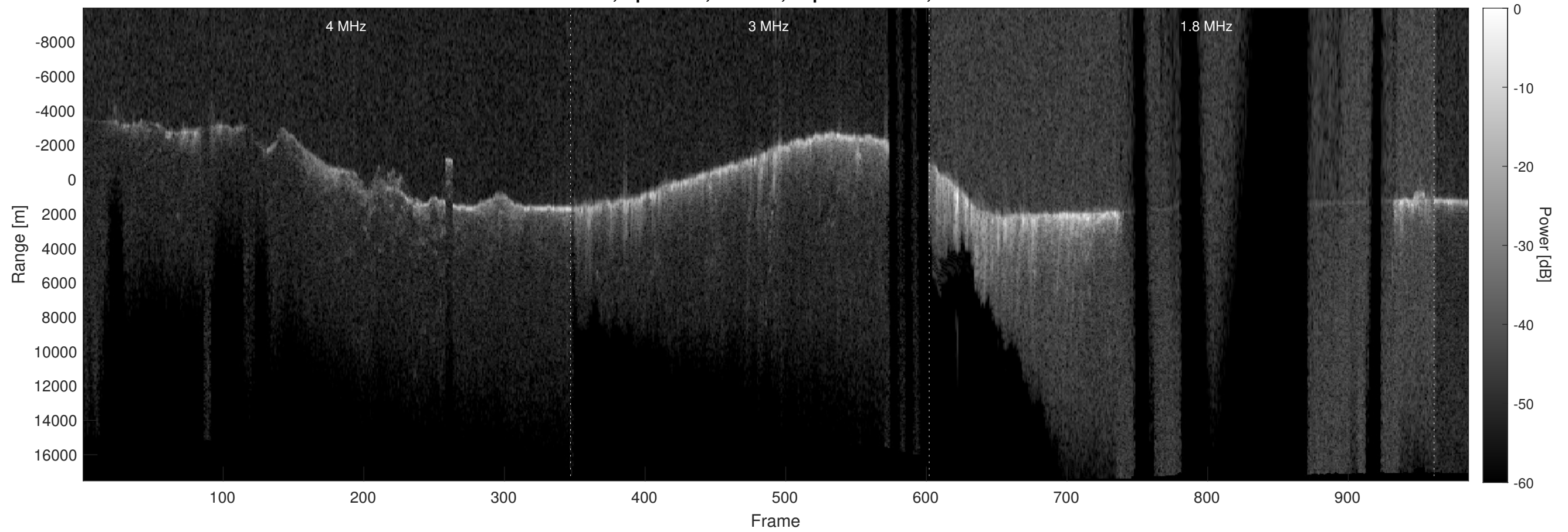
Orbit 1905, Optimized, Window, Depth-Corrected, Channel 2
