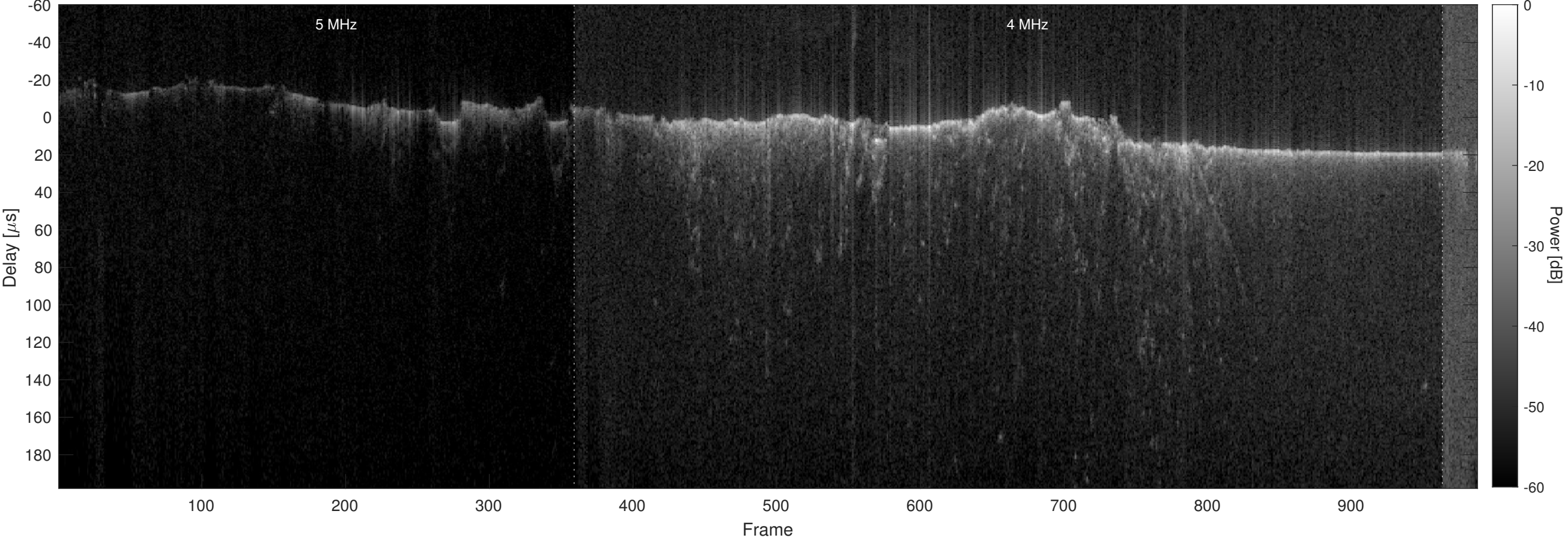
Orbit 1906, Optimized, No Window, Channel 2
