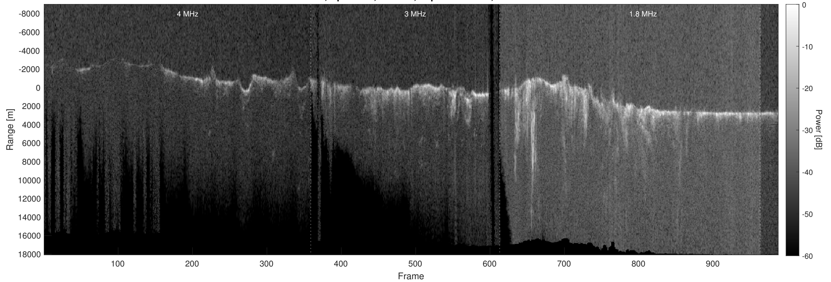
Orbit 1906, Optimized, Window, Depth-Corrected, Channel 2
