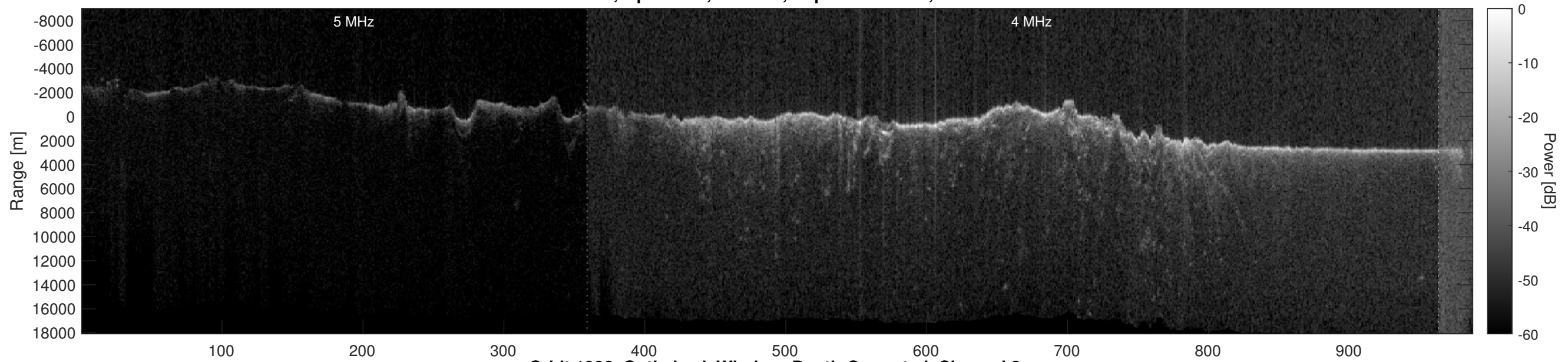
Orbit 1906, Optimized, Window, Depth-Corrected, Channel 2
