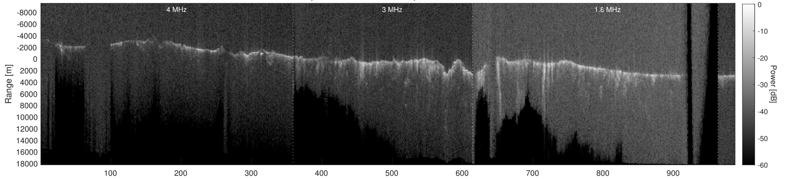
Orbit 1907, Depth-Corrected Cluttergram
