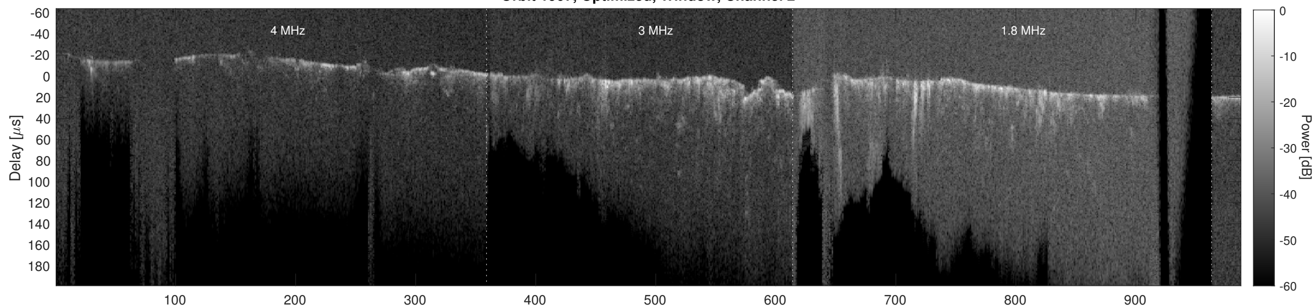
Orbit 1907, Cluttergram
