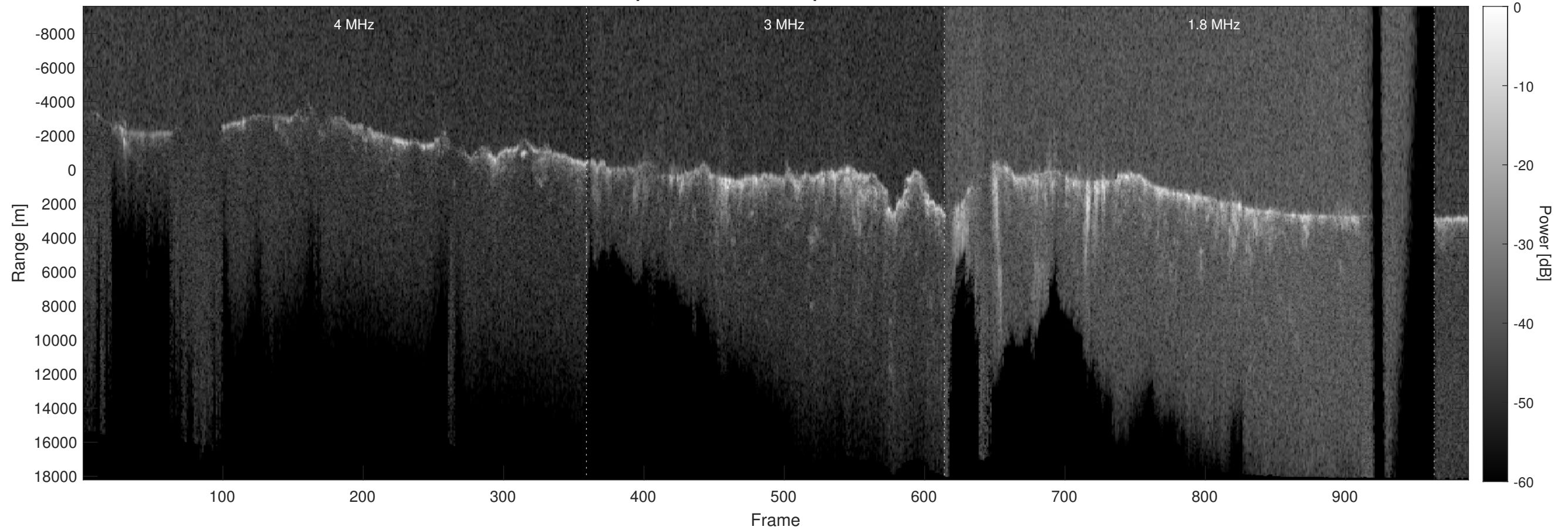
Orbit 1907, Optimized, Window, Depth-Corrected, Channel 2
