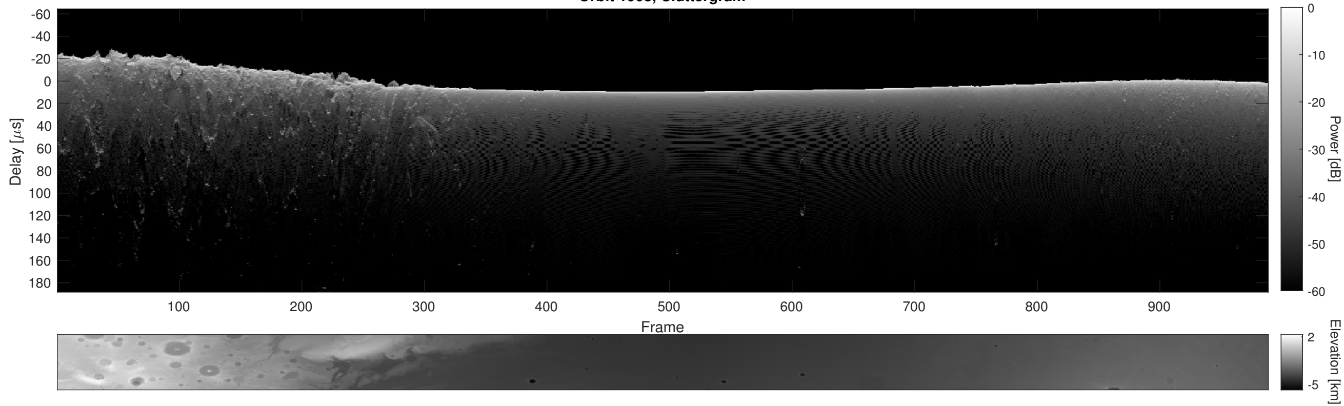
Orbit 1908, Cluttergram
