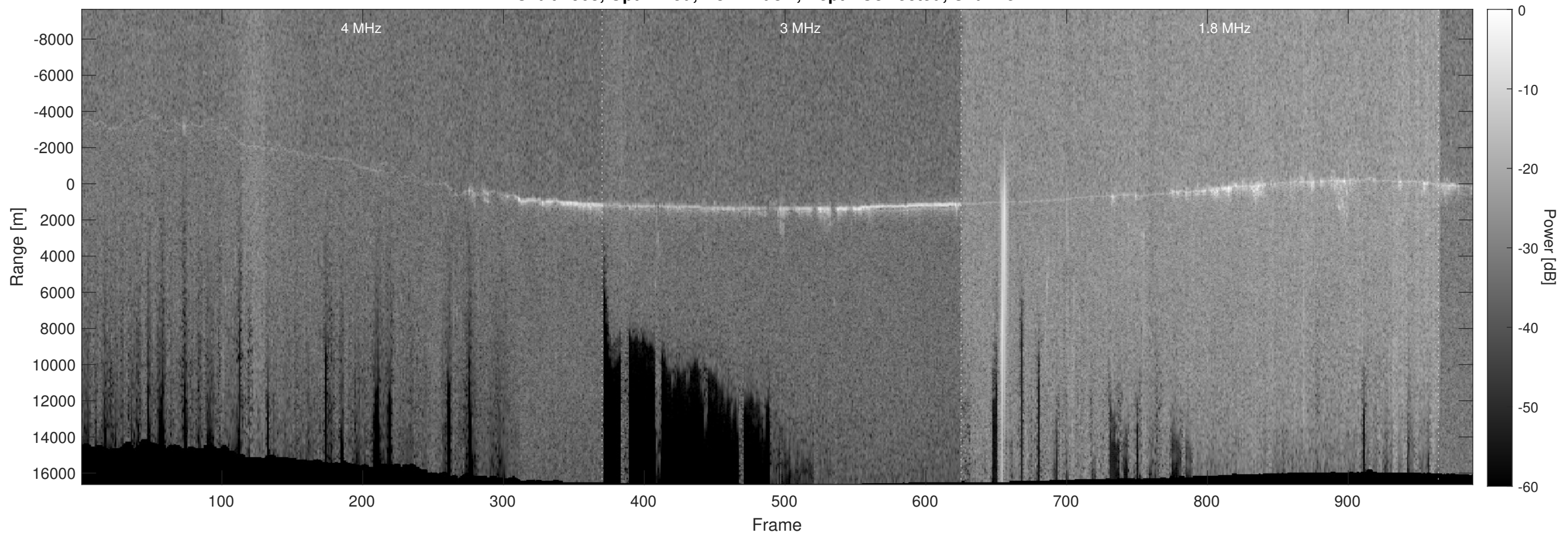
Orbit 1908, Optimized, No Window, Depth-Corrected, Channel 2
