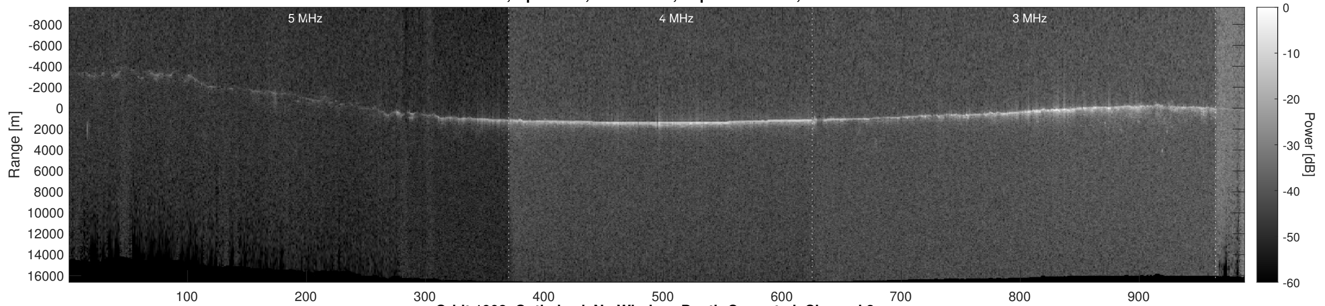
Orbit 1908, Optimized, No Window, Depth-Corrected, Channel 2
