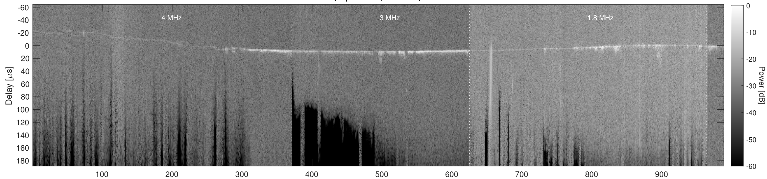
Orbit 1908, Cluttergram
