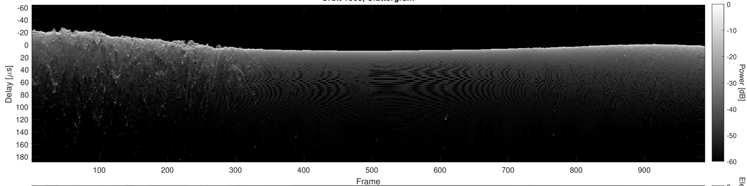
Orbit 1908, Cluttergram
