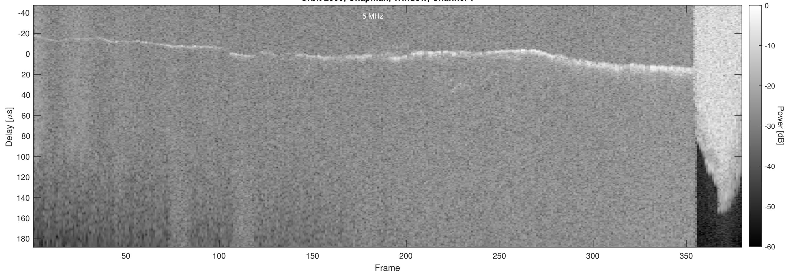
Orbit 2000, Chapman, Window, Channel 2
