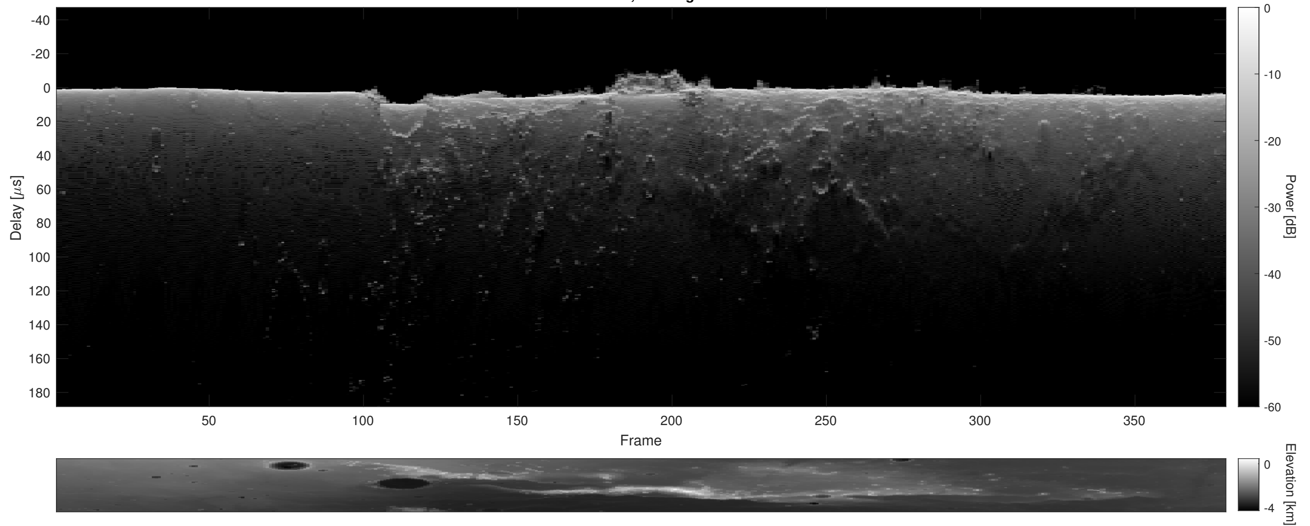
Orbit 2000, Cluttergram
