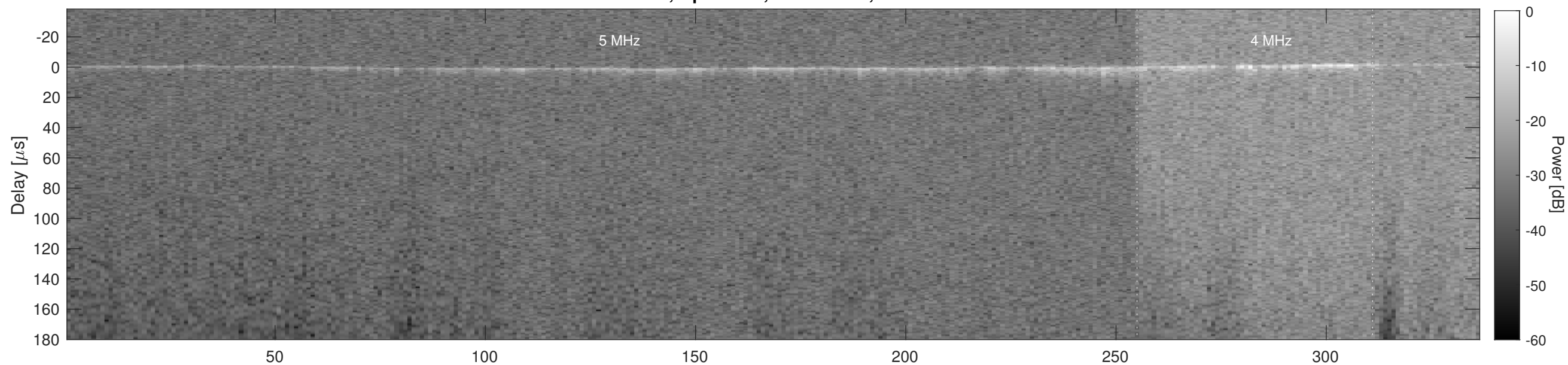
Orbit 2008, Cluttergram
